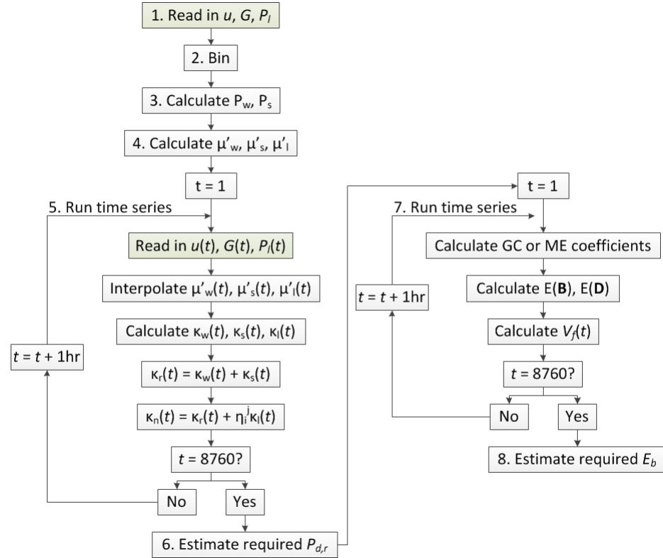
Figure 4.5: Fundamental algorithm for time series/probabilistic model
