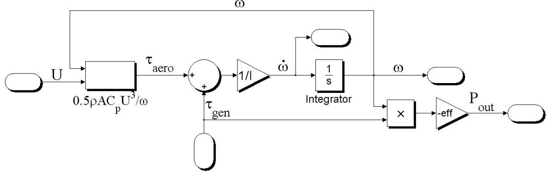
Figure 2.9: Plant block diagram
