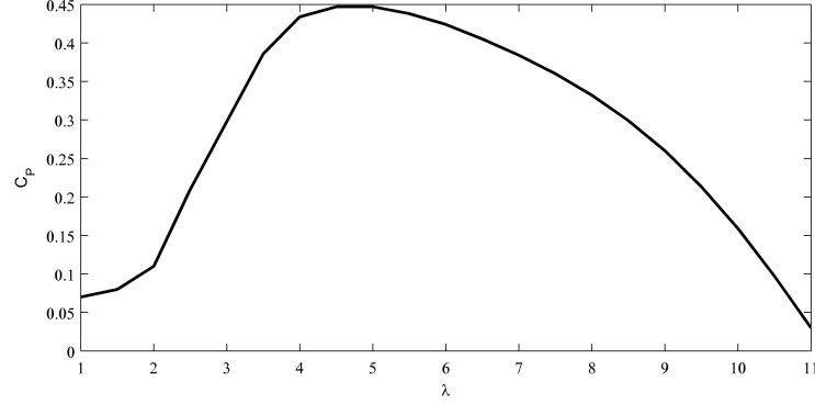
Figure 3.3: C_p - \lambda curve
