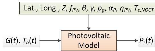
Figure 2.10: Solar sub-model
