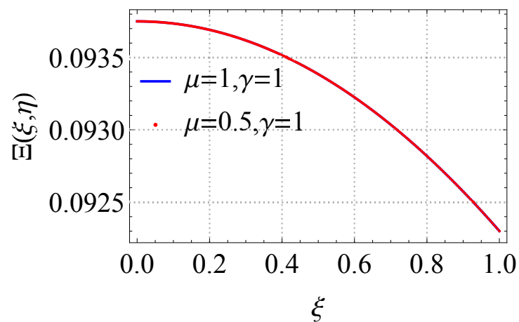
Figure 5. Graph of the solution of Model 3, with \alpha_2 = 2.7 , \alpha_1 = 0.7 , T = 1 , m = 5 and \tau = 0.00001 , and for different values of \mu and \gamma .
