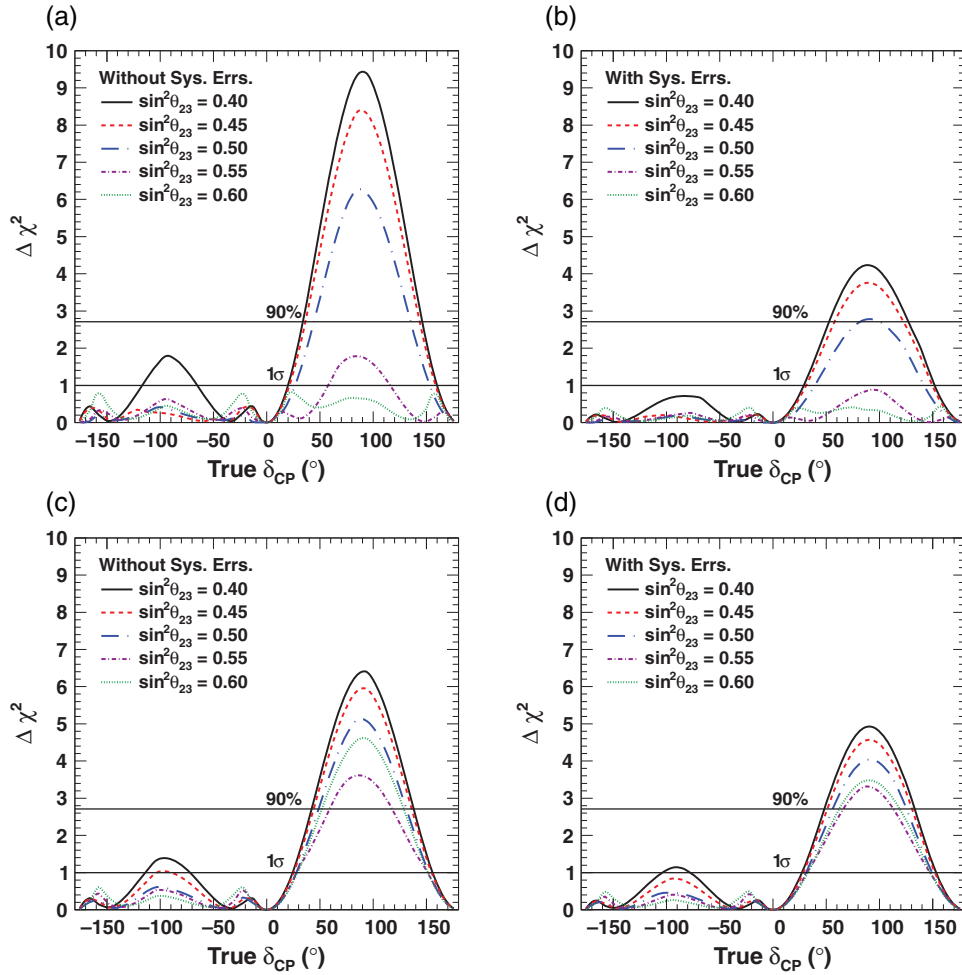
Fig. 9. The expected \Delta\chi^2 for the \sin\delta_{\text{CP}} = 0 hypothesis, plotted as a function of \delta_{\text{CP}} for various values of \sin^2\theta_{23} (given in the legend) in the case of inverted mass hierarchy. (a) 100% \nu -mode, statistical error only. (b) 100% \nu -mode, with the 2012 systematic errors. (c) 50% \nu , 50% \bar{\nu} -mode, statistical error only. (d) 50% \nu -, 50% \bar{\nu} -mode, with the 2012 systematic errors.
