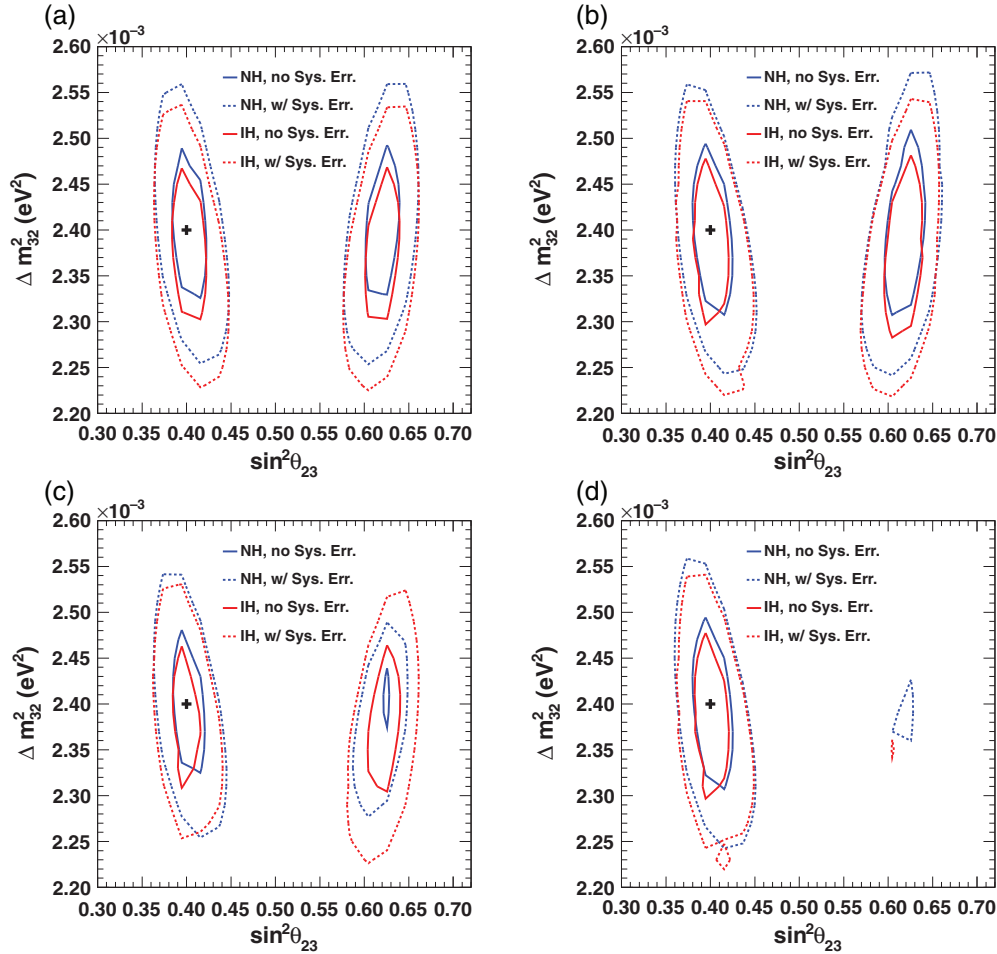
Fig. 6. \Delta m_{32}^2 vs. \sin^2 \theta_{23} 90% C.L. intervals for 7.8 \times 10^{21} POT. Contours are plotted for the case of true \delta_{\text{CP}} = 0^\circ , \sin^2 \theta_{23} = 0.4 , \Delta m_{32}^2 = 2.4 \times 10^{-3} \text{ eV}^2 and NH. The blue curves are fitted assuming the correct MH(NH), while the red are fitted assuming the incorrect MH(IH), and contours are plotted from the minimum \chi^2 value for both MH assumptions. The solid contours are with statistical error only, while the dashed contours include the 2012 systematic errors fully correlated between \nu - and \bar{\nu} -mode. (a) 100% \nu -mode. (b) 50% \nu -, 50% \bar{\nu} -mode. (c) 100% \nu -mode, with ultimate reactor error. (d) 50% \nu -, 50% \bar{\nu} -mode, with ultimate reactor error.
