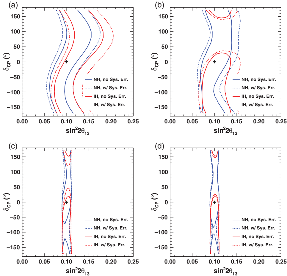
Fig. 4. \delta_{\text{CP}} vs. \sin^2 2\theta_{13} 90% C.L. intervals for 7.8 \times 10^{21} POT. Contours are plotted for the case of true \delta_{\text{CP}} = 0^\circ and NH. The blue curves are fitted assuming the correct MH(NH), while the red are fitted assuming the incorrect MH(IH), and contours are plotted from the minimum \chi^2 value for both MH assumptions. The solid contours are with statistical error only, while the dashed contours include the 2012 systematic errors fully correlated between \nu - and \bar{\nu} -mode. (a) 100% \nu -mode. (b) 50% \nu -, 50% \bar{\nu} -mode. (c) 100% \nu -mode, with ultimate reactor constraint. (d) 50% \nu -, 50% \bar{\nu} -mode, with ultimate reactor constraint.
