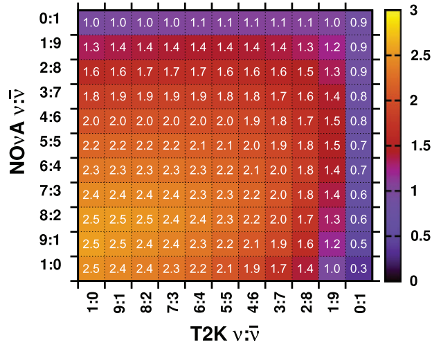
Fig. 22. Lowest \Delta\chi^2 for a combined T2K + NOνA fit to determine the mass hierarchy for various \nu:\bar{\nu} running ratios. True values are assumed to be: MH=NH, \sin^2(\theta_{23}) = 0.5 . Normalization systematics are assumed.
