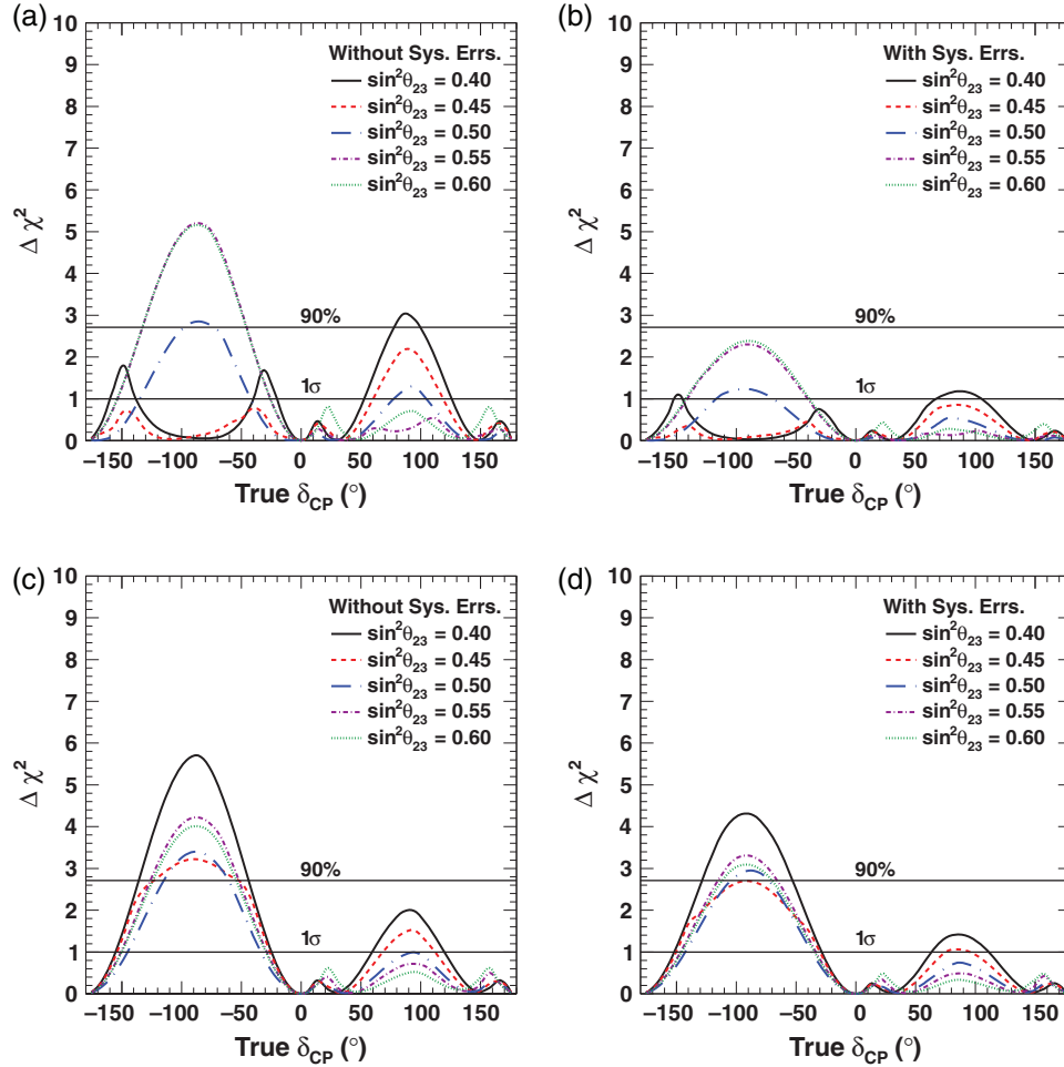
Fig. 8. The expected \Delta\chi^2 for the \sin\delta_{CP} = 0 hypothesis, plotted as a function of \delta_{CP} for various values of \sin^2\theta_{23} (given in the legend) in the case of normal mass hierarchy. (a) 100% \nu -mode, statistical error only. (b) 100% \nu -mode, with the 2012 systematic errors. (c) 50% \nu , 50% \bar{\nu} -mode, statistical error only. (d) 50% \nu , 50% \bar{\nu} -mode, with the 2012 systematic errors.
