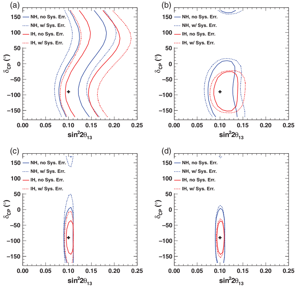
Fig. 5. \delta_{\text{CP}} vs. \sin^2 2\theta_{13} 90% C.L. intervals for 7.8 \times 10^{21} POT. Contours are plotted for the case of true \delta_{\text{CP}} = -90^\circ and NH. The blue curves are fitted assuming the correct MH(NH), while the red are fitted assuming the incorrect MH(IH), and contours are plotted from the minimum \chi^2 value for both MH assumptions. The solid contours are with statistical error only, while the dashed contours include the 2012 systematic errors fully correlated between \nu - and \bar{\nu} -mode. (a) 100% \nu -mode. (b) 50% \nu -, 50% \bar{\nu} -mode. (c) 100% \nu -mode, with ultimate reactor constraint. (d) 50% \nu -, 50% \bar{\nu} -mode, with ultimate reactor constraint.
