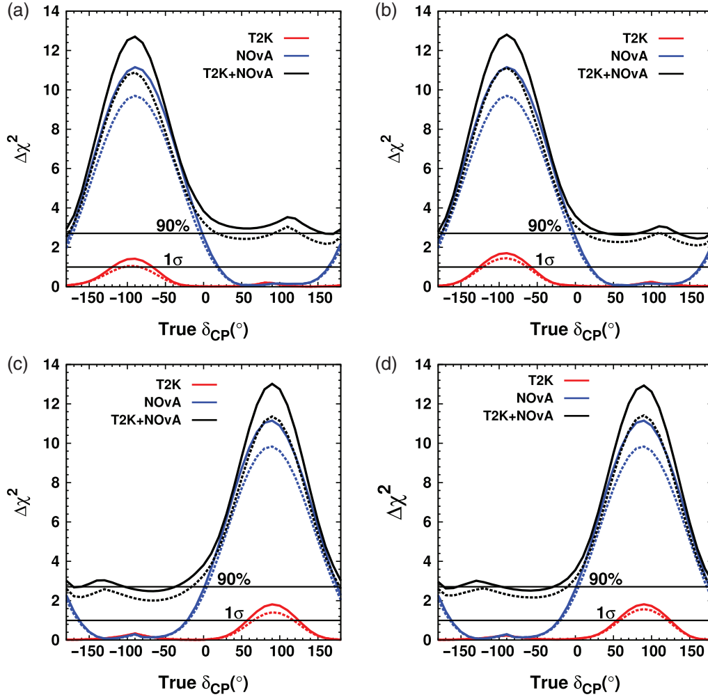
Fig. 21. The predicted \Delta\chi^2 for rejecting the incorrect MH hypothesis, as a function of \delta_{\text{CP}} for T2K (red), \text{NO}\nu\text{A} (blue), and T2K + \text{NO}\nu\text{A} (black). Dashed (solid) curves indicate studies where normalization systematics are (not) considered. The “true” value of \sin^2(\theta_{23}) is assumed to be 0.5, and the “true” MH is assumed to be the NH (top) or the IH (bottom). The “test” MH is unconstrained. (a) 1:0 T2K, 1:1 \text{NO}\nu\text{A} \nu:\bar{\nu} , NH. (b) 1:1 T2K, 1:1 \text{NO}\nu\text{A} \nu:\bar{\nu} , NH. (c) 1:0 T2K, 1:1 \text{NO}\nu\text{A} \nu:\bar{\nu} , IH. (d) 1:1 T2K, 1:1 \text{NO}\nu\text{A} \nu:\bar{\nu} , IH.
