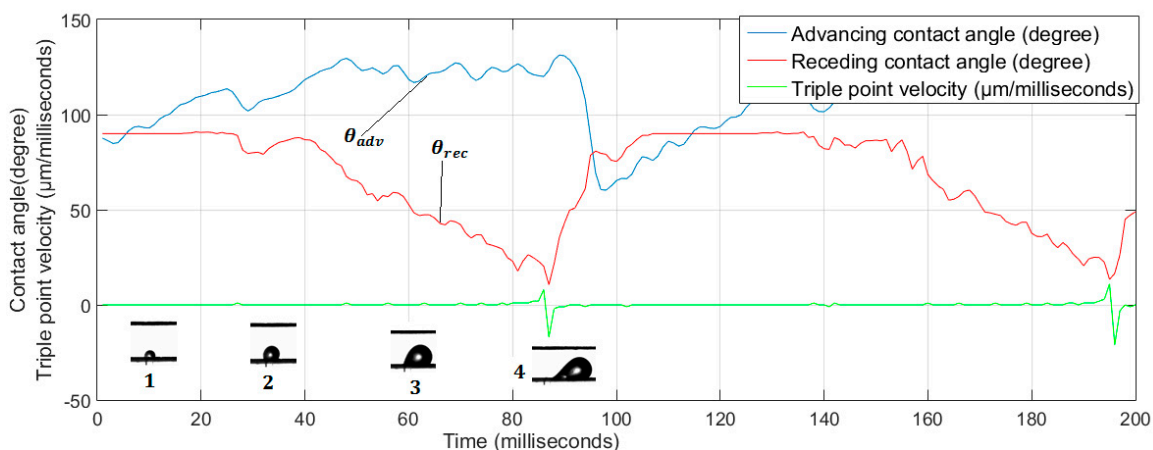
Figure 21. Water droplet images and corresponding evolution of \theta_{adv} , \theta_{rcd} , and TPV: (1) at droplet emergence, (2) droplet growth, (3) onset of droplet deformation, (4) detachment.
