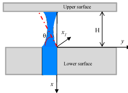
Figure 5. Schematic of a capillary bridge and geometric parameters.
