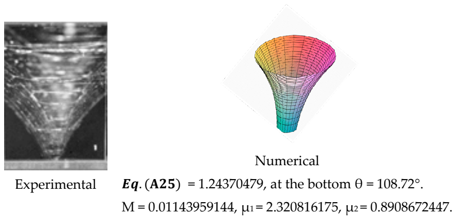
Figure 23. Comparison between experimental [74] and numerical unduloid surfaces.
