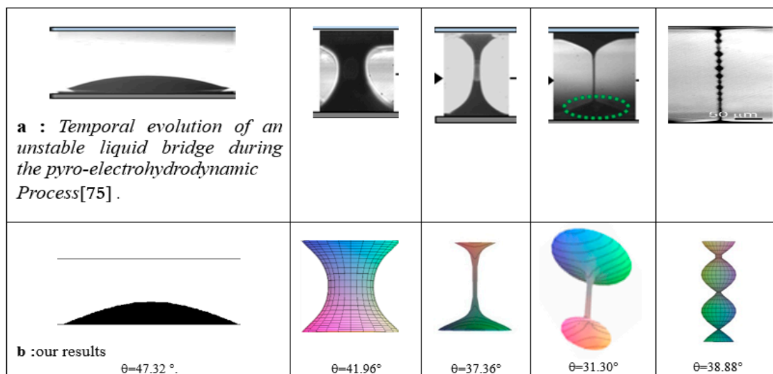
Figure 24. Comparison of model predictions to experiments reported by Grilli et al., 2011 [75].
