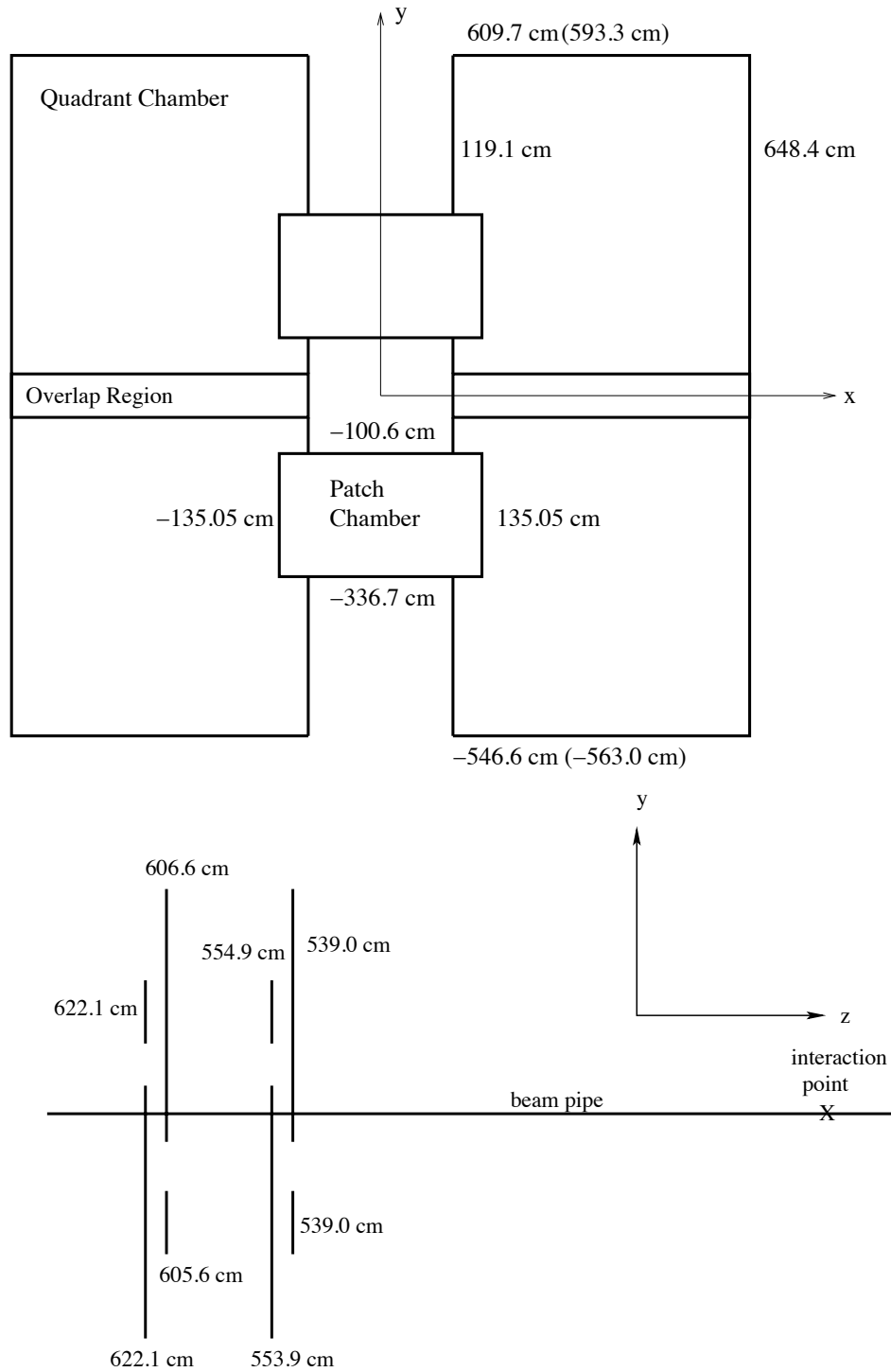
Figure A.2: The endcap regions of the muon chambers in the x - y (upper) and y - z (lower) planes. The quadrant chambers overlap vertically, but not horizontally.
