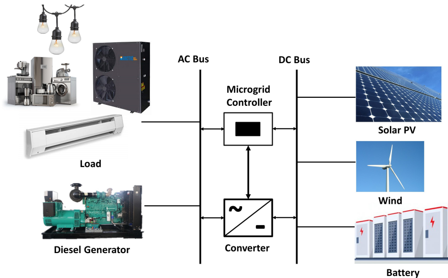
Figure 3.3: Schematic diagram of an integrated electrical and thermal energy system.
