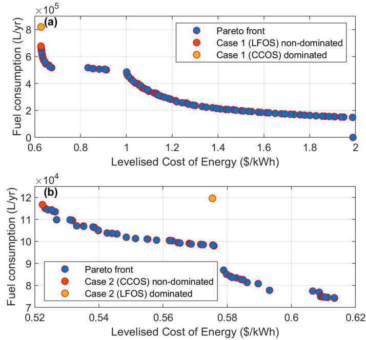
Figure 3.13: Changing the dispatch control would make the solution sub-optimal (dominated): (a) Case 1 Pareto front (under load following) with the combined electricity and thermal load profiles; (b) Case 2 Pareto front (under cycle charging) with electricity load profile only.
