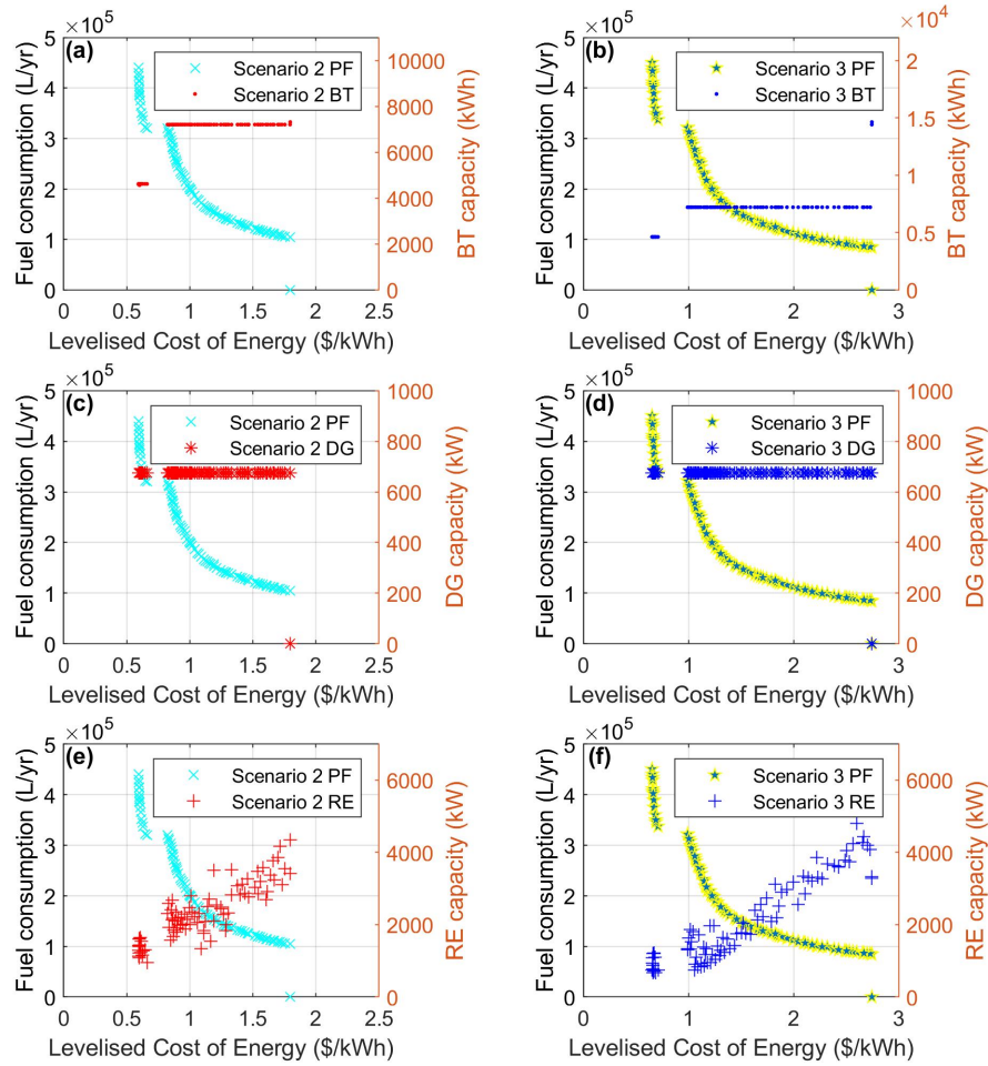
Figure 3.17: Comparison of subcomponents optimal capacity with Pareto front (PF) for scenarios 2 and 3: (a) BT storage - Scenario 2; (b) BT storage - Scenario 3; (c) DG - Scenario 2; (d) DG - Scenario 3; (e) RE - Scenario 2; (f) RE - Scenario 3.
