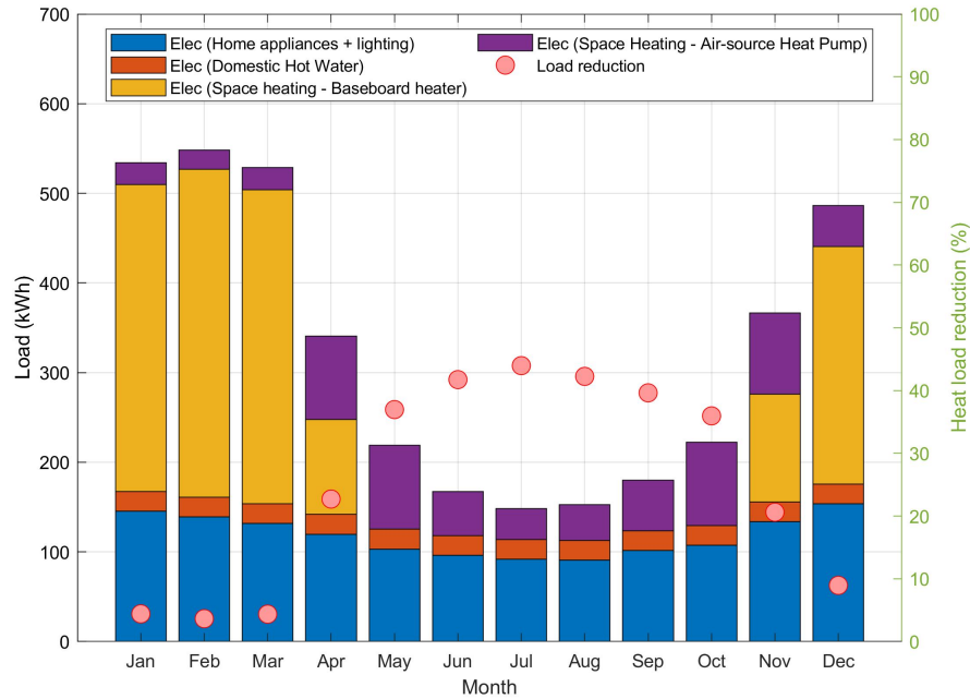
Figure 3.14: Scenario 3 heat load reduction caused by using ASHP and baseboard heater.
