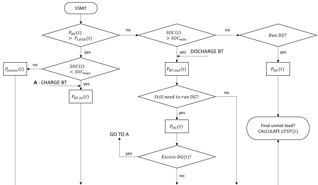
Figure 2.6: Flowchart of load following operation strategy.
