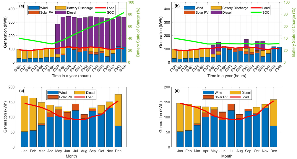
Figure 2.19: The solution with minimum LCOE and maximum fuel consumption was modified in terms of operation strategy to see the effect on the simulation results: (a) Hourly simulation results under Cycle Charging strategy; (b) Hourly simulation results under Load Following strategy; (c) Average monthly simulation results under Cycle Charging strategy; (d) Average monthly simulation results under Load Following strategy.
