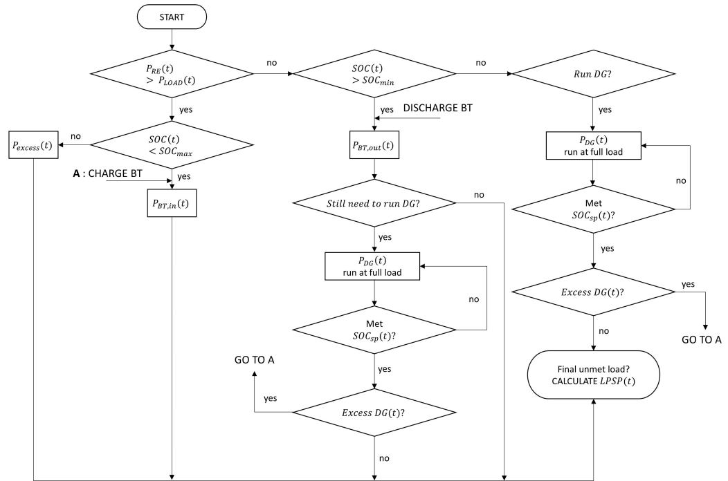
Figure 2.7: Flowchart of cycle charging operation strategy.
