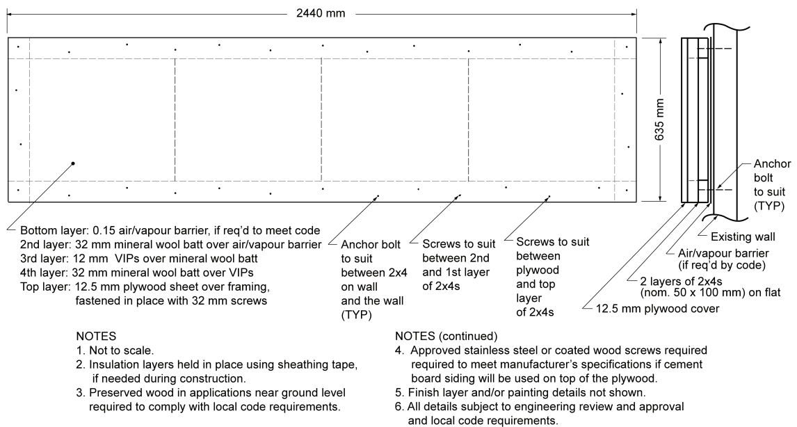
Fig. 3. Detail of Vacuum Insulation Panel (VIP) insulation to add RSI 5.5 nominal to an existing wall.
