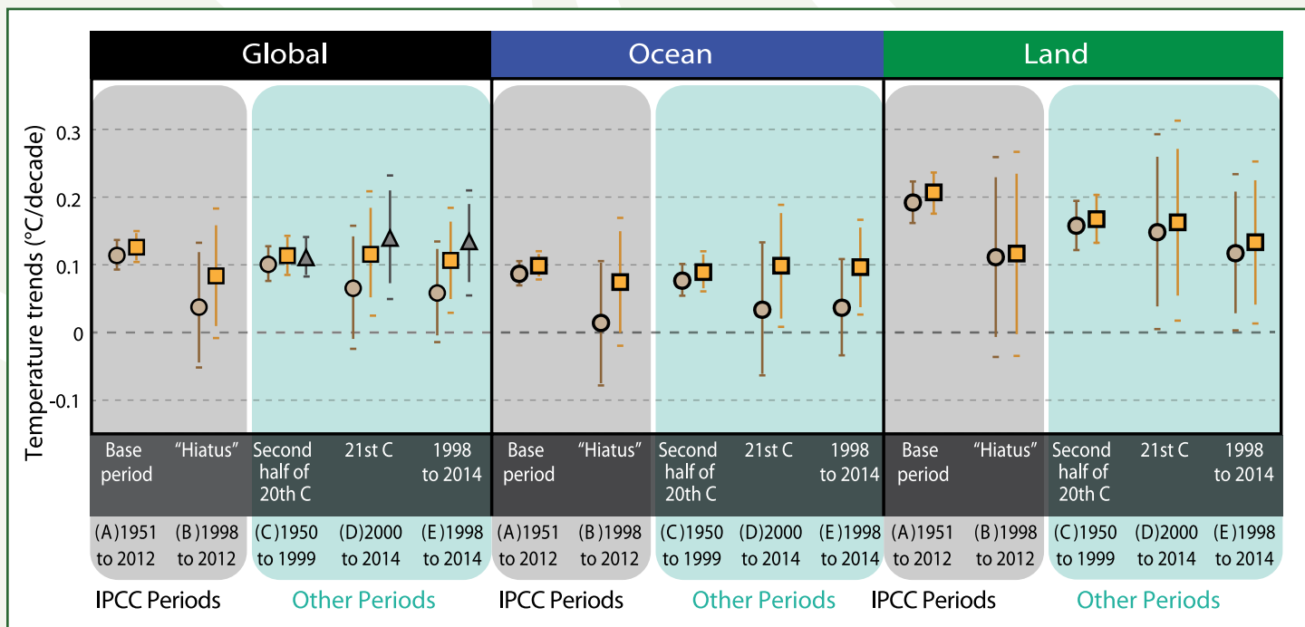
Figure 1: Global surface temperature trends, from Karl et al. (2015).
