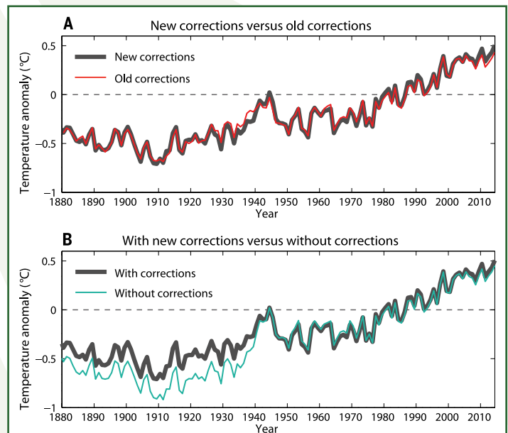
Figure 1: Global surface temperature anomalies, from Karl et al. (2015).
