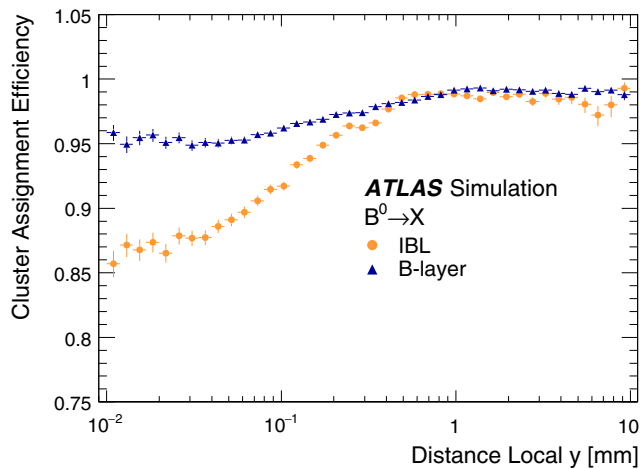
(e) B^0 \rightarrow X sample
