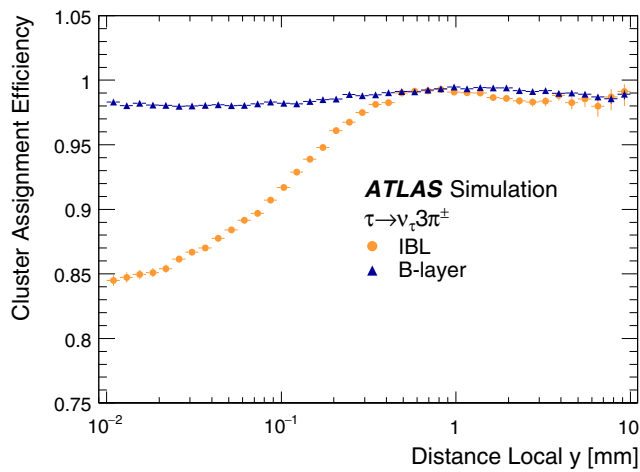
(c) \tau \rightarrow \pi^+\pi^-\pi^+\nu_\tau sample
