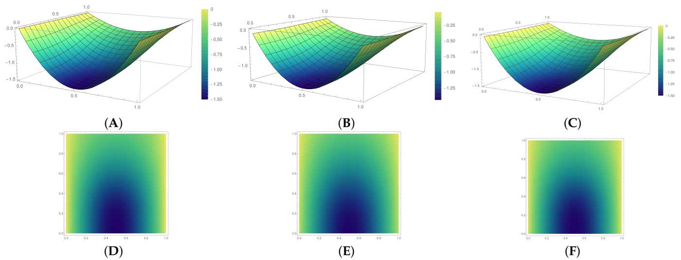
Figure 2. The function h_2(y,z) , and approximations for r,s = 20 and r,s = 60 with density graphs. (A) h_2(y,z) ; (B) r,s = 20 ; (C) r,s = 60 ; (D) is the density plot of (A); (E) is the density plot of (B); (F) is the density plot of (C).
