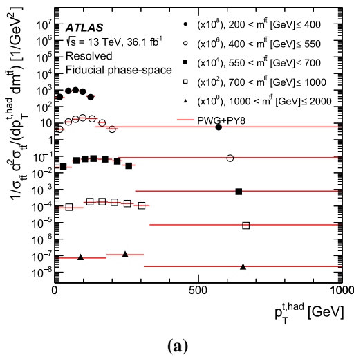
Fig. 26 a Particle-level normalised differential cross-section as a function of p_T^{t, had} in bins of m^{t\bar{t}} in the resolved topology compared with the prediction obtained with the POWHEG+PYTHIA8 MC generator. Data
