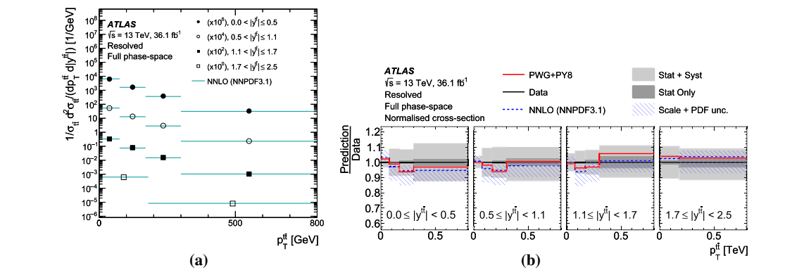
Fig. 61 a Parton-level normalised differential cross-section as a function of p_T^l in bins of |y^l| in the resolved topology compared with the NNLO prediction obtained using the NNPDF3.1 NNLO PDF set. Data points are placed at the centre of each bin. b The ratio of the measured
