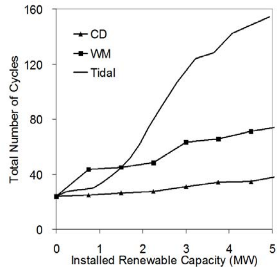
Figure 51: Total number of diesel generator cycles with all renewable options, linked grid with operational strategy
