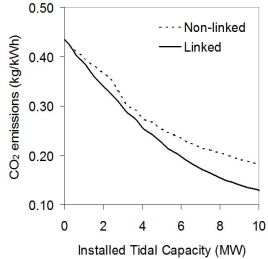
Figure 21: Average CO 2 emissions vs. installed tidal capacity
