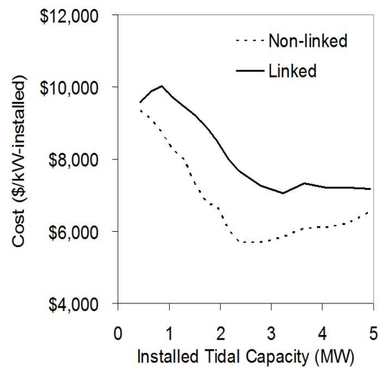
Figure 42: Simulation break even project cost vs. installed tidal capacity
