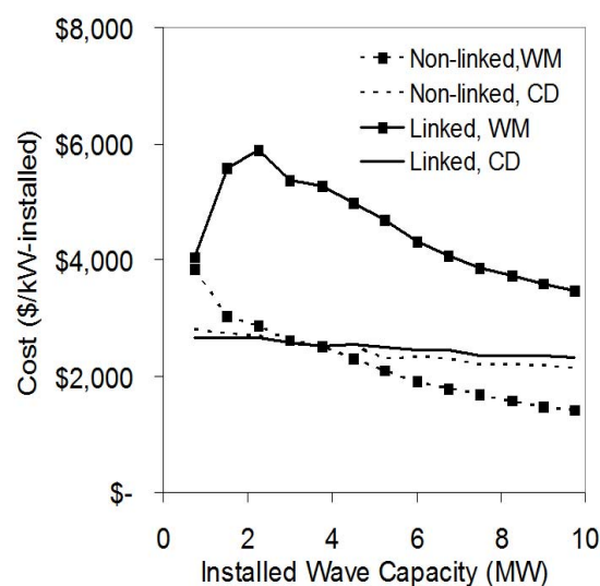
Figure 49: Simulation break even project cost vs. installed wave capacity
