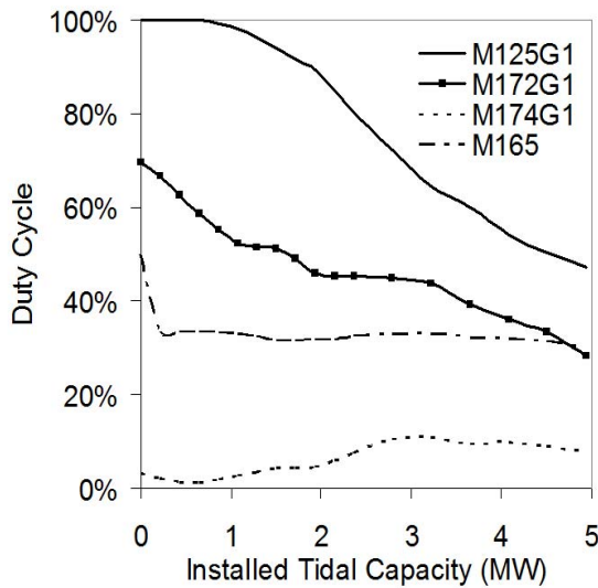
Figure 35: Simulation diesel generator duty
