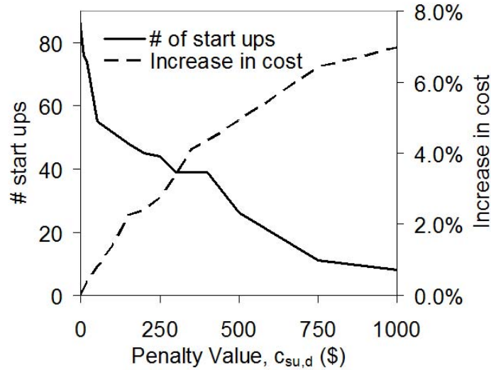
Figure 11: Sensitivity results for linked grids case, month of January data
