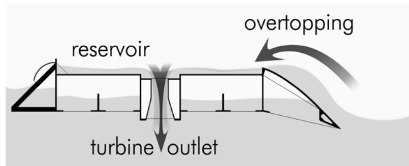
Figure 3: Wave Dragon operating principle [37]
