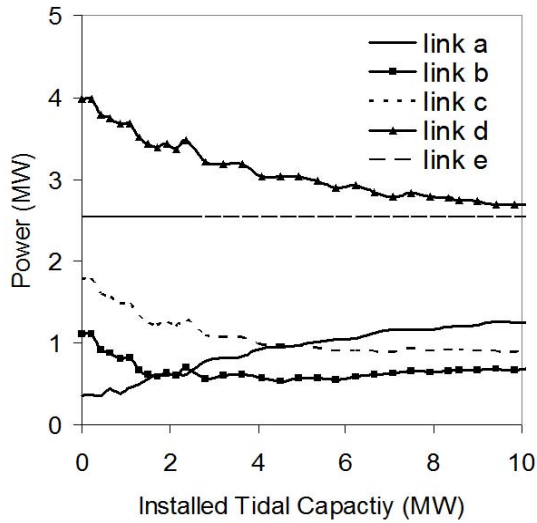
Figure 20: Average line power flow vs. installed tidal capacity, linked case
