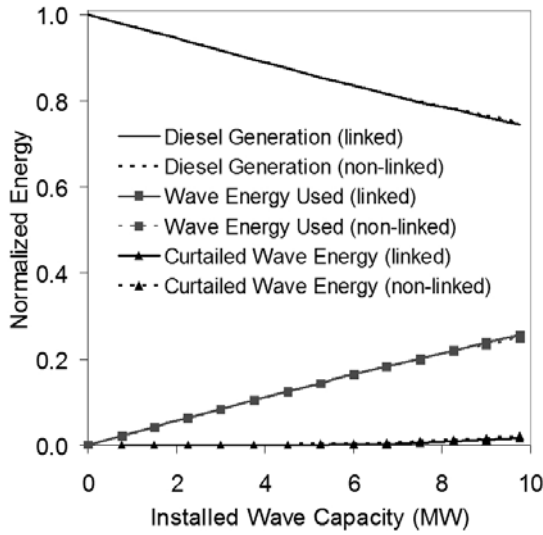
Figure 44: Simulation energy contribution by source vs. installed wave capacity, CD location
