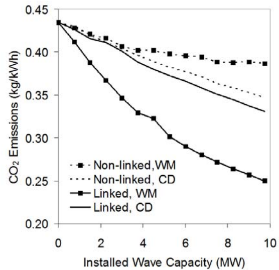
Figure 31: Average CO 2 emissions vs. installed wave capacity
