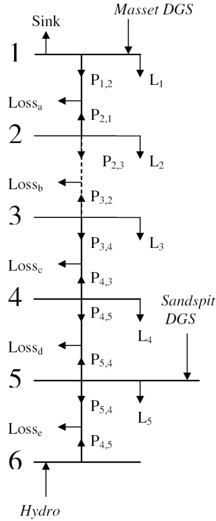
Figure 6: Network Diagram
