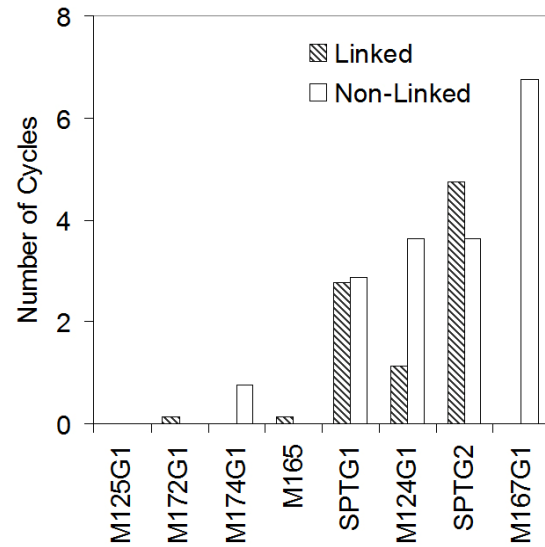
Figure 14: Average number of diesel generator cycles, no renewable power
