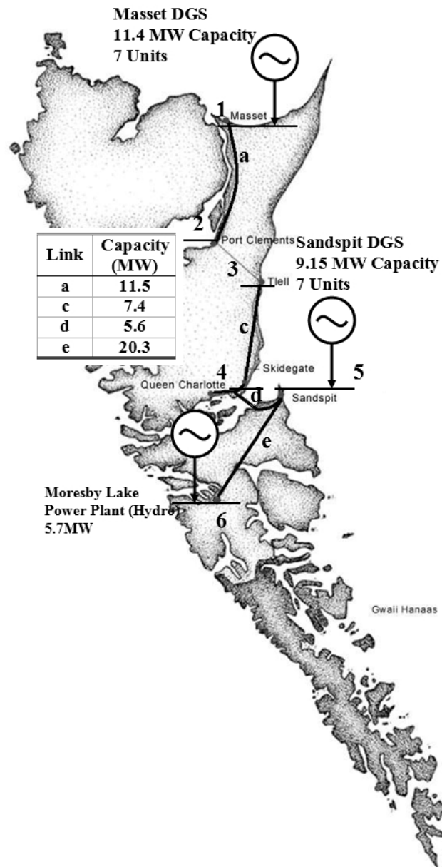
Figure 5: Haida Gwaii electricity system (data from [3])
