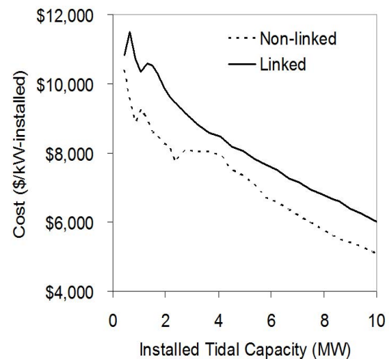
Figure 23: Break even project cost vs. installed tidal capacity
