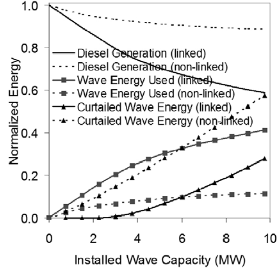
Figure 45: Simulation energy contribution by source vs. installed wave capacity, WM location
