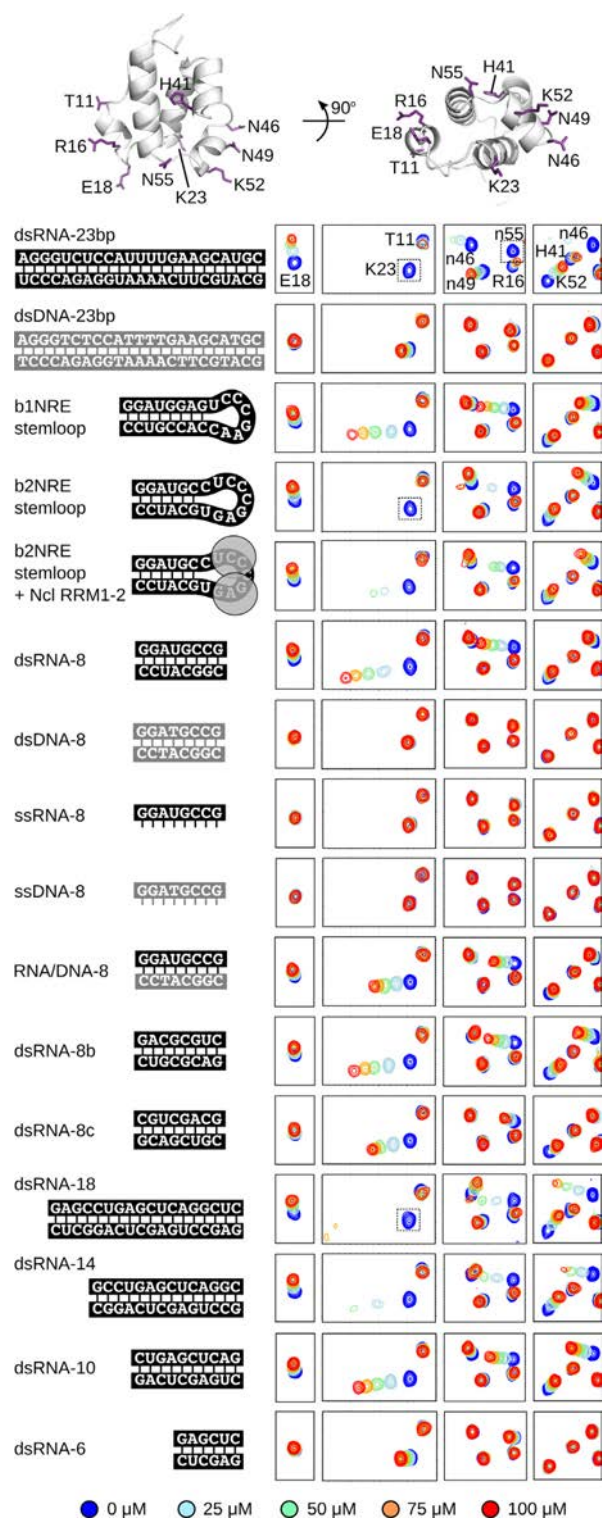
Figure 5. Binding preference for the isolated BTHB domain. Regions of NMR spectra following titration of various ligands into 100 \mu\text{M} ^{15}\text{N} -labelled FKBP25 (1-74) . The unbound spectrum is shown in blue, and the spectra following addition of 25, 50, 75 and 100 \mu\text{M} ligand are coloured light blue, light green, orange and red, respectively. The location of residues from the BTHB with annotated crosspeaks are indicated (top panel; atomic coordinates from PDB ID 2KFV) (23). Annotations with a small letter n correspond to the asparagine sidechain amide crosspeaks. Dotted boxes indicate peaks that broaden below detection upon addition of ligand. Full spectra are in Supplementary Figure S4.
