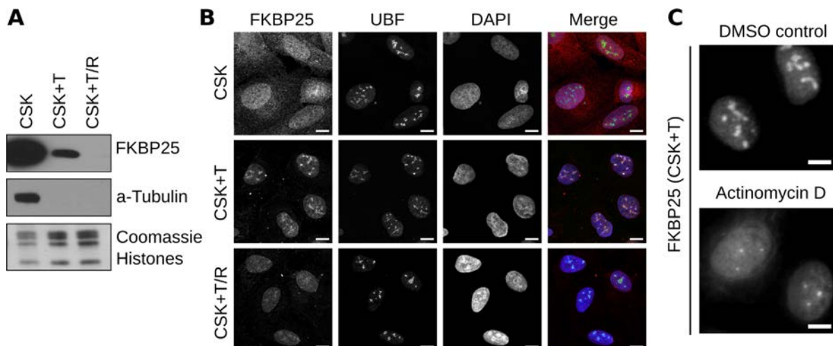
Figure 2. FKBP25 requires RNA for nucleolar localization. (A) Western blot analysis of U2OS cells following CSK treatment, with an additional Triton wash or a combination of Triton and RNaseA treatment. (B) Confocal microscopy of FKBP25 and the nucleolar-specific upstream binding factor (UBF). Cells were either untreated (CSK), pre-extracted with Triton (CSK + T), or pre-extracted with Triton and treated with RNaseA (CSK + T + R) prior to fixation. Scale bar is 10 \mu\text{m} . (C) Epi-fluorescence microscopy of FKBP25 in cells treated with DMSO or the RNA polymerase I inhibitor actinomycin D (10 nM for 4 h) and pre-extracted with CSK-T. Scale bar is 5 \mu\text{m} .
