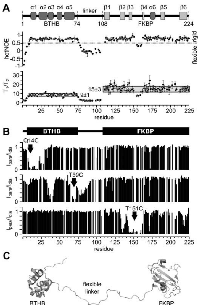
Figure 7. The BTHB and FKBP domains of FKBP25 are structurally independent. (A) ^{15}\text{N} relaxation measurements of ^{15}\text{N} -labelled FKBP25 at 298K using a 700 MHz NMR spectrometer. Heteronuclear \{^1\text{H}\}^{15}\text{N} NOE measurements for backbone amide nitrogen identify residues that are conformationally rigid (values greater than 0.5) or flexible (less than 0.5) at the ps-ns timescale. The ratio of T1 over T2 values results with differing values of 9 \pm 1 and 15 \pm 3 for the BTHB and FKBP domains, respectively. The secondary structure of FKBP25 is illustrated at the top. (B) Incorporation of the nitroxide compound TEMPO to the FKBP25 mutant Q14C, T69C and T151C. Distance-dependent attenuation of crosspeak intensities caused by the paramagnetic nitroxide are shown, and are restricted to intra-domain effects. Full analysis in Supplementary Figure S6. (C) The two domains of FKBP25 do not form a single structural unit in solution, but are only connected by the flexible linker.
