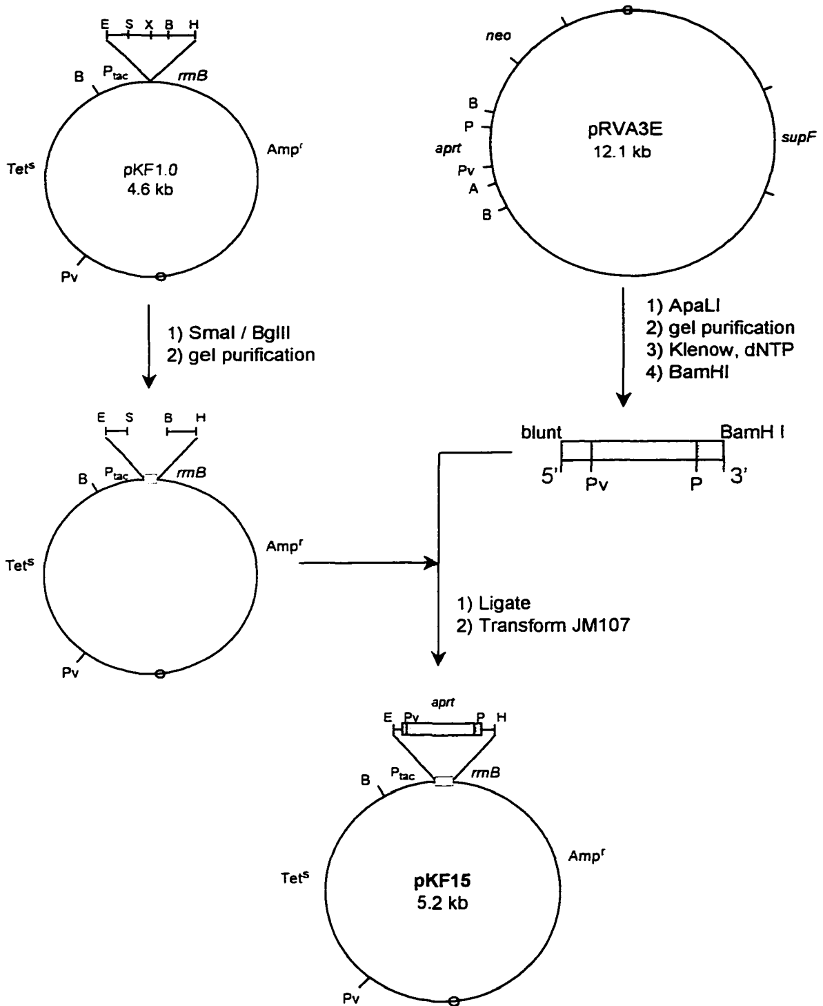
Figure 3.2 : Cloning aprt from pRVA3E into pKF1.0 (derived from pKK223-3, see Appendix I), as described in text. A; Apa LI (3' end of coding sequence, single site in aprt , multiple unmapped sites in vector), B; Bam HI, E; Eco RI, H; Hind III, P; Pst I, Pv; Pvu II (marks 5' end of coding sequence), S; Sma I, X; Xba I.
