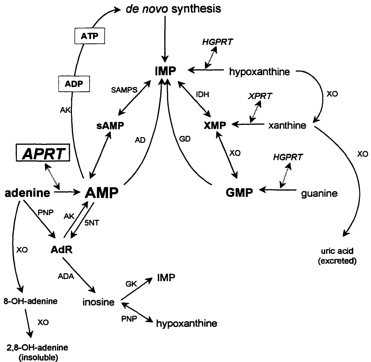
Figure 1.1 : The relationship of adenine phosphoribosyl transferase (APRT) to other components of purine metabolism, the central role of IMP, and the interconversion and alternate salvage of purine bases. In some species ( e.g. E. coli ), hypoxanthine-guanine phospho-ribosyl transferase (HGPRT) is replaced by two discrete enzymes, HPRT and GPRT. Cofactors and cosubstrates are not indicated. Alternate salvage of guanine, hypoxanthine, and xanthine, to their respective nucleosides, by purine nucleoside phosphorylase and 5' nucleotidase, is not shown. AD; adenylylate deaminase. AdR; adenosine. AK; adenosine kinase. AMP; adenosine monophosphate. GD; guanylate deaminase. GK; guanosine kinase. GMP; guanosine monophosphate. IDH; IMP dehydrogenase. IMP; inosine monophosphate. PNP; purine nucleoside phosphor-ylase. SAMPS; adenylosuccinate synthetase. sAMP; succinyl AMP. XO; xanthine oxidase. XMP; xanthine monophosphate. XPRT; xanthine phosphoribosyl transferase
