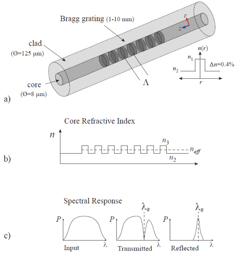
Figure 4: Fibre Bragg Grating fundamentals. a) dark shaded areas indicated fibre core volumes of altered index of refraction b) periodic stepped-index of refraction profile in the fibre core along axis. c) spectral response of an FBG. Image reprinted with permission from N. David [25].
