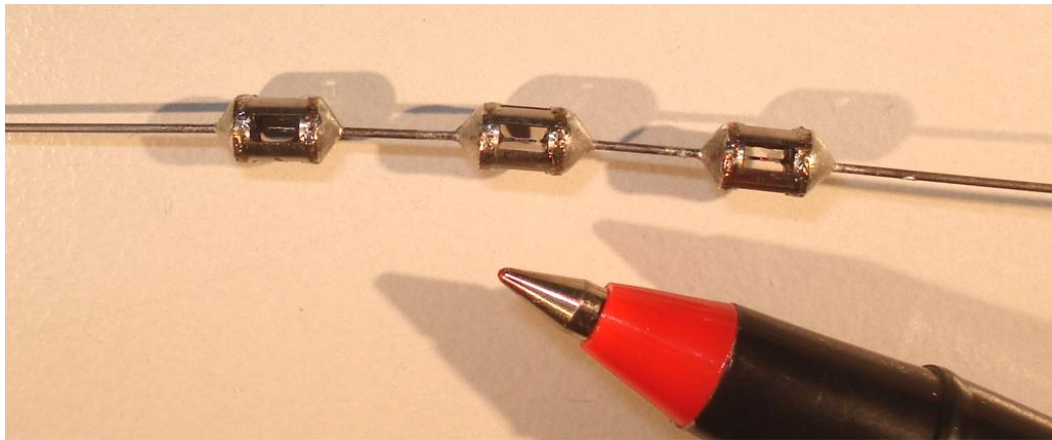
Figure 23: Typical three-pod prototype in hydrodynamic configuration. Shown here is a three-grating sensor; indistinguishable from the single-grating variant.
