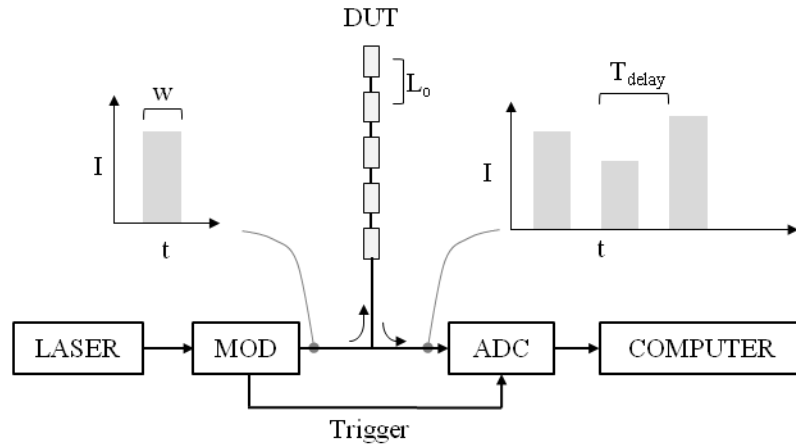
Figure 10: TDM schematic. MOD is a high frequency modulator, ADC is an analogue to digital converter. Top left plot represents interrogation pulse into the Device Under Testing, DUT, and the top right plot shows the resulting pulse train incident on the ADC (only the first three pulses are shown for clarity). Pulse intensities in the pulse train yield strain.
