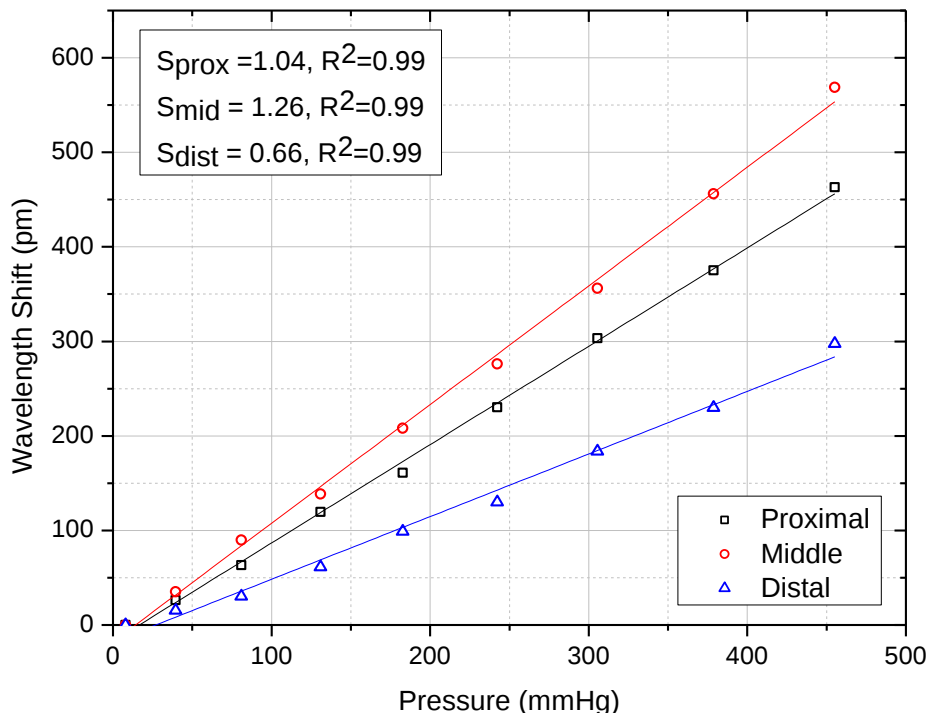
Figure 39: Sensitivity to hydrostatic pressure in contact-sensitive configuration
