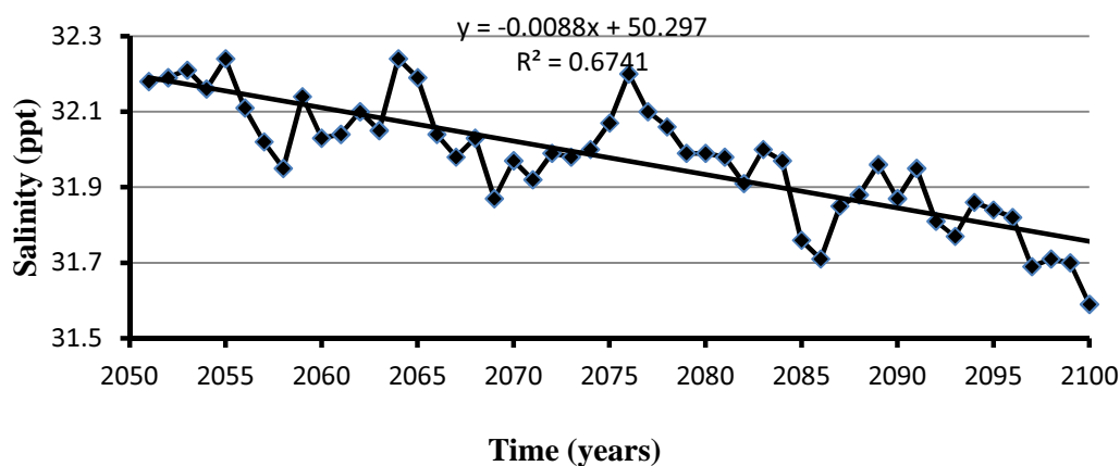
Figure 13: Projected SSS (2051-2100) of open ocean adjacent waters to the BC's coast
