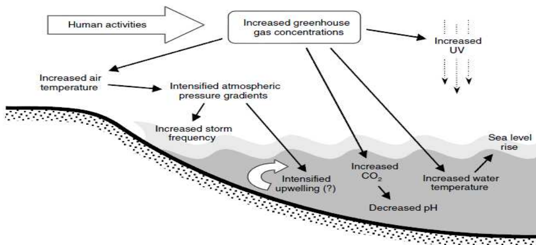
Figure 4: Important abiotic changes associated with climate change
