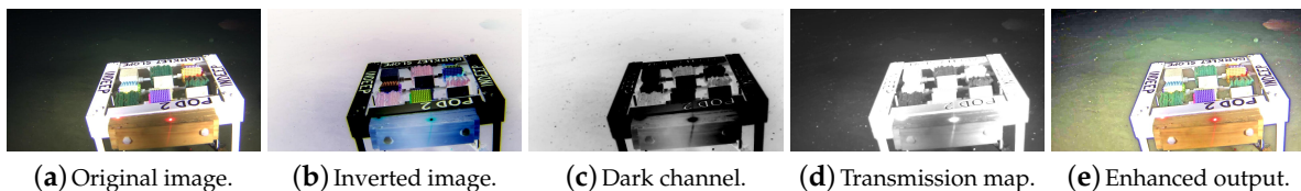
Figure 2. OceanDark 's sample enhancement process using static patch sizes of 5 \times 5 and \omega = 0.9 . The original image (a) is first inverted, turning the dark regions into hazy segments (b). The dehazing process involves the calculation of the dark channel (c) and transmission map (d) of the inverted image. The haze-less version of the image is obtained and inverted again for the final output (e).
