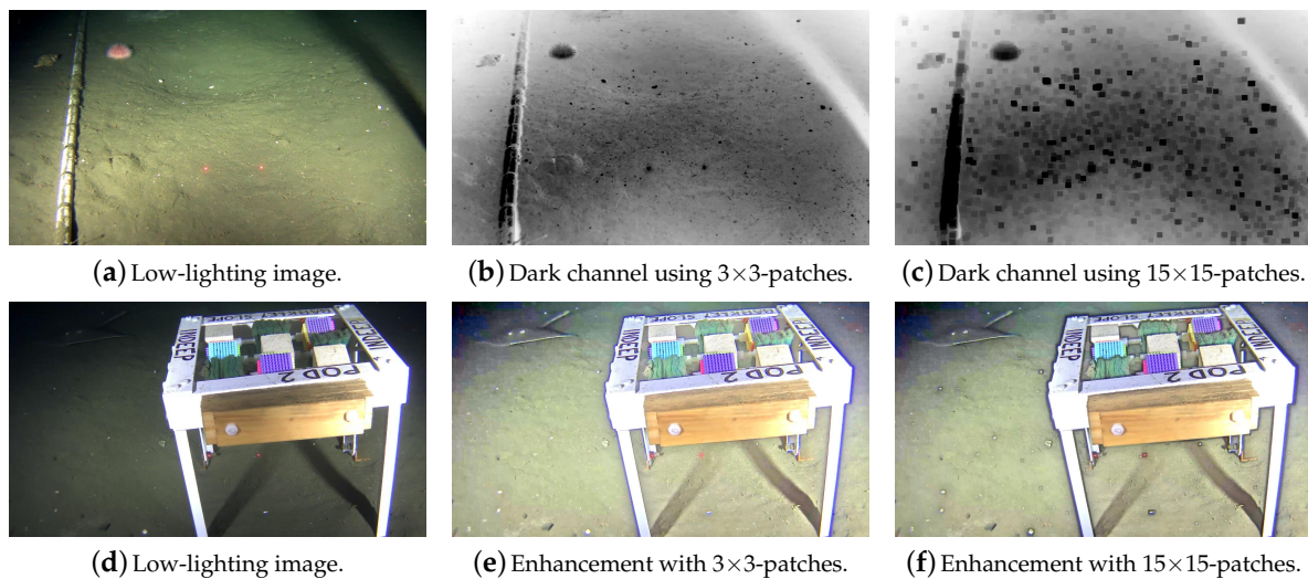
Figure 4. Dehazed scenes and dark channels obtained using \Omega_{3 \times 3} and \Omega_{15 \times 15} . The first row shows a low-lighting image (a) and its DC when using \Omega_{3 \times 3} (b) and \Omega_{15 \times 15} (c). The mean intensity of the latter is lower, resulting in a darker DC. The second row shows the results of enhancing a low-lighting image (d) with \Omega_{3 \times 3} (e) and \Omega_{15 \times 15} (f).
