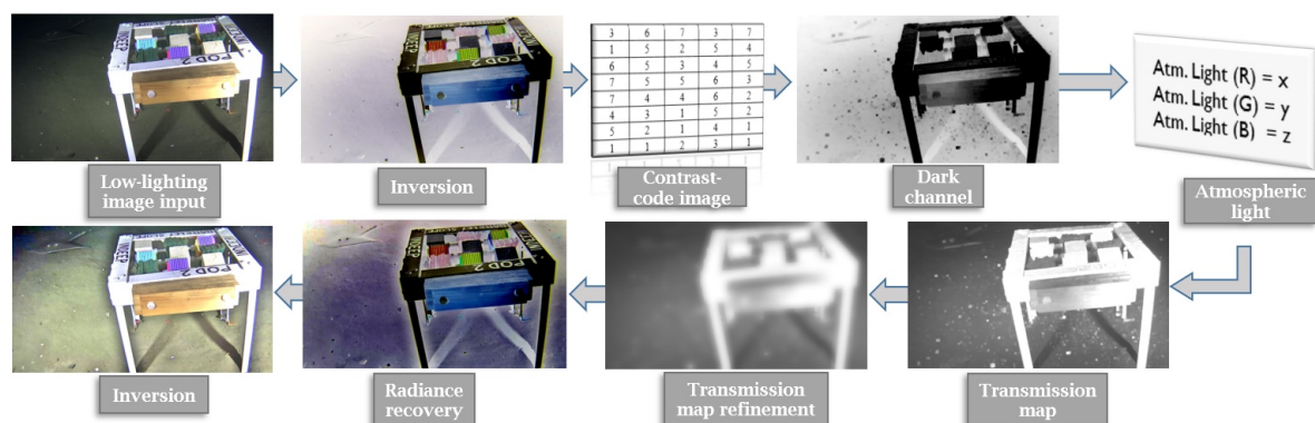
Figure 1. Low-lighting underwater image enhancement framework applied to a sample low-lighting underwater image from OceanDark . The image is initially inverted, and then put through a novel, contrast-guided dehazing process before being inverted once again. The output better highlights important features and structures of the original image that were not clearly visible in the original image.
