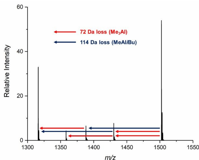
Figure 2. Partial MS/MS spectrum of the [Me_{32}iBu_3Al_{22}O_{16}]^- species (i.e. 16,6 after three Me for Bu exchanges) at m/z 1501. Initial two losses shown only to illustrate preference for i Bu loss of Me for full spectrum see Supplemental Information Figure S11.
