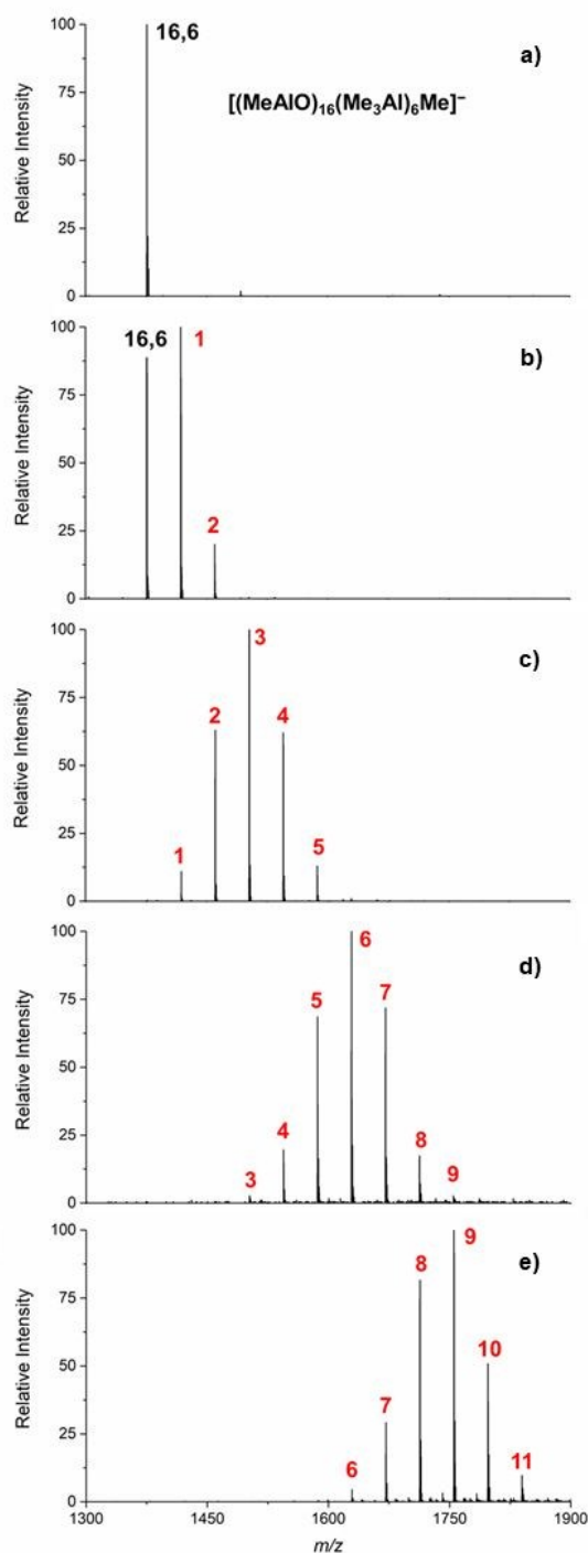
Figure 1. Room temperature negative ion ESI-MS spectra in PhF of 30 wt% MAO at equilibrium (5 minutes after mixing), (a) modified with 1 mol% i\text{Bu}_3\text{Al} (b), 5 mol% i\text{Bu}_3\text{Al} (c), 10 mol% i\text{Bu}_3\text{Al} (d), 20 mol% i\text{Bu}_3\text{Al} (e). All at an OMTS:Al ratio of 1:100. Number of Me/Bu substitutions in [(\text{MeAlO})_{16}(\text{Me}_3\text{Al})_6\text{Me}]^- is shown in red.
