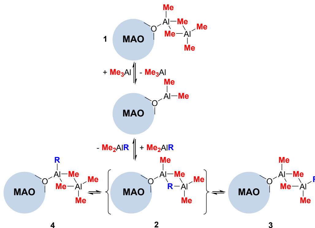
Scheme 1. Alkyl exchange between MAO and \text{Me}_2\text{AIR} .
