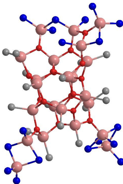
Figure 6. Optimized structure for neutral (MeAlO)_{16}(Me_3Al)_6 (Al pink, O red, and C grey).
