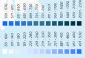
R95P Wettest Day Precipitation - Future (2050)
