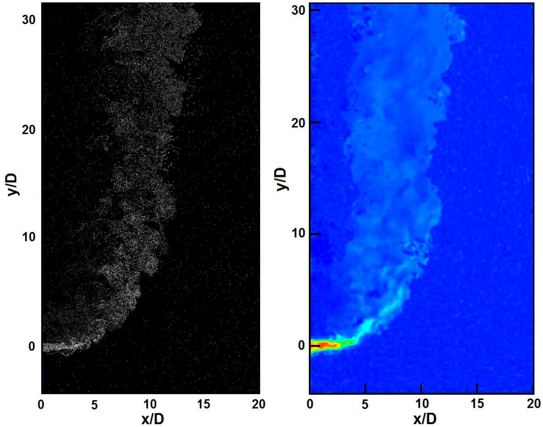
Figure 3.31 – Instantaneous PIV image (left), Corresponding Velocity Field (Right), Fr = 250
