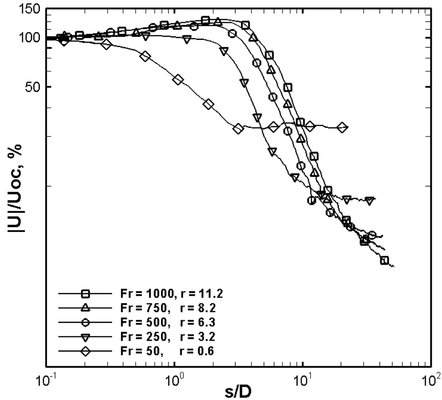
Figure 3.23 – Jet centerline time-averaged velocity magnitude decay normalized by jet diameter, D
