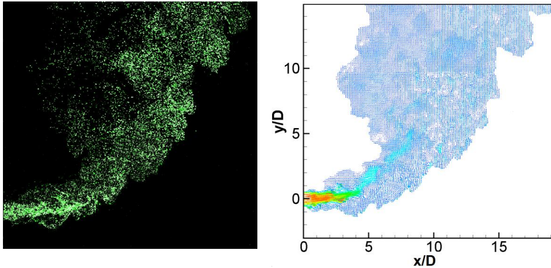
Figure 1.2 – PIV principles, Particles instantaneous image (Left), corresponding velocity field (Right).
