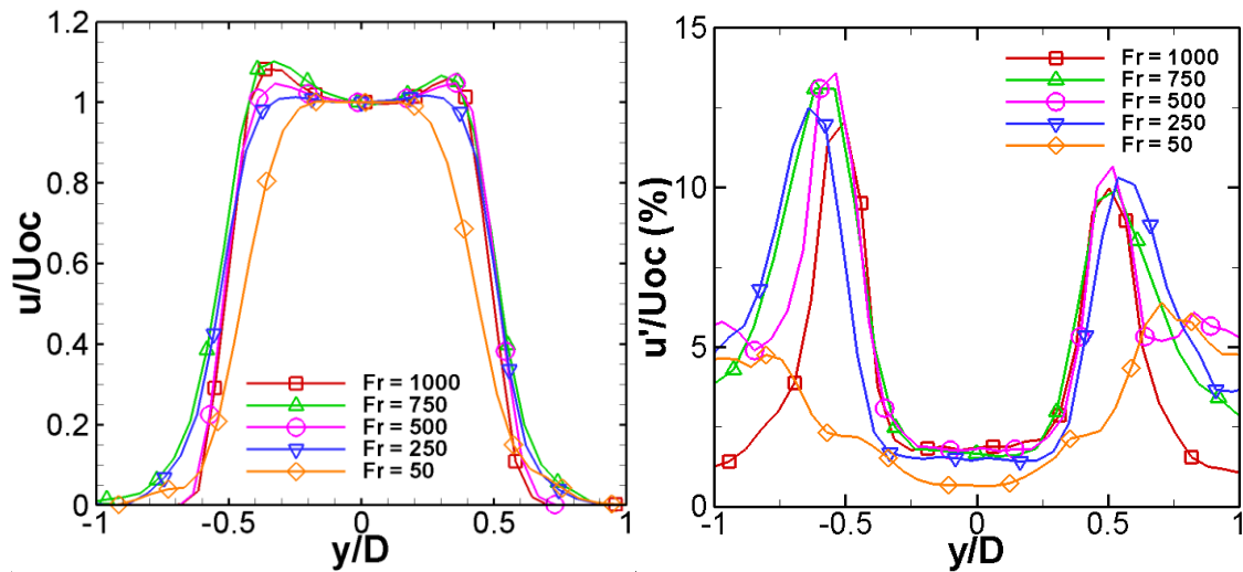
Figure 2.2 – Initial normalized radial mean velocity profile (left) and normalized radial rms values (right)
