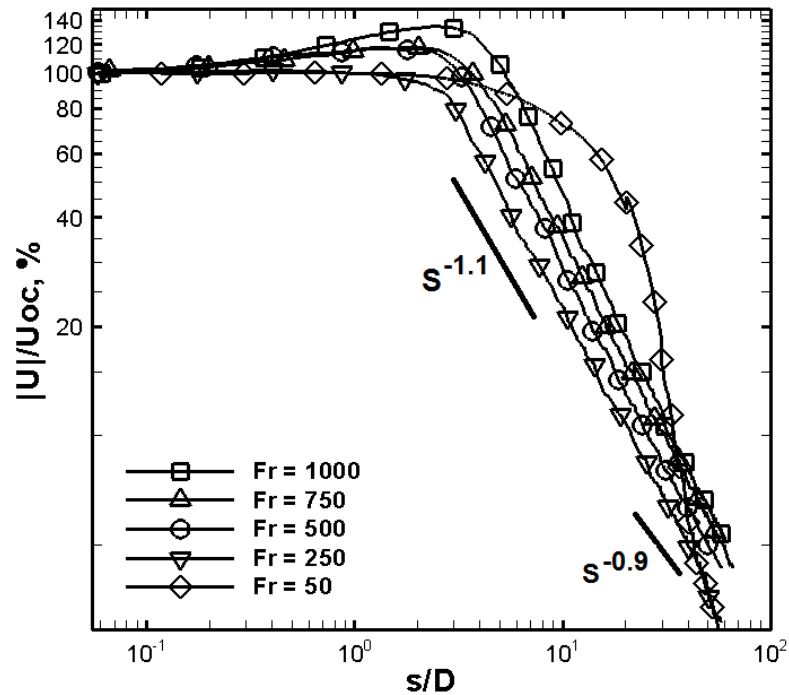
Figure 3.8 – Jet centerline mean velocity magnitude decay, free jet cases.
