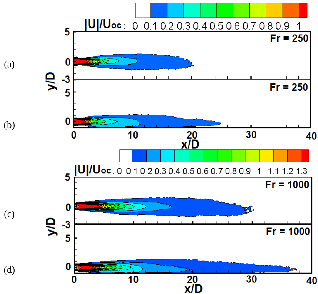
Figure 3.42 – Time-averaged velocity fields (a) Fr = 250 at 3D , (b) Fr = 250 at 1D , (c) Fr = 1000 at 3D and (d) Fr = 1000 at 1D distance from the ground surface.
