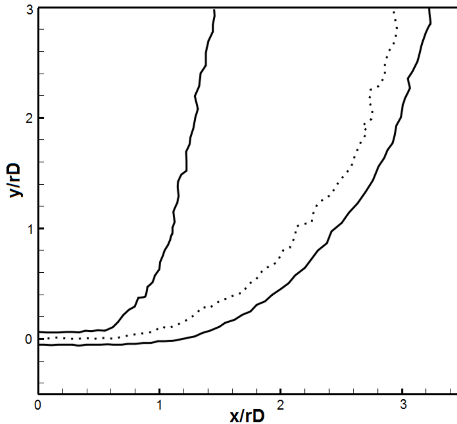
Figure 3.36 – Boundary contours for time-averaged velocity field, Fr = 1000 .
