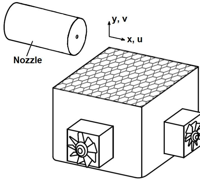
Figure 2.3 – schematics of the crossflow apparatus
