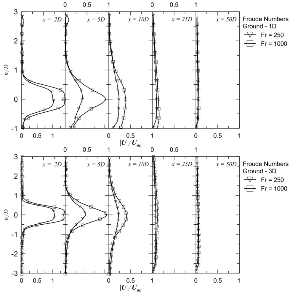
Figure 3.49 – Normalized velocity profiles for jets near the ground surface with nozzle to surface distance of 1D (top) and 3D (bottom).
