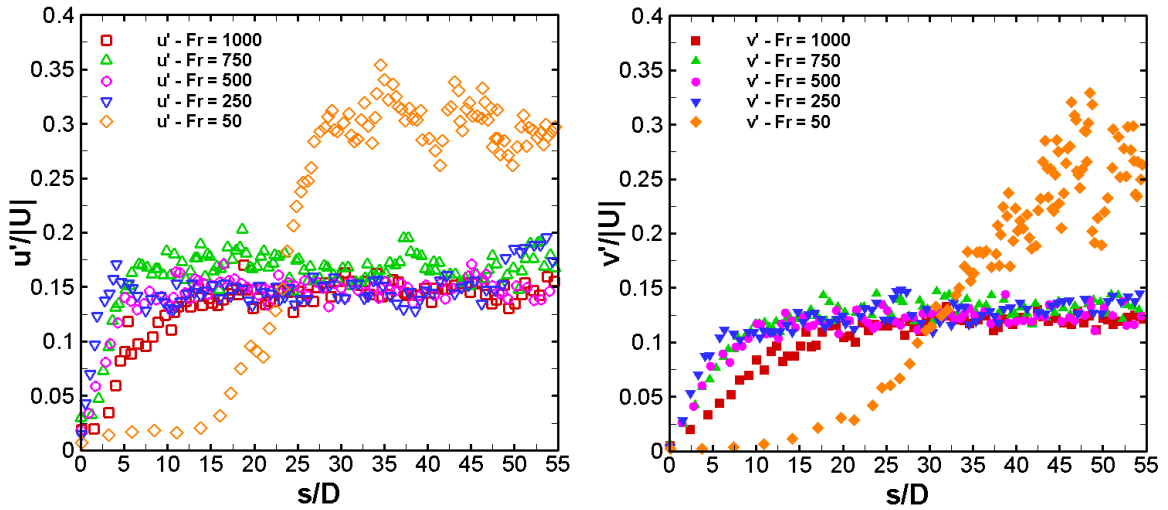
Figure 3.11 – Normalized velocity fluctuations along jet center line, free jet cases, axial- (left) and radial-velocity fluctuations (right).
