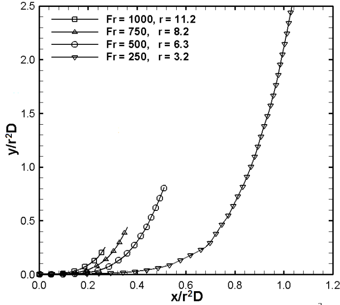
Figure 3.20 – Jet centerline representation normalized by r^2D .
