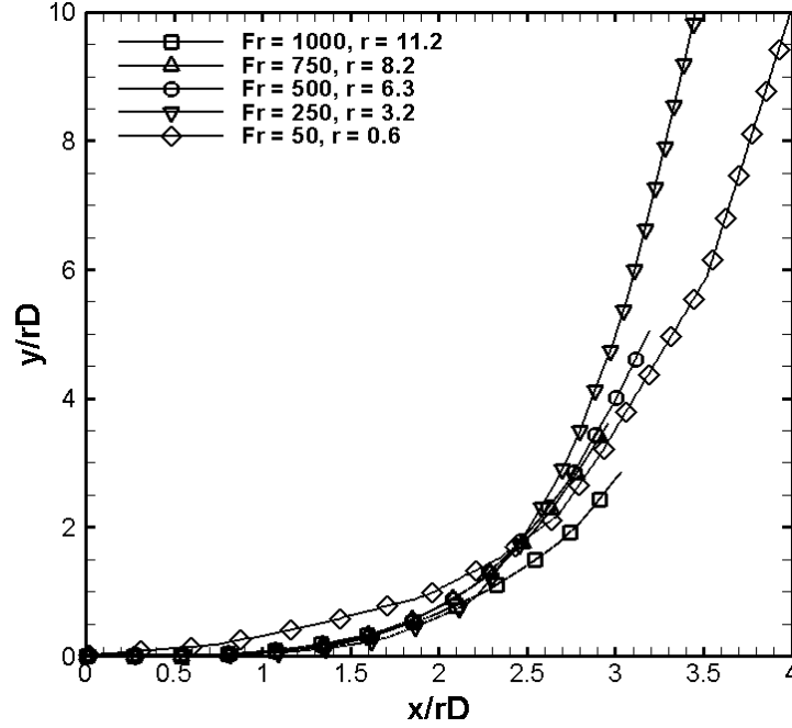
Figure 3.21 – Jet centerline representation normalized by rD .
