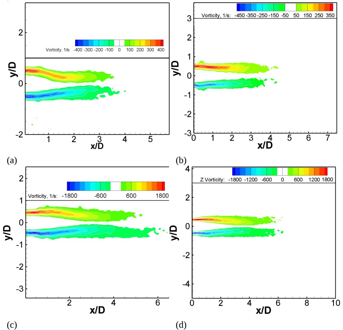
Figure 3.65 – Time-averaged out-of-plane vorticity contours for Fr = 250 located at (a) 1D, (b) 3D and Fr = 1000 located at (c) 1D and (d) 3D from the ceiling surface.
