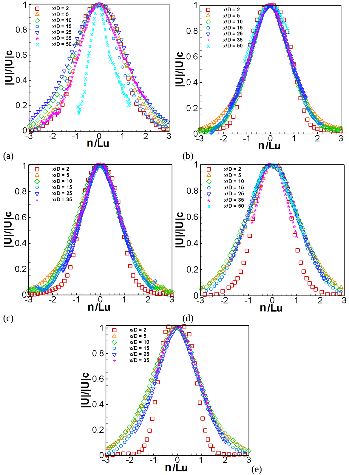
Figure 3.9 – Radial profiles of the normalized time-averaged velocity. Fr = (a) 50, (b) 250, (c) 500, (d) 750 and (e) 1000.
