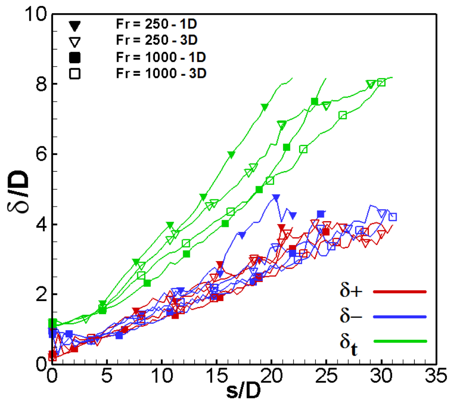
Figure 3.74 – Flow width, Jet near the vertical wall surface.
