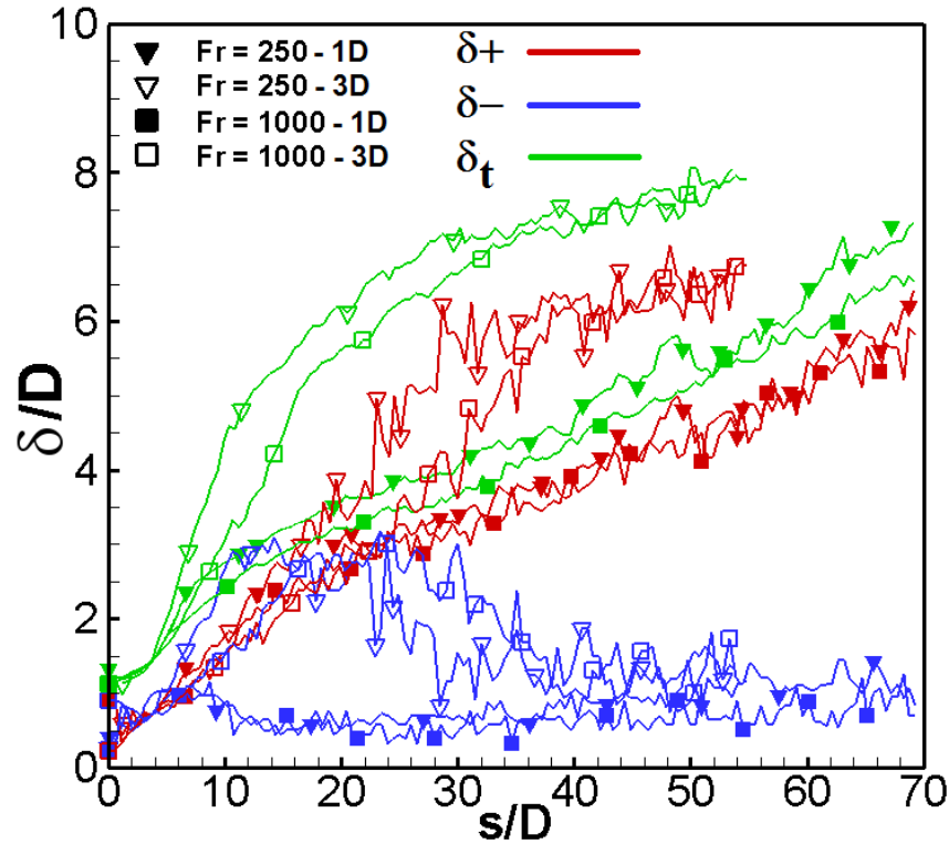
Figure 3.70 – Flow width, Jet near the ground surface.
