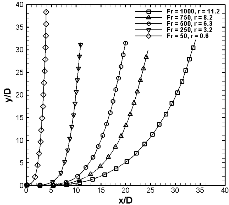
Figure 3.19 – Jet centerline representation normalized by D .
