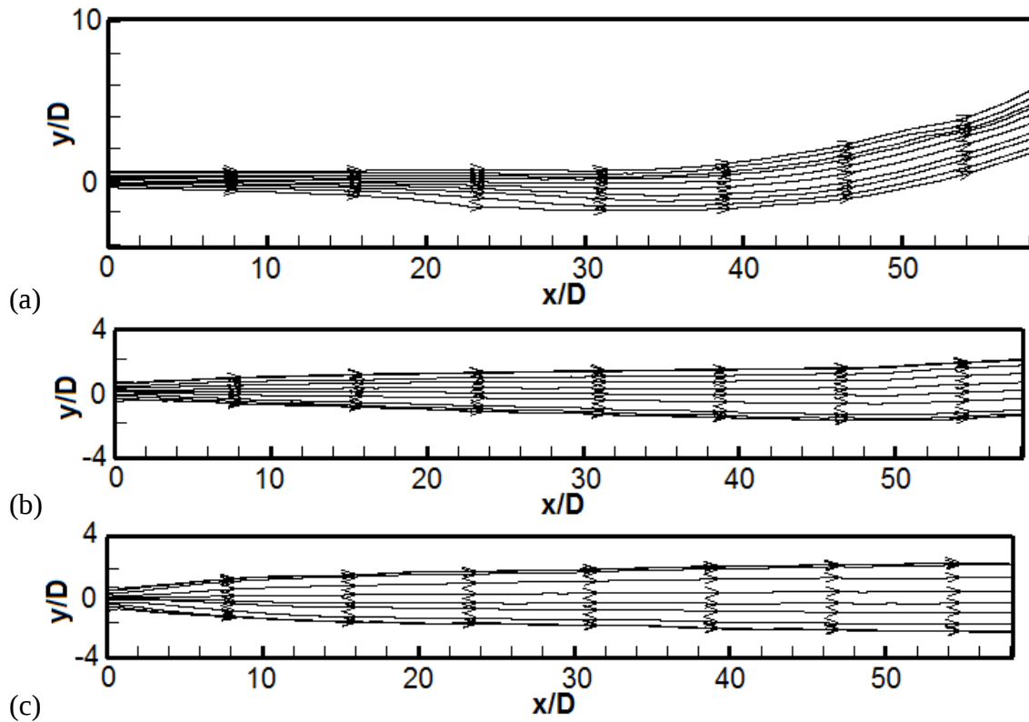
Figure 3.14 – Time-averaged streamlines Fr = (a) 50, (b) 250, (c) 1000.
