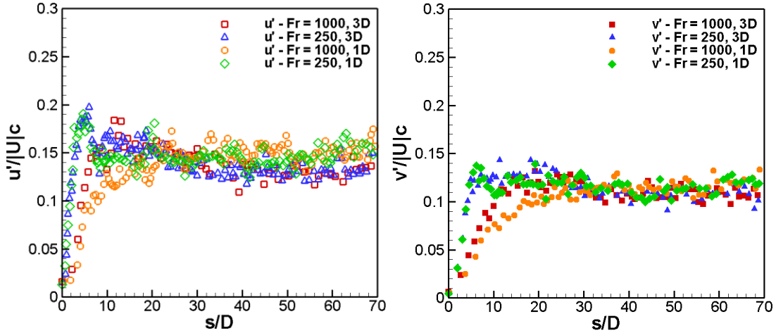
Figure 3.60 – Normalized velocity fluctuations along jet center line, jet near vertical wall surface.
