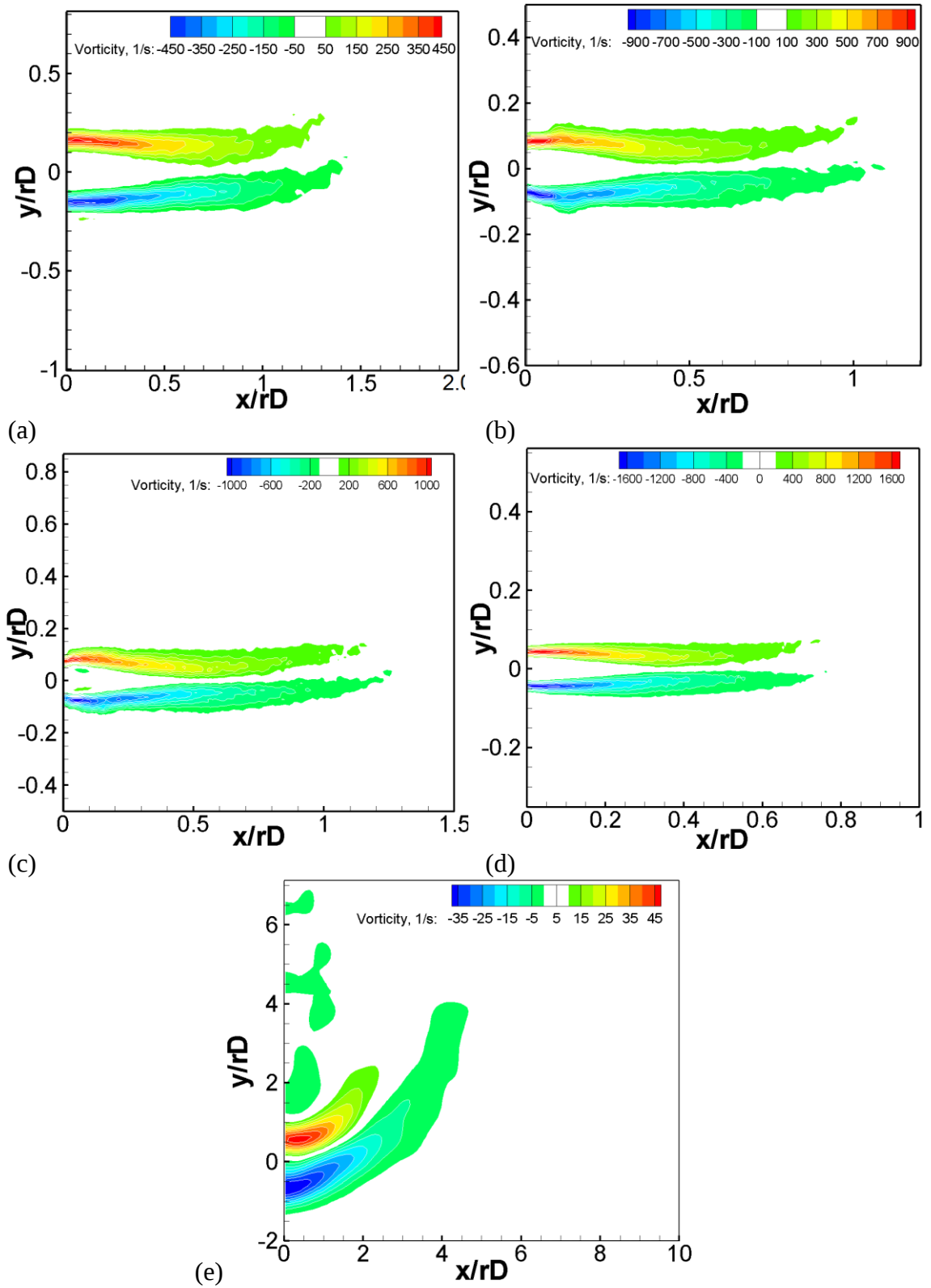
Figure 3.33 – Time-averaged out-of-plane vorticity contours Fr = (a) 250, (b) 500, (c) 750, (d) 1000 and (e) 50.
