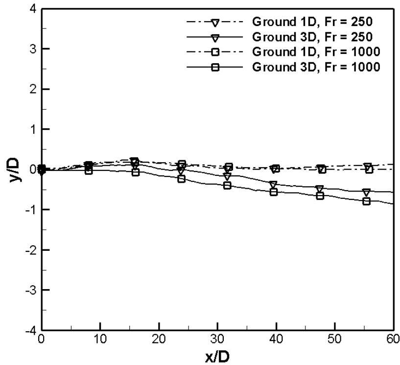
Figure 3.39 – Jet centerline representation for ground boundary normalized by D .
