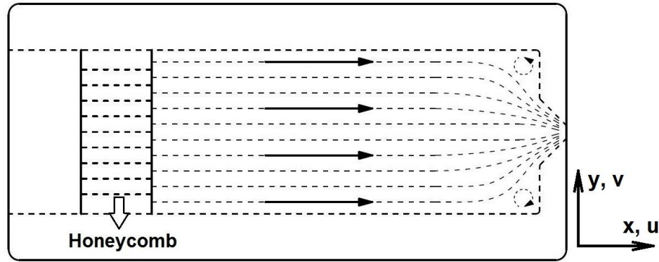
Figure 2.1 – Sharp-edged nozzle schematic
