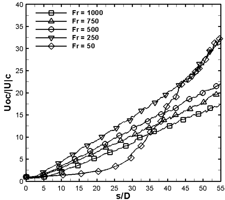
Figure 3.7 – Jet spread rate, free jet cases.
