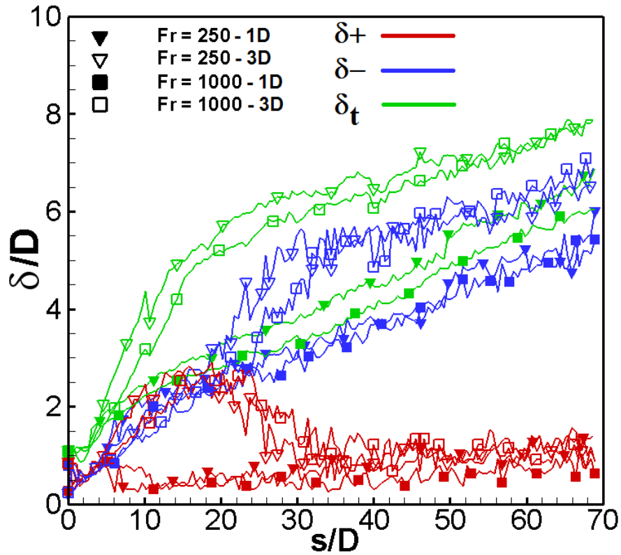
Figure 3.72 – Flow width, Jet near the ceiling surface.
