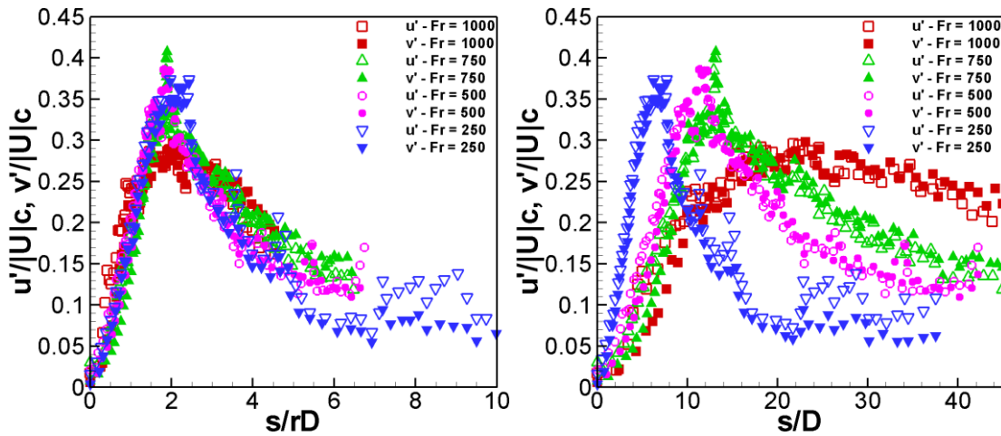
Figure 3.28 – Normalized velocity fluctuations along jet center line, jet in crossflow, jet centerline normalized by rD (left) and nozzle diameter (right).
