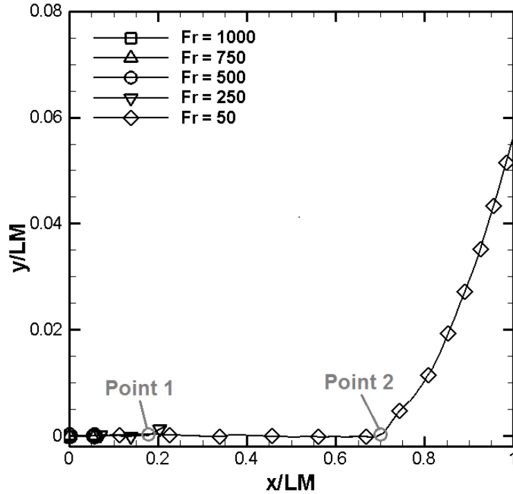
Figure 3.6 – Jet centerlines for free jet cases using L_M length scale.
