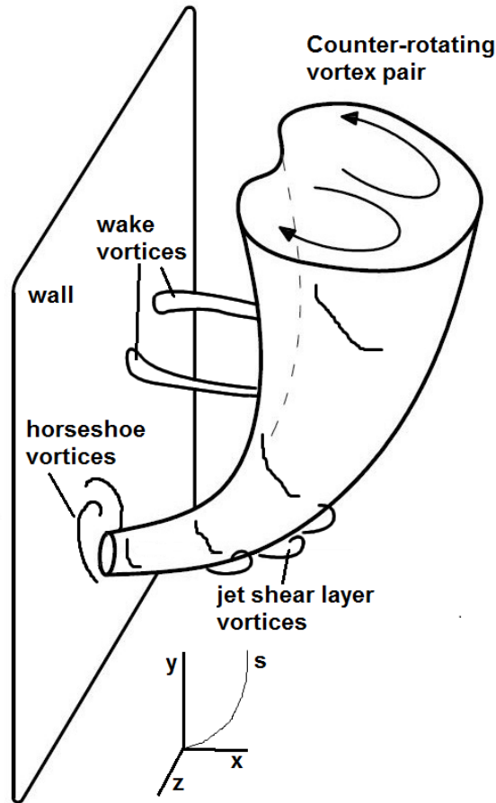
Figure 3.30 – Schematics of jet in crossflow vortical structure (re-drawn from (Fric and Roshko 1994))
