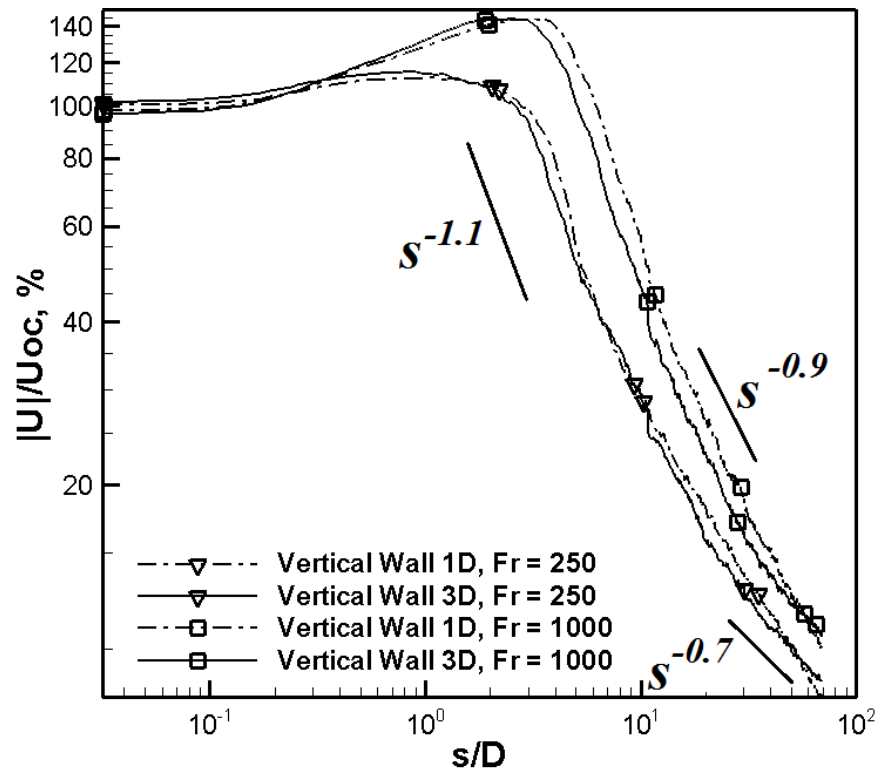
Figure 3.47 – Centerline velocity decay rates for vertical wall boundary.
