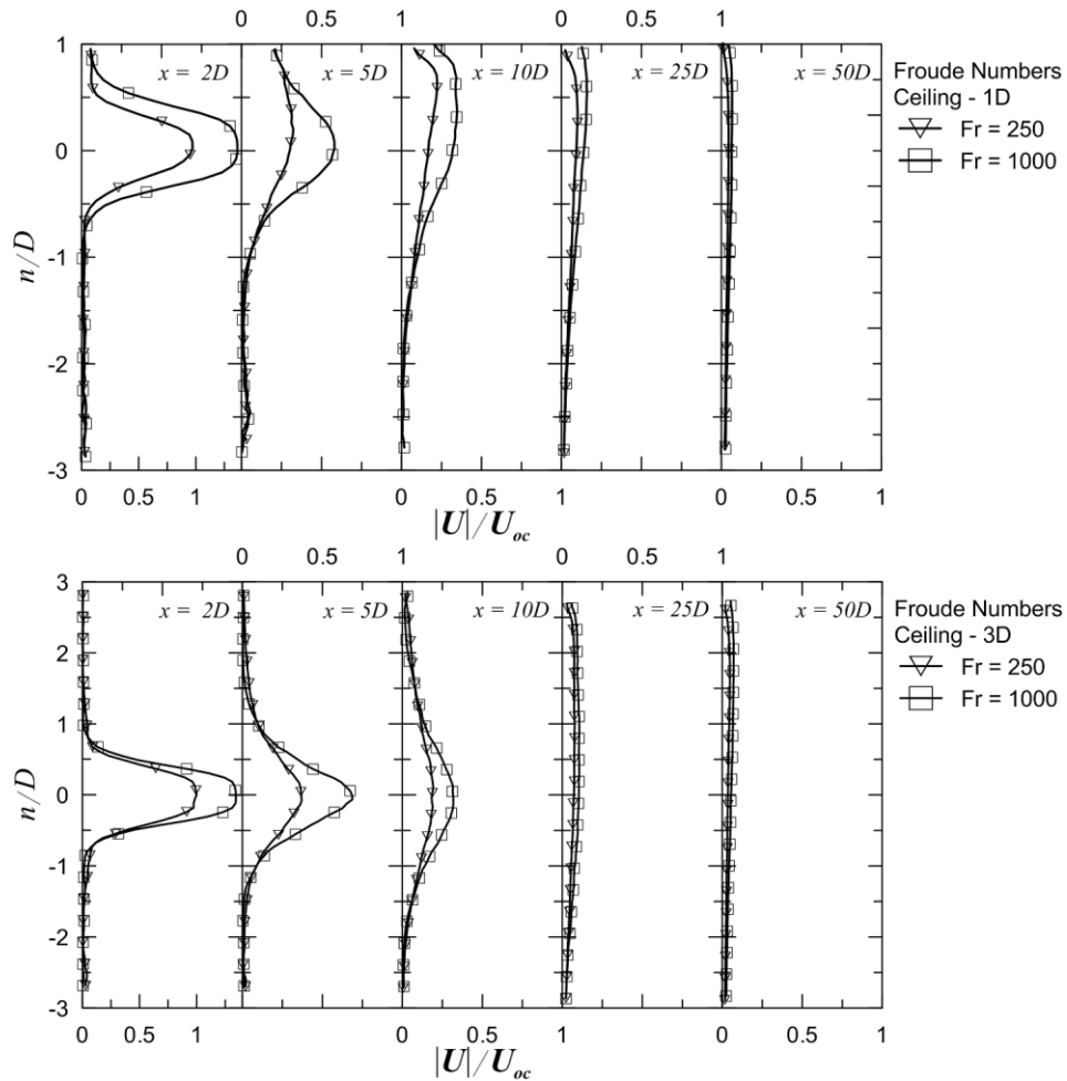
Figure 3.51 – Normalized velocity profiles for jets near the ceiling surface with nozzle to surface distance of 1D (top) and 3D (bottom).
