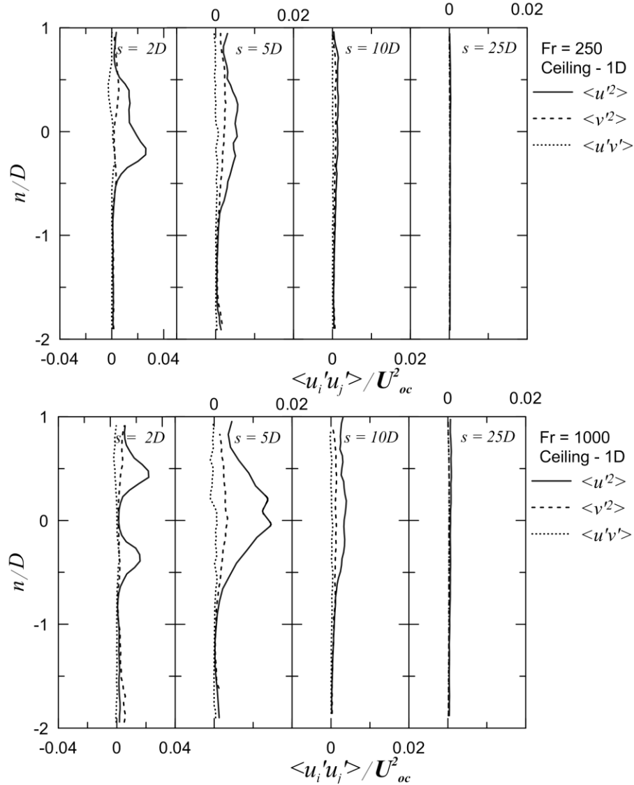
Figure 3.59 – Stress profiles in jet center-plane for jets located at 1D from ceiling surface (a) Fr = 250 , (b) Fr = 1000 .
