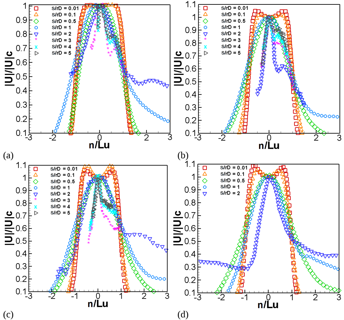
Figure 3.26 – Radial velocity profiles, jet in crossflow Fr = (a) 250, (b) 500, (c) 750 and (d) 1000.
