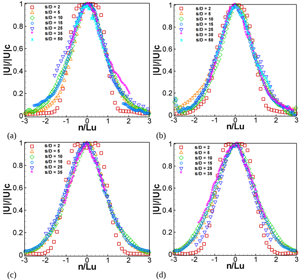
Figure 3.52 – Radial profiles of the time-averaged velocity, jet near vertical wall surface, Fr = 250 located at (a) 1D, (b) 3D and Fr = 1000 located at (c) 1D and (d) 3D from the vertical wall.
