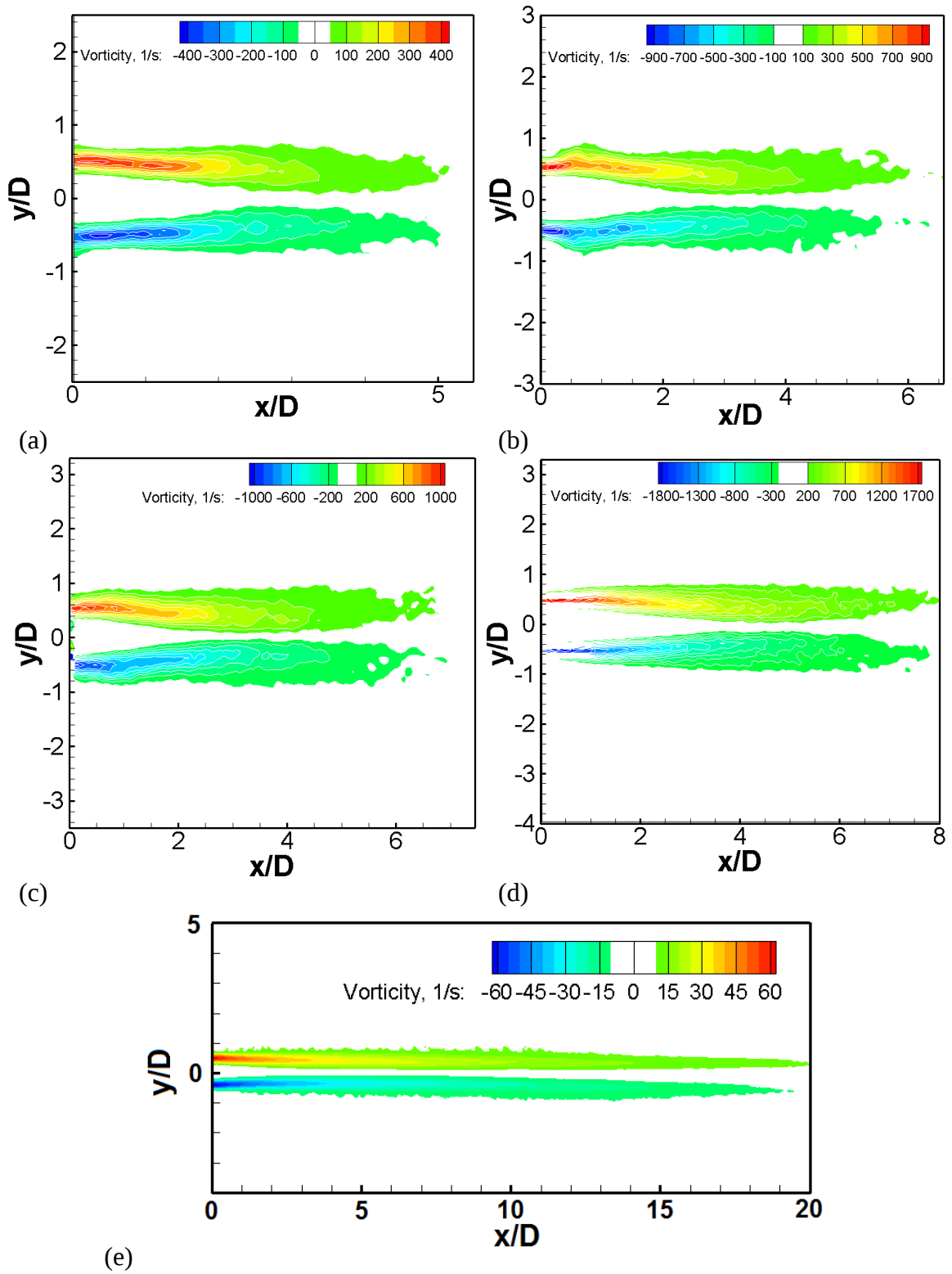
Figure 3.13 – Time-averaged out-of-plane vorticity contours Fr = (a) 250, (b) 500, (c) 750, (d) 1000 and (e) 50.
