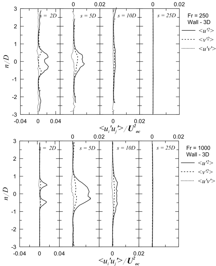
Figure 3.61 – Stress profiles in jet center-plane for jets located at 3D from vertical wall surface (a) Fr = 250 , (b) Fr = 1000 .
