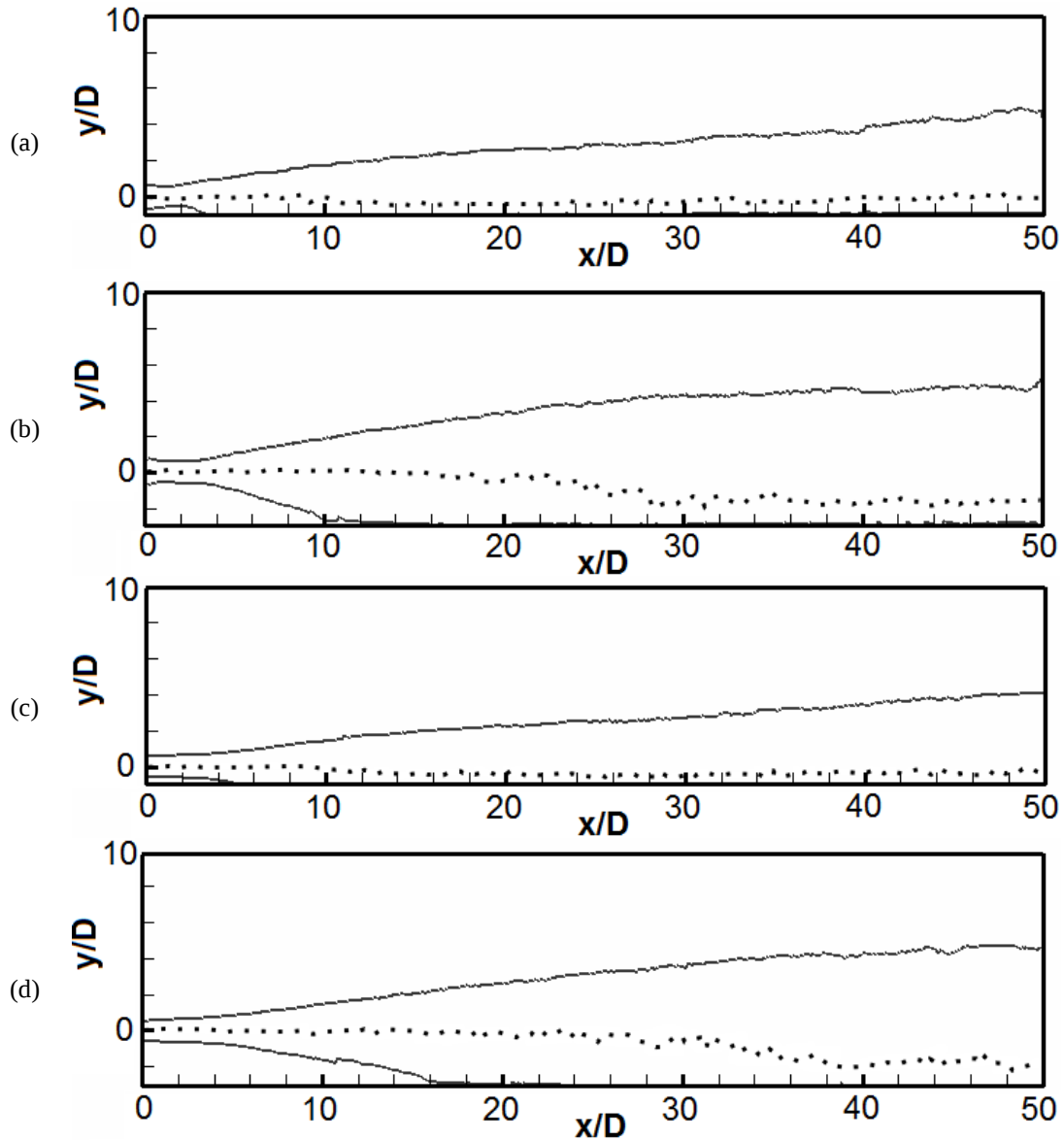
Figure 3.69 – Boundary contours for Fr = 250 located at (a) 1D, (b) 3D and Fr = 1000 located at (c) 1D and (d) 3D from the ground surface.
