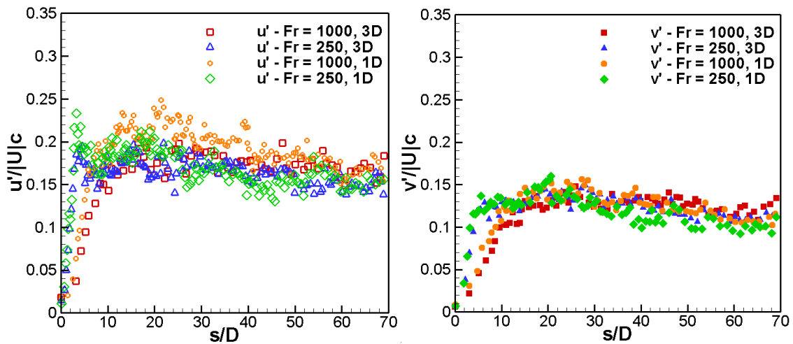
Figure 3.54 – Normalized velocity fluctuations along jet center line, jet near ground surface.
