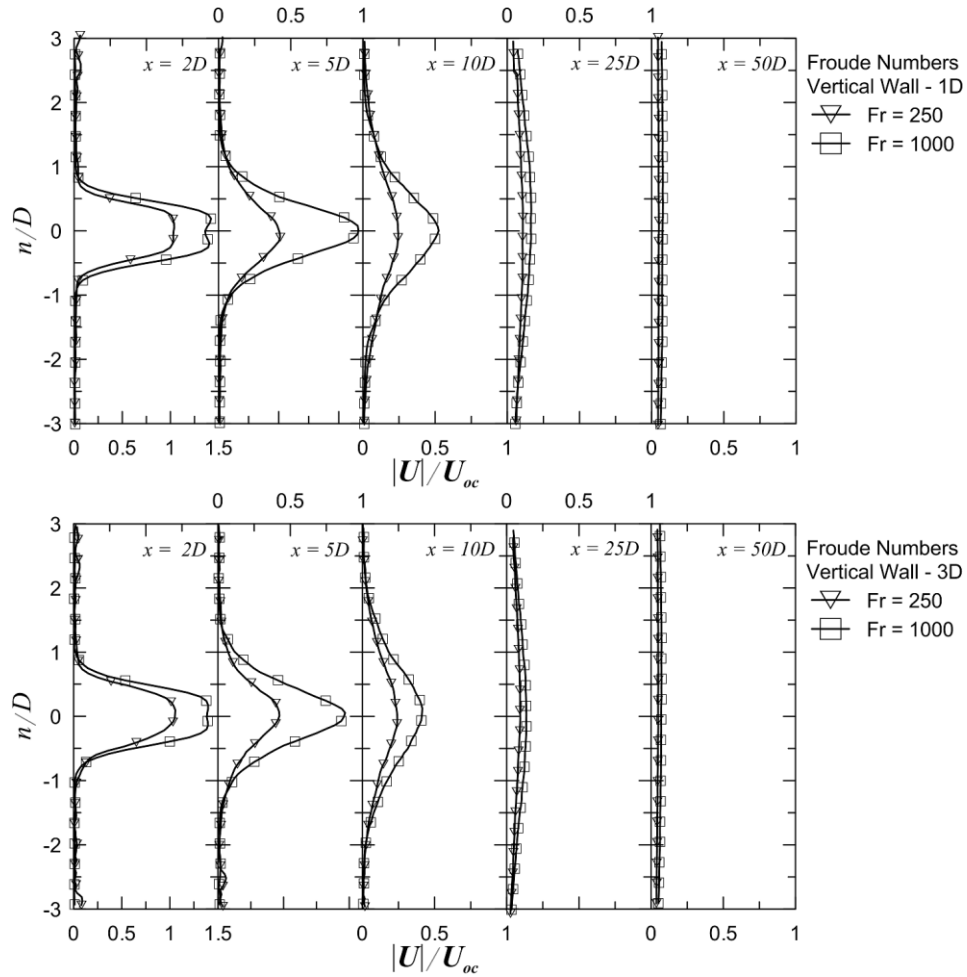
Figure 3.53 – Normalized velocity profiles for jets near the vertical wall surface with nozzle to surface distance of 1D (top) and 3D (bottom).
