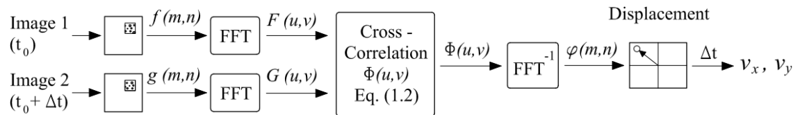
Figure 1.3 – PIV cross-correlation flowchart.
