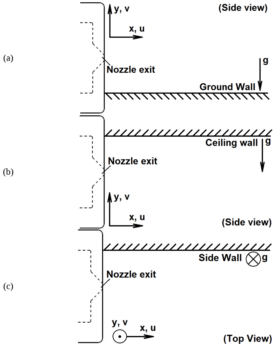
Figure 2.5 – Jet and surface orientation for wall effect cases, (a) ground, (b) ceiling and (c) vertical wall orientations
