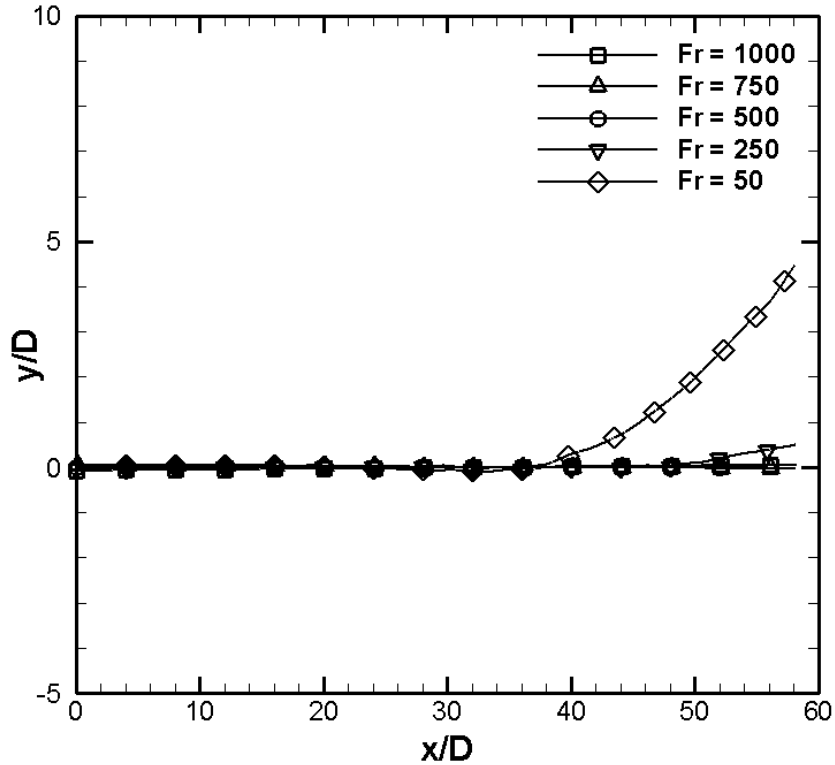
Figure 3.4 – Jet centerlines representations for free jet cases.
