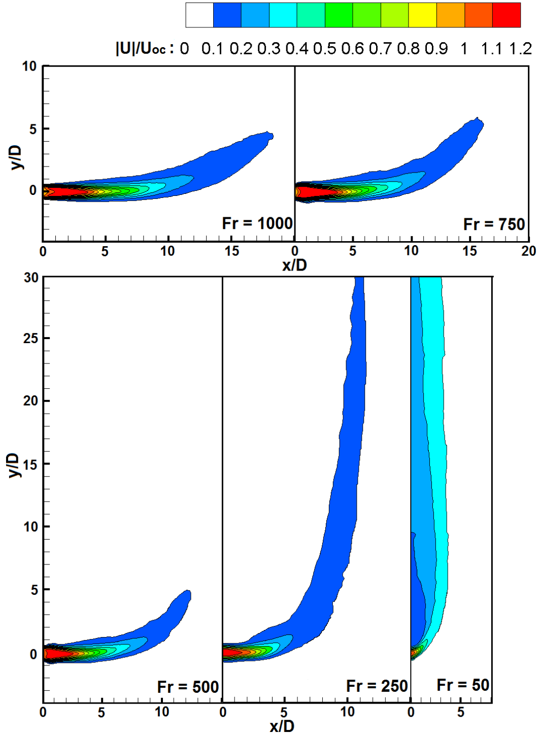
Figure 3.22 – Normalized time-averaged velocity magnitude ( |U|/U_{oc} ) for jet in crossflow.
