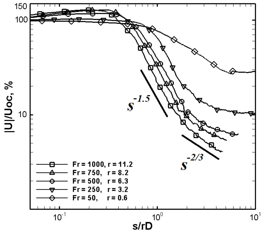
Figure 3.24 – Time-averaged velocity decay along jet centerline normalized by rD length scale
