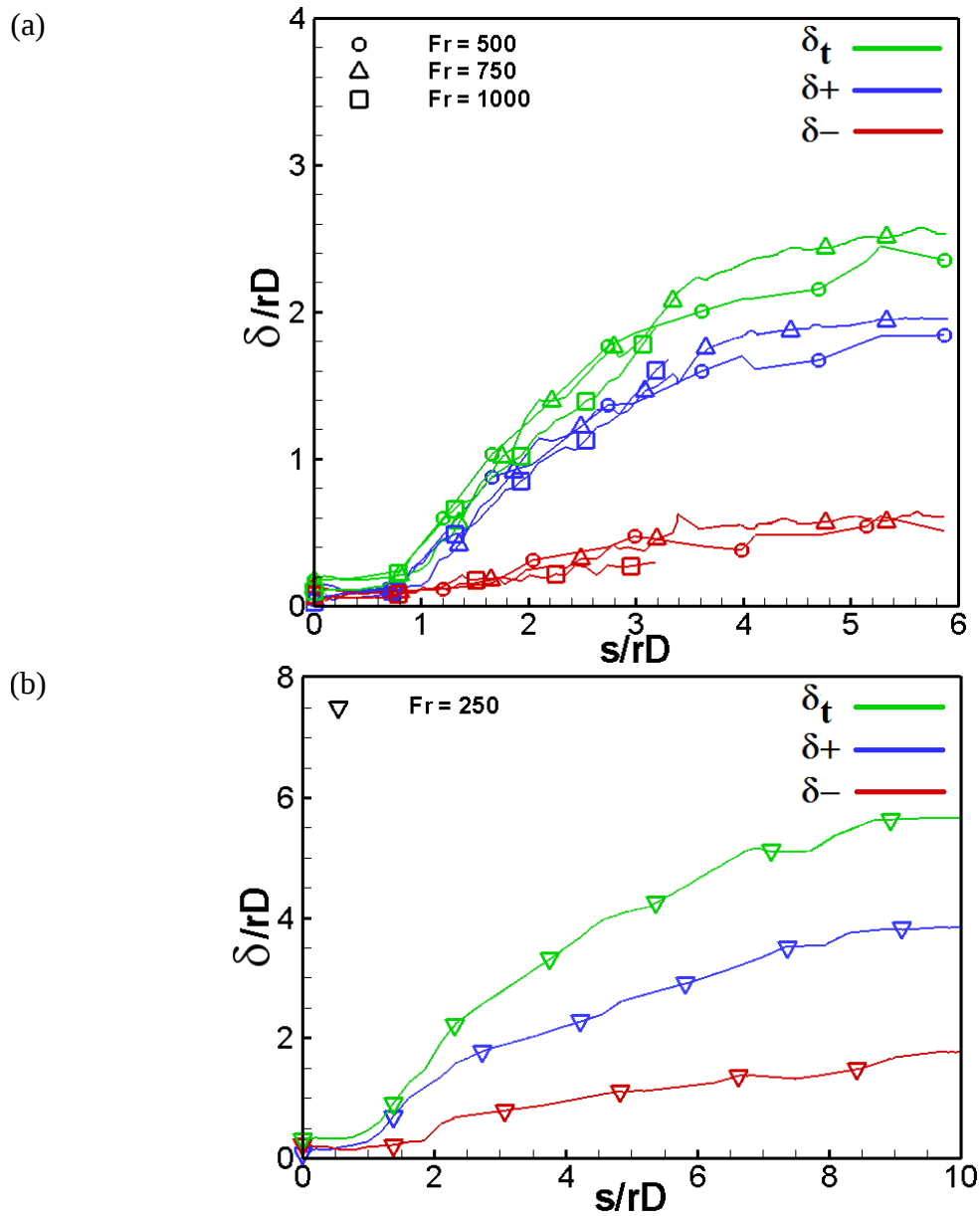
Figure 3.37 – Flow widths in jet centerplane for crossflowing jets, Fr = (a) 1000, 750 and 500, (b) 250.
