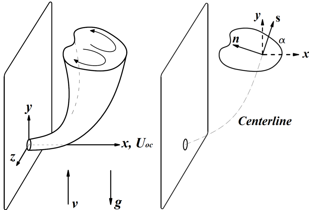
Figure 3.18 – Jet in crossflow (left), corresponding coordinate system (right).
