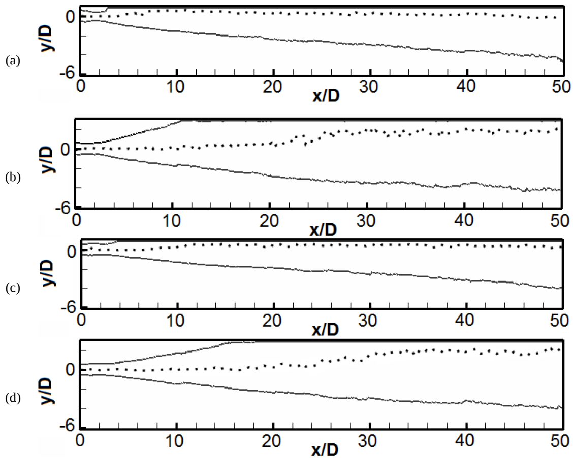
Figure 3.71 – Boundary contours for Fr = 250 located at (a) 1D, (b) 3D and Fr = 1000 located at (c) 1D and (d) 3D from the ceiling surface.
