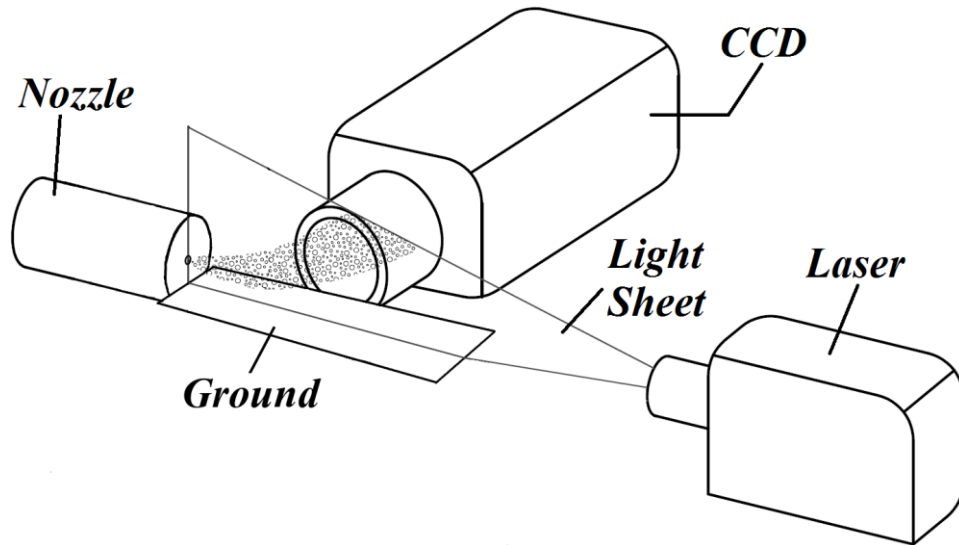
Figure 3.38 – Schematic of experimental setup for ground boundary.
