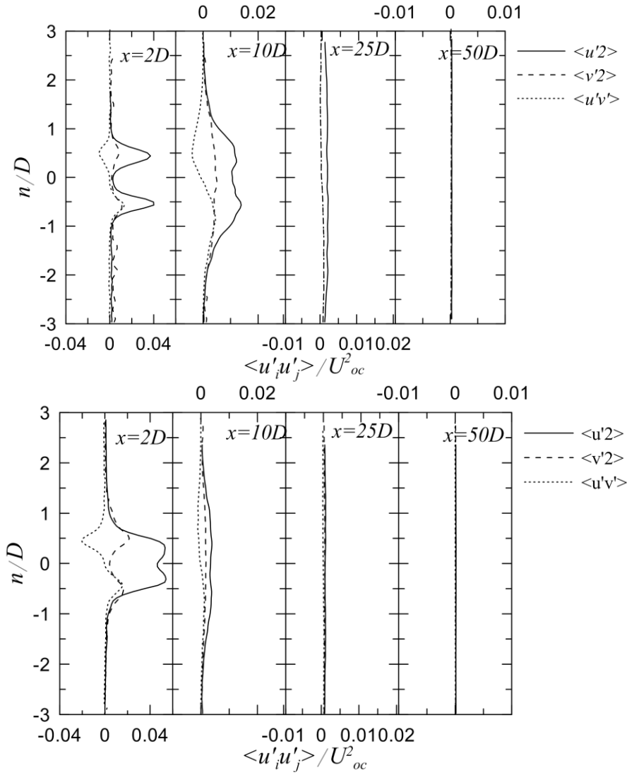
Figure 3.12 – Stress profiles in jet center-plane for free jet cases. (a) Fr = 1000 , (b) Fr = 250 .
