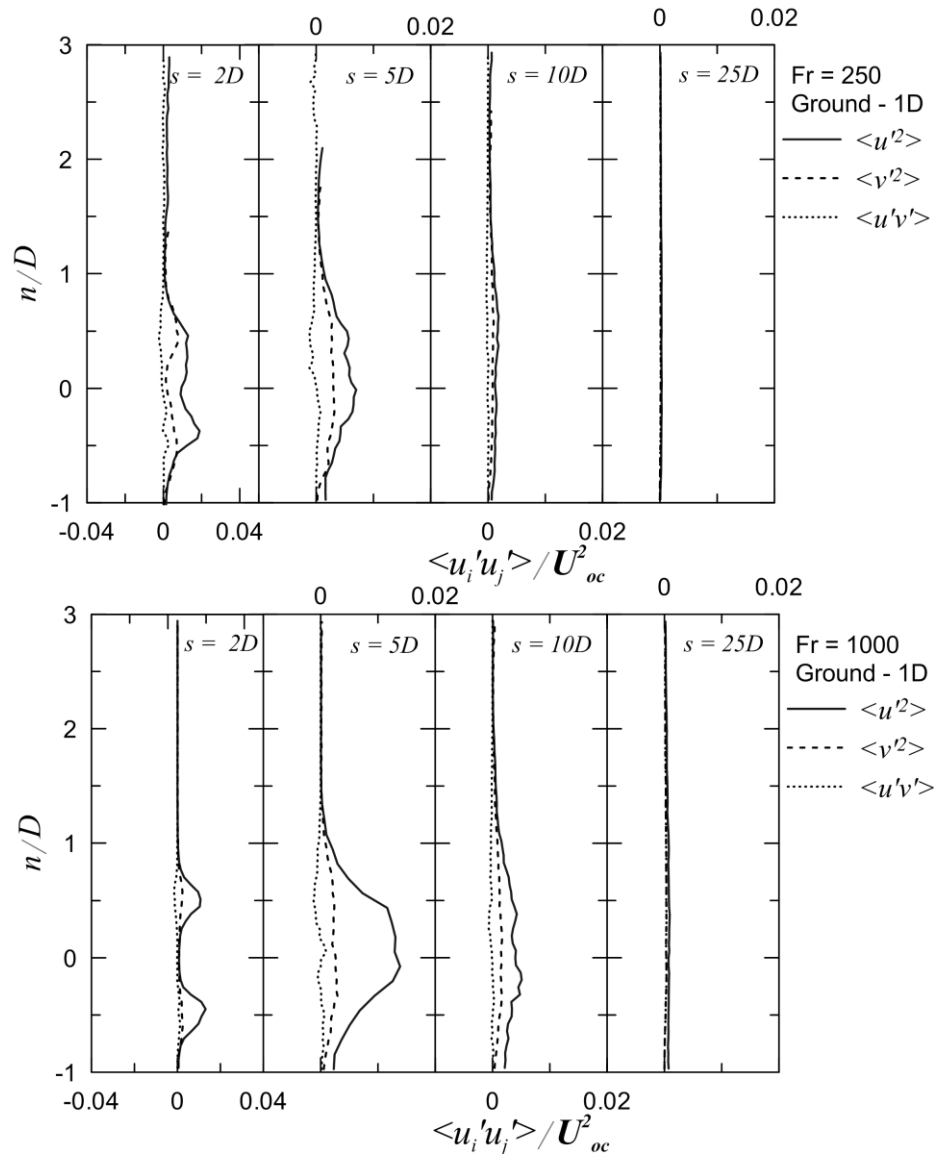
Figure 3.56 – Stress profiles in jet center-plane for jets located at 1D from ground surface (a) Fr = 250 , (b) Fr = 1000 .
