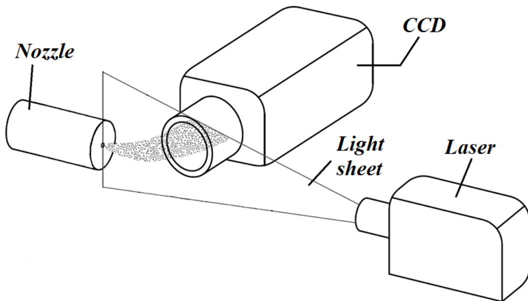
Figure 3.3 – Schematic of the experimental setup for free horizontal jet cases.
