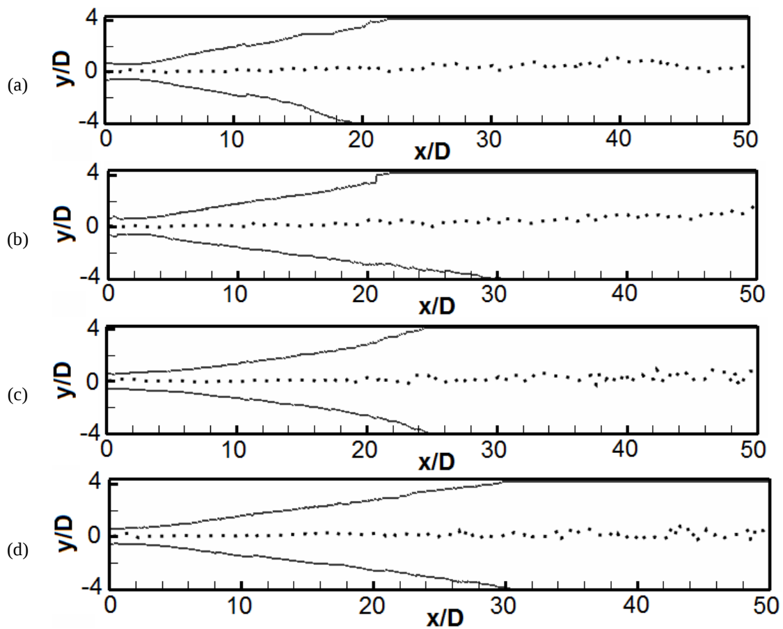
Figure 3.73 – Boundary contours for Fr = 250 located at (a) 1D , (b) 3D and Fr = 1000 located at (c) 1D and (d) 3D from the vertical wall surface.
