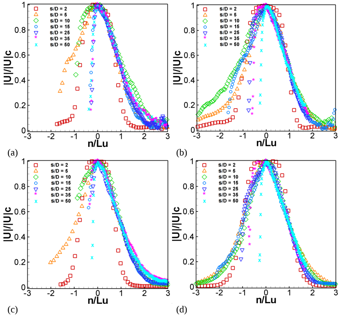
Figure 3.48 – Radial profiles of the time-averaged velocity, jet near ground surface, Fr = 250 located at (a) 1D, (b) 3D and Fr = 1000 located at (c) 1D and (d) 3D from the ground surface.
