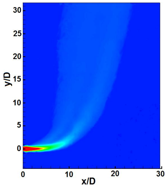
Figure 3.32 – Time-averaged velocity magnitude field, Fr = 500
