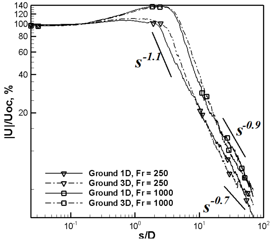
Figure 3.45 – Centerline velocity decay rates for ground boundary.
