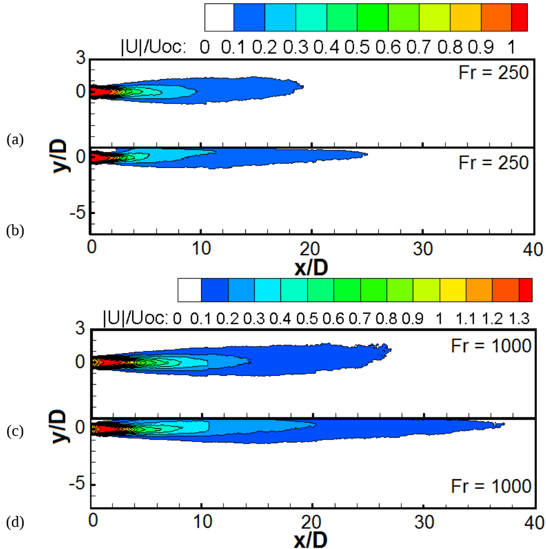
Figure 3.43 – Time-averaged velocity fields (a) Fr = 250 at 3D , (b) Fr = 250 at 1D , (c) Fr = 1000 at 3D and (d) Fr = 1000 at 1D distance from the ceiling surface.
