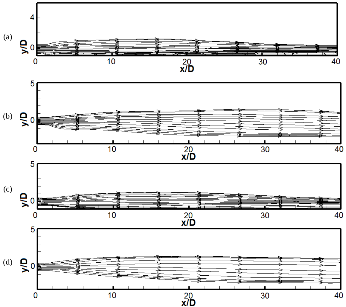
Figure 3.64 – Flow streamlines for Fr = 250 with nozzle to surface distance of (a) 1D , (b) 3D and Fr = 1000 with nozzle to surface distance of (c) 1D and (d) 3D - Jet near ground surface.
