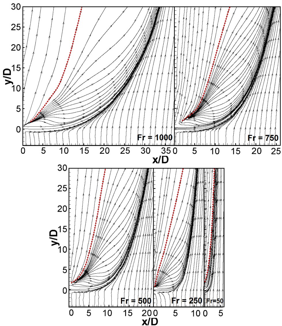
Figure 3.34 – Flow streamlines of jet center-plane determined from the time-averaged velocity field
