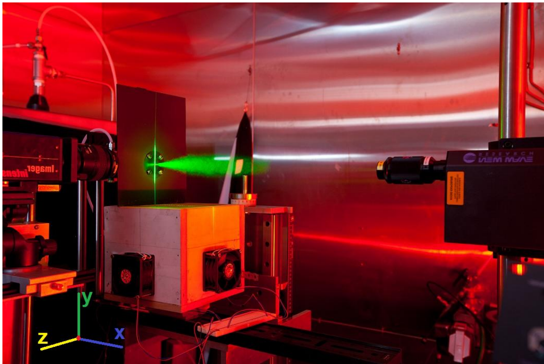
Figure 2.4 – Experimental apparatus
