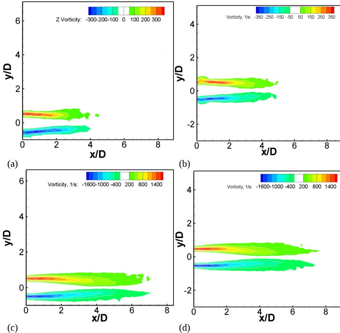
Figure 3.63 – Time-averaged out-of-plane vorticity contours for Fr = 250 located at (a) 1D, (b) 3D and Fr = 1000 located at (c) 1D and (d) 3D from the ground surface.
