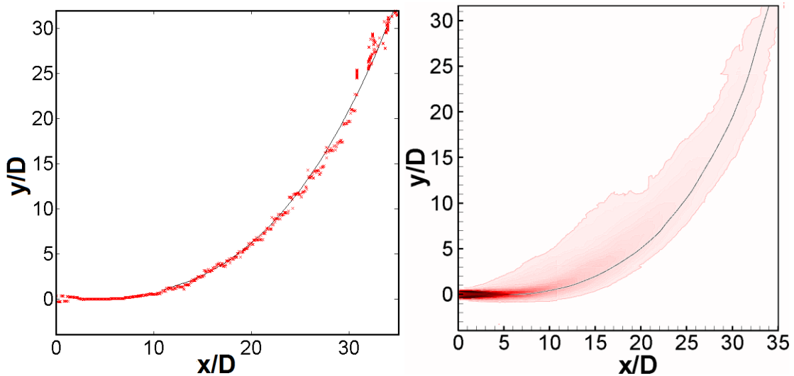
Figure 3.2 – Local maxima in the normalized time-averaged velocity field (left); jet centerline (right)
