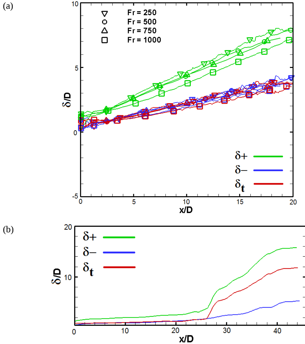
Figure 3.16 – Flow width, Fr = (a) 250, 500, 750 and 1000, and (b) 50.
