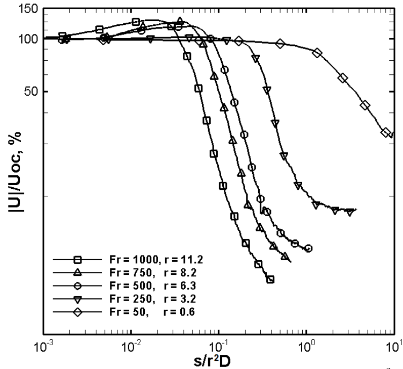
Figure 3.25 – Centerline time-averaged velocity magnitude decay normalized by r^2D length scale
