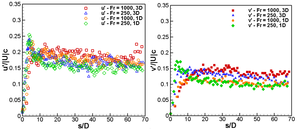
Figure 3.57 – Normalized velocity fluctuations along jet center line, jet near ceiling surface.
