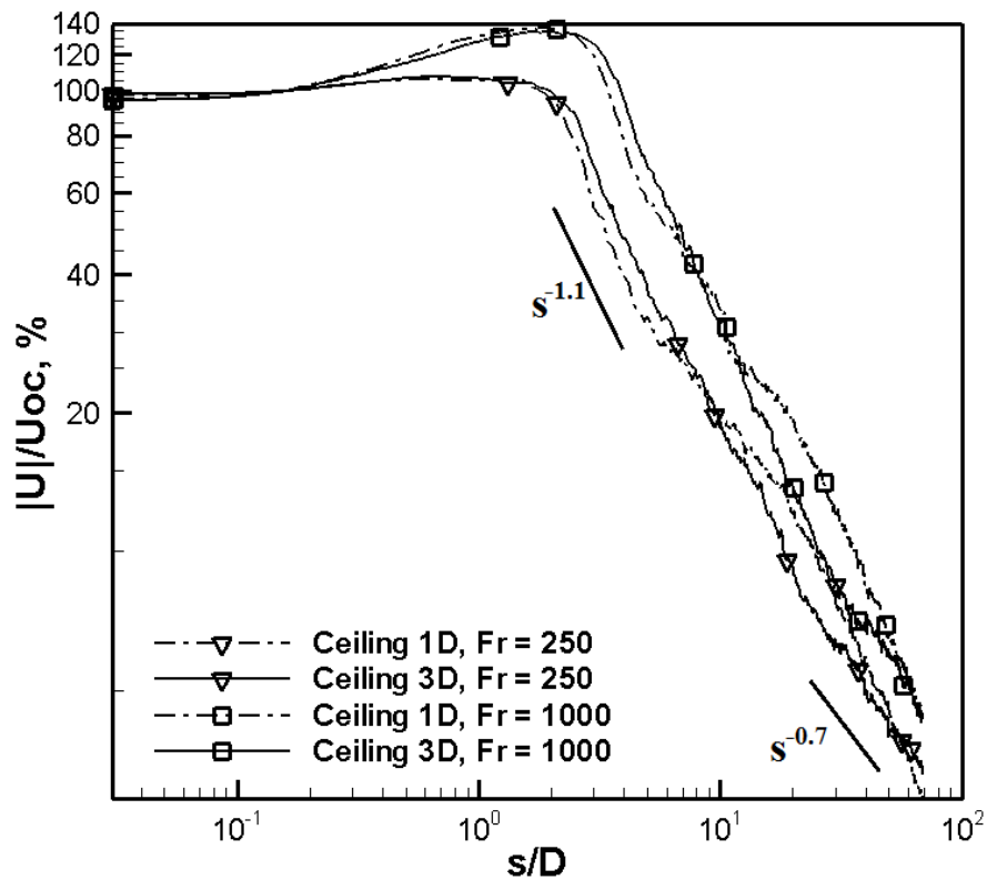
Figure 3.46 – Centerline velocity decay rates for ceiling boundary.
