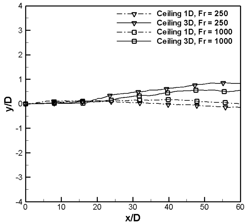
Figure 3.40 – Jet centerline representation for ceiling boundary normalized by D .
