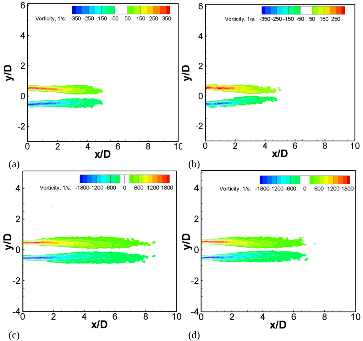
Figure 3.67 – Time-averaged out-of-plane vorticity contours for Fr = 250 located at (a) 1D, (b) 3D and Fr = 1000 located at (c) 1D and (d) 3D from the vertical wall surface.
