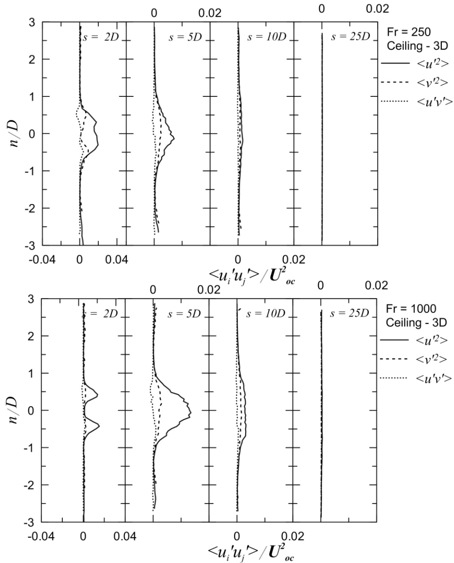
Figure 3.58 – Stress profiles in jet center-plane for jets located at 3D from ceiling surface (a) Fr = 250 , (b) Fr = 1000 .
