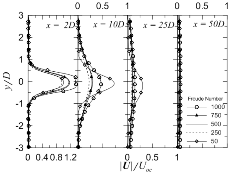
Figure 3.10 – Time-averaged normalized velocity magnitude profiles of the free jet cases.
