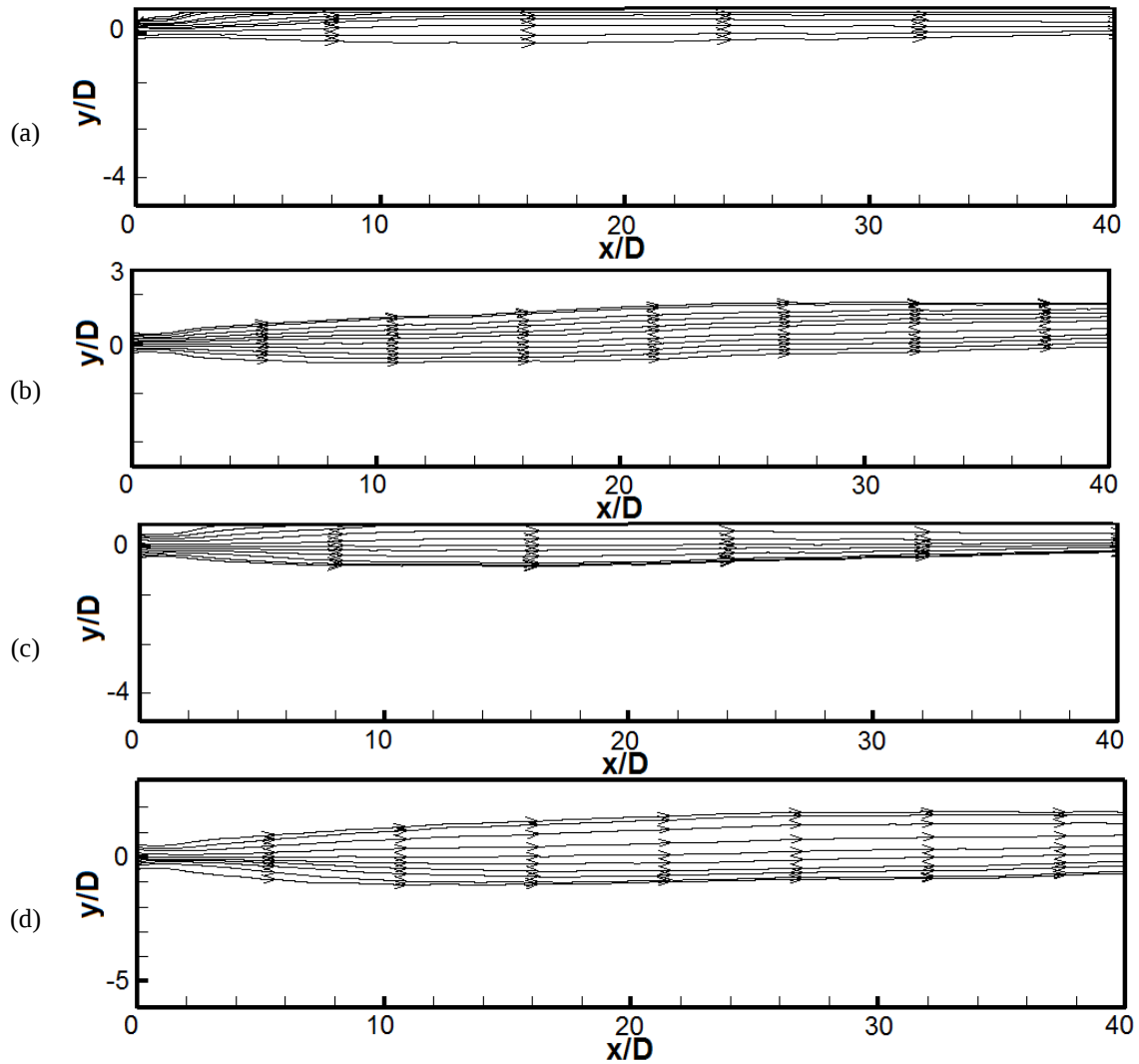
Figure 3.66 – Flow streamlines for Fr = 250 located at (a) 1D , (b) 3D and Fr = 1000 located at (c) 1D and (d) 3D from the ceiling surface.
