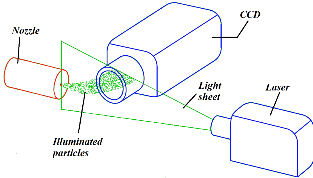
Figure 2.6 – Schematics of the PIV setup
