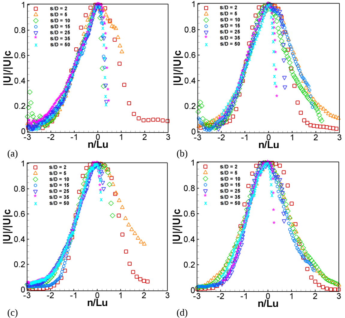
Figure 3.50 – Radial profiles of the time-averaged velocity, jet near ceiling surface, Fr = 250 located at (a) 1D, (b) 3D and Fr = 1000 located at (c) 1D and (d) 3D from the ceiling surface.
