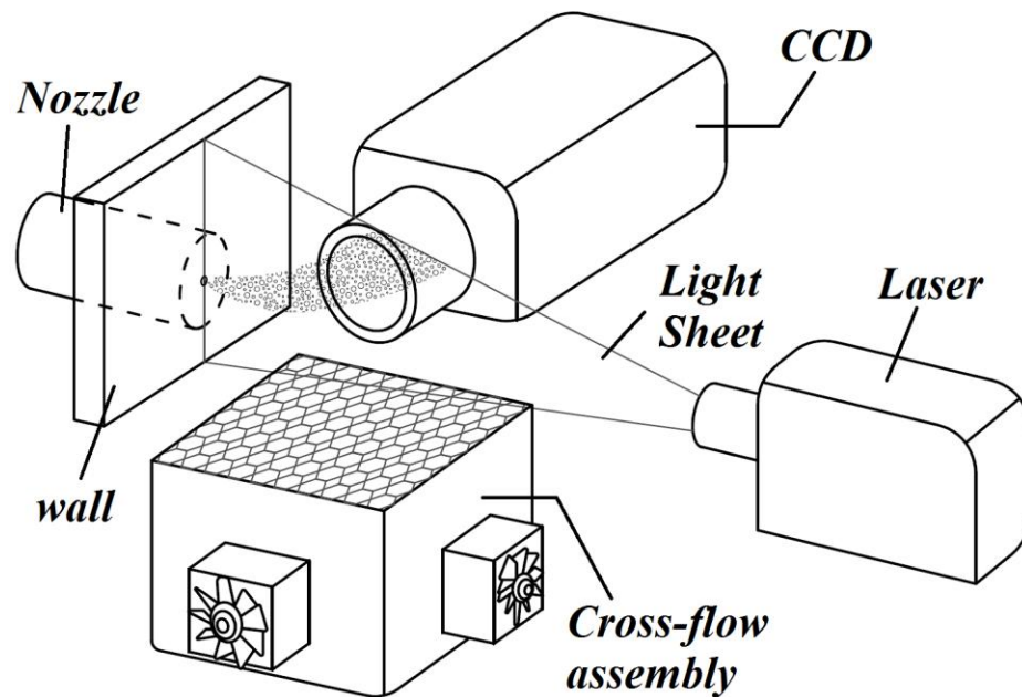
Figure 3.17 – Schematics of the experimental setup for jet in crossflow cases.
