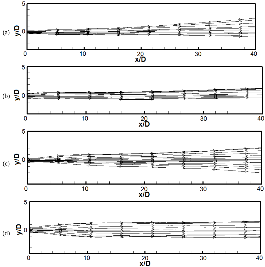
Figure 3.68 – Flow streamlines for Fr = 250 located at (a) 1D , (b) 3D and Fr = 1000 located at (c) 1D and (d) 3D from the vertical wall surface.
