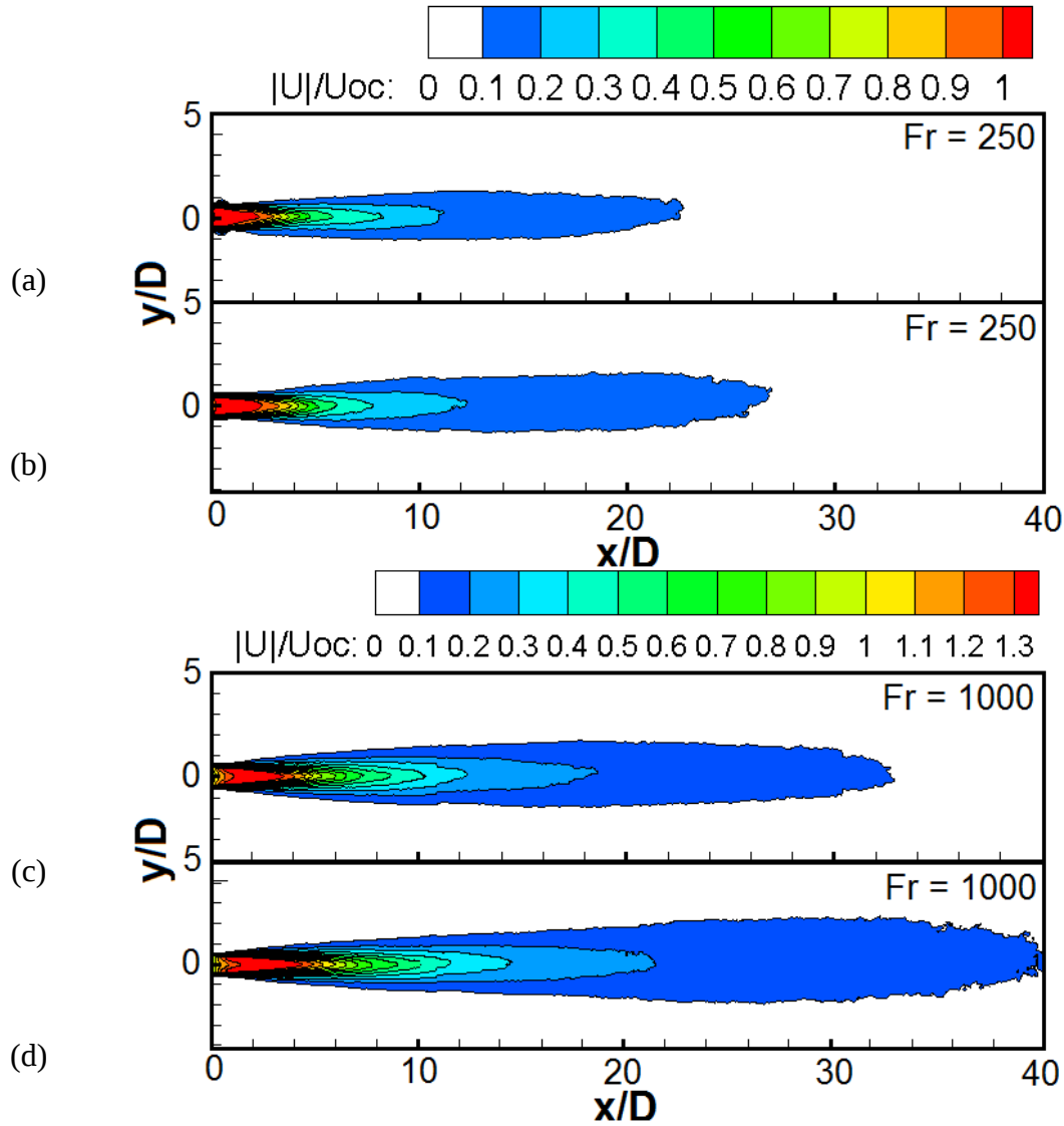
Figure 3.44 – Time-averaged velocity fields (a) Fr = 250 at 3D , (b) Fr = 250 at 1D , (c) Fr = 1000 at 3D and (d) Fr = 1000 at 1D distance from the vertical wall.
