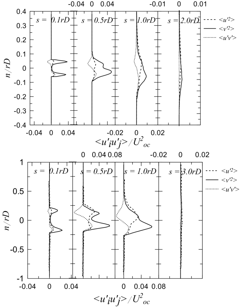
Figure 3.29 – Stress profiles in jet center-plane for jet in crossflow cases. (a) Fr = 1000 , (b) Fr = 250 .
