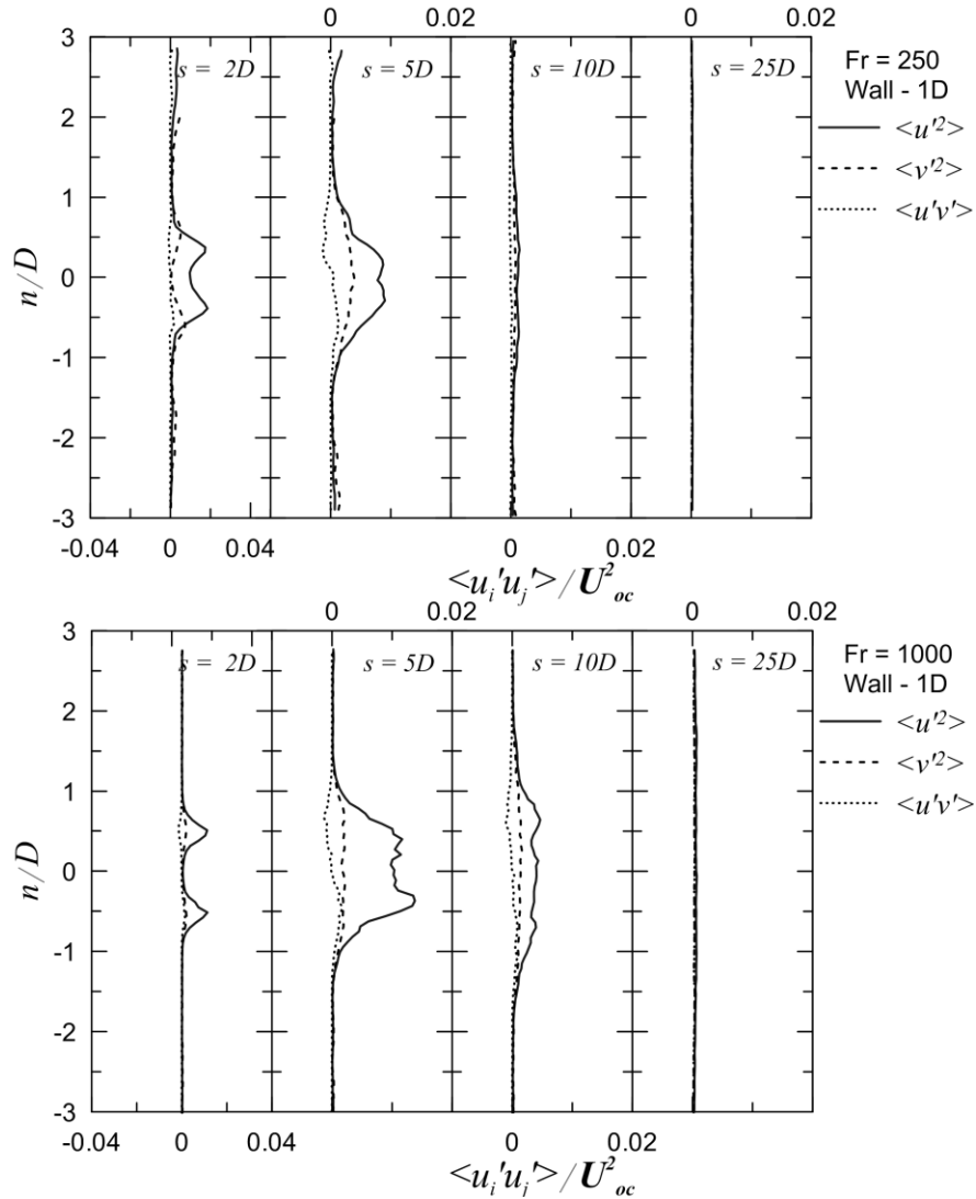
Figure 3.62 – Stress profiles in jet center-plane for jets located at 1D from vertical wall surface for Fr = 250 (top) and Fr = 1000 (bottom).
