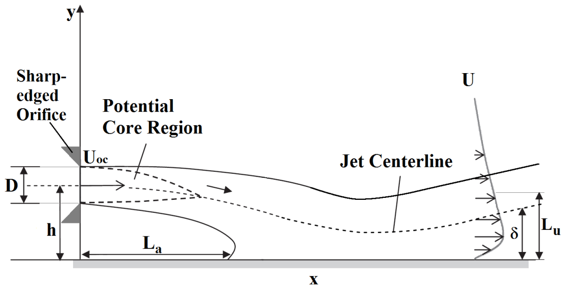
Figure 1.1 – Schematics of the wall jet flow.
