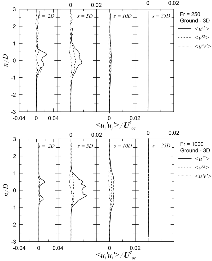
Figure 3.55 – Stress profiles in jet center-plane for jets located at 3D from ground surface (a) Fr = 250 , (b) Fr = 1000 .
