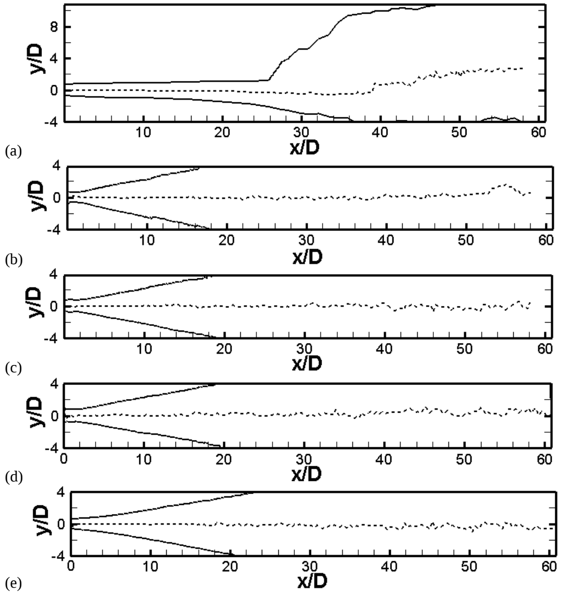
Figure 3.15 – Free jet boundary contours, Fr = (a) 50, (b) 250, (c) 500, (d) 750 and (e) 1000.
