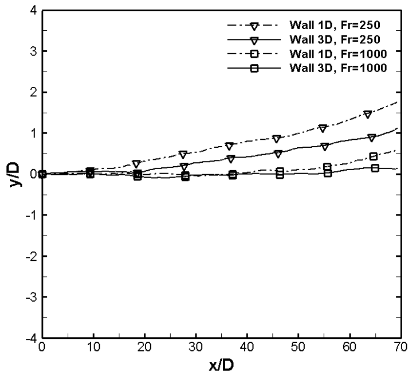
Figure 3.41 – Jet centerline representation for vertical wall boundary normalized by D .
