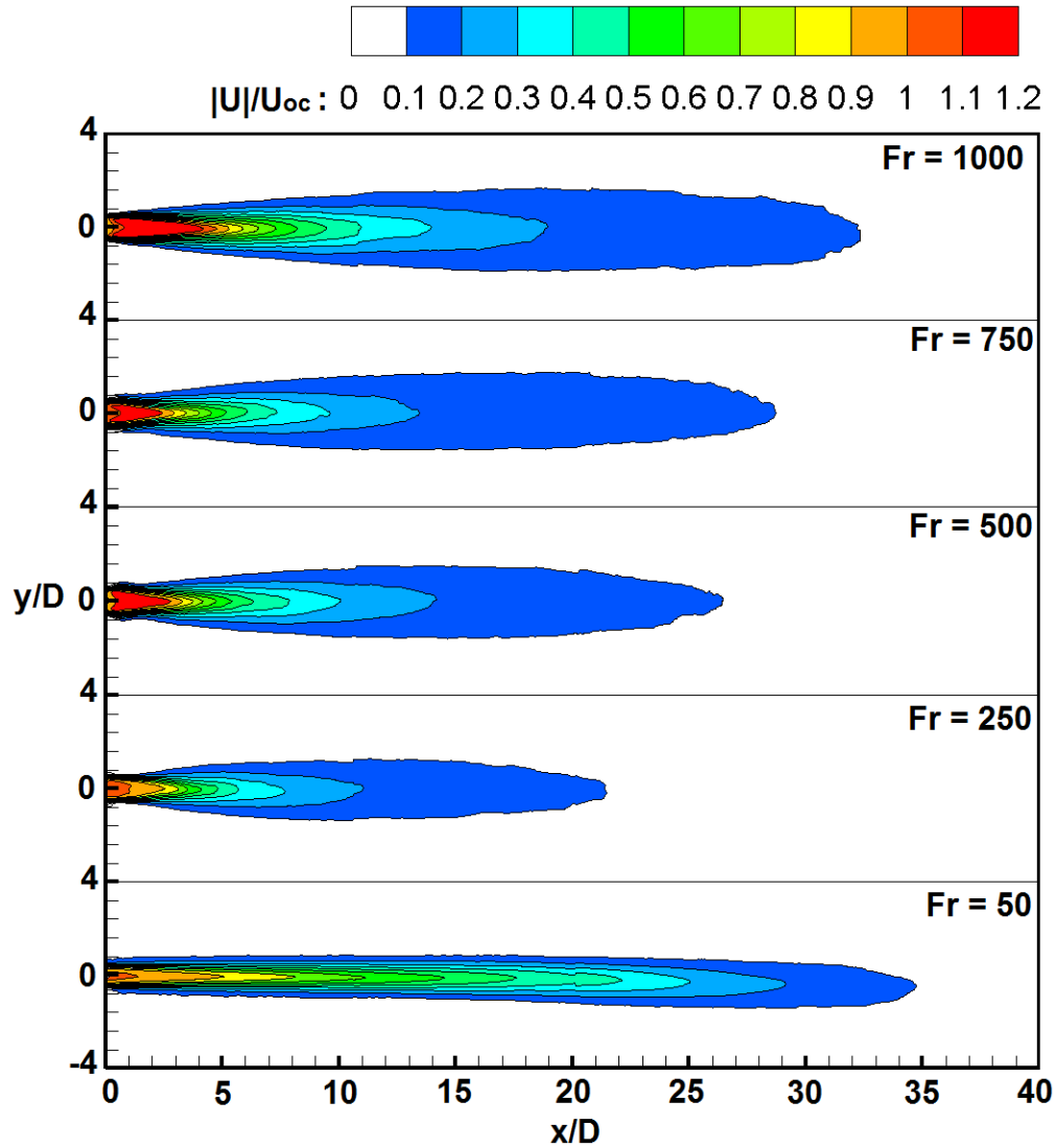
Figure 3.5 – Normalized time-averaged velocity magnitude ( |U|/U_{oc} ) contours between x/D = 0 - 40 .
