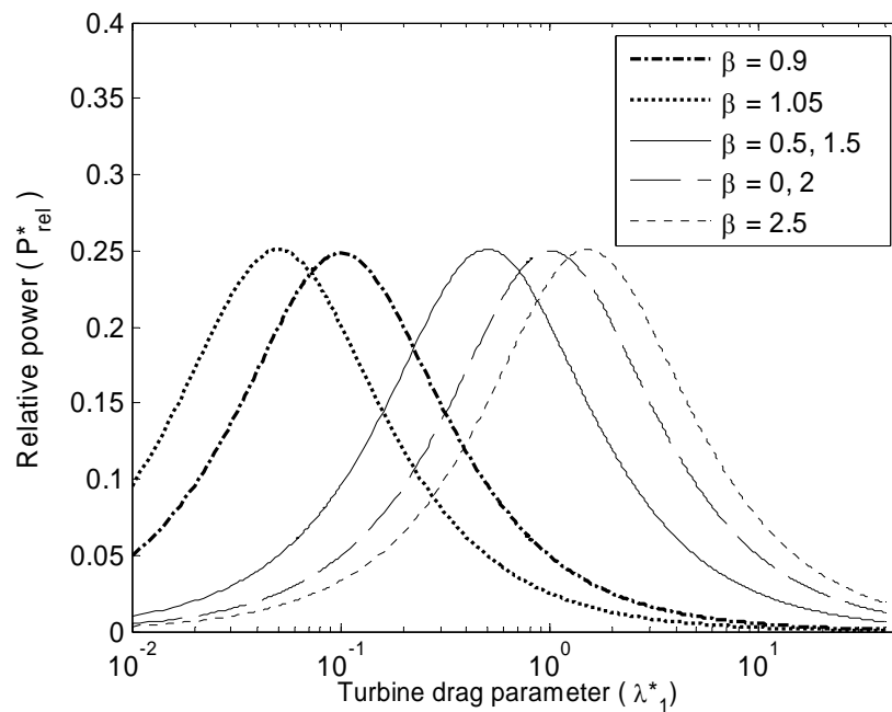
Figure 3.3: Relative power as a function of the turbine drag parameter for varying bay geometries when friction is assumed linearly proportional with the flow rate and losses are negligible.
