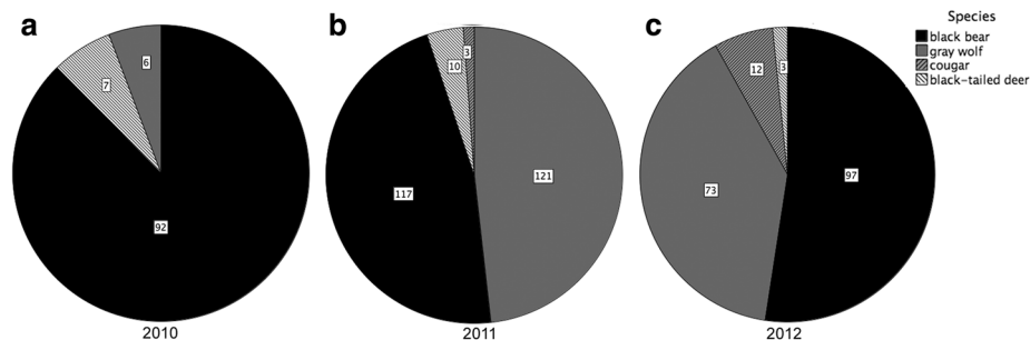
Figure 2 Summary of camera-trapped large mammals in supratidal and intertidal zones in a 2010, b 2011 and c 2012. Cameras (2010, n = 7,422 camera days; 2011, n = 11,545 camera days; 2012, n = 11,500 camera days) were located on beaches in Quatsino Sound, British Columbia, Canada. Counts for large mammals reflect independent camera detections on a 30-min basis (see "Methods").
