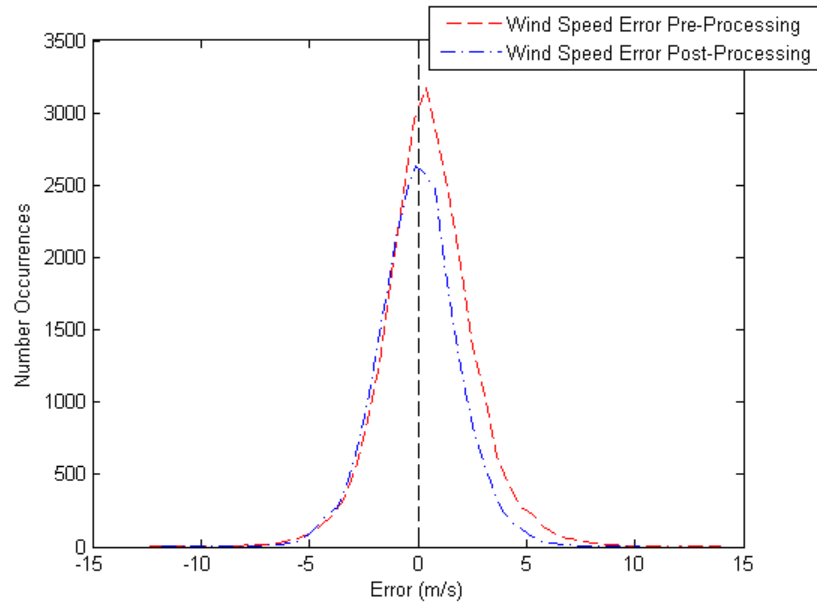
Figure E.2: Day-Ahead Wind Speed Forecast Error Distribution
