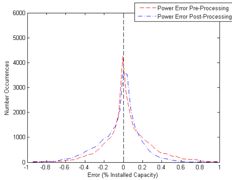
Figure E.8: Three Day-Ahead Wind Power Forecast Error Distribution
