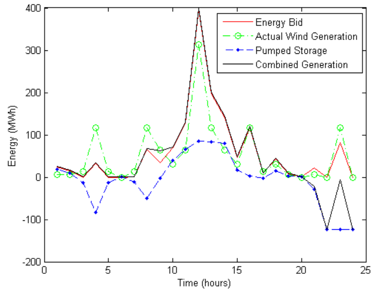
Figure D.8: Sample Day 5 Operation - Reliability Case
