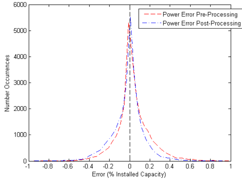
Figure E.5: Day-Out Wind Power Forecast Error Distribution
