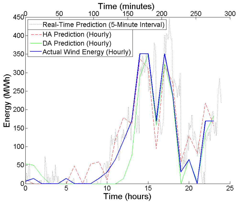
Figure 2.3: 24-hour Wind Forecast Time Series showing Real-Time, Hour-Ahead (HA), and Day-Ahead (DA), Forecasts in comparison to Actual Output
