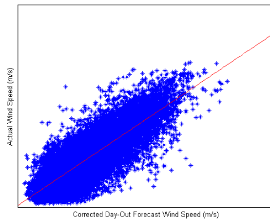
Figure E.10: Actual vs. Day-Out Wind Speed Forecast Post-Processing
