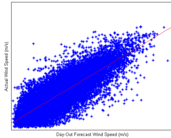
Figure E.9: Actual vs. Day-Out Wind Speed Forecast Pre-Processing
