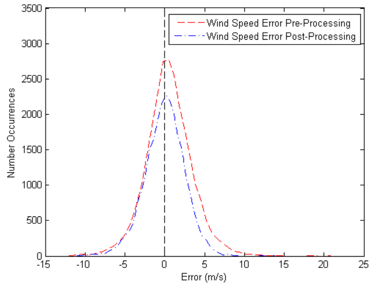
Figure E.4: Three Day-Ahead Wind Speed Forecast Error Distribution
