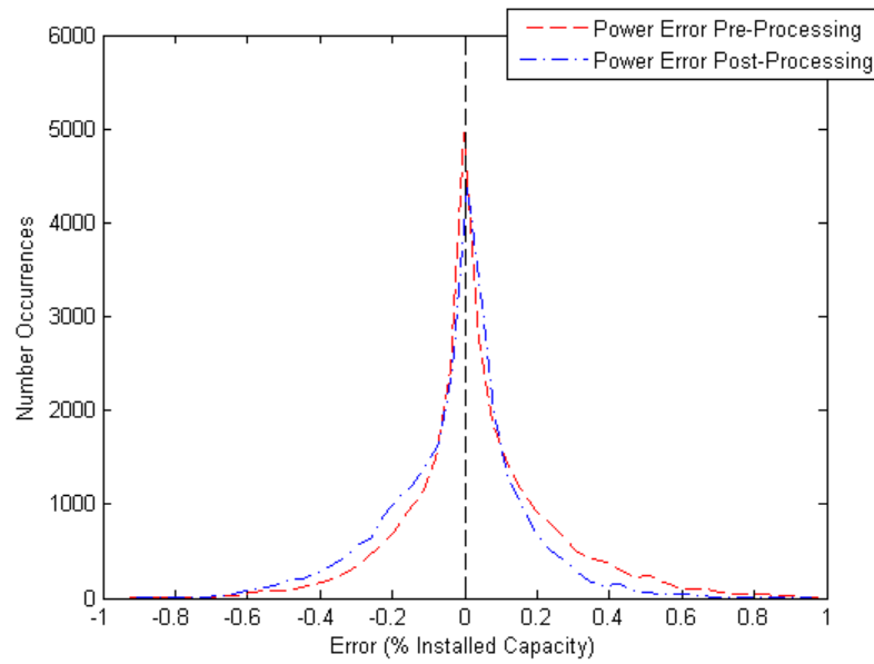
Figure E.7: Two Day-Ahead Wind Power Forecast Error Distribution
