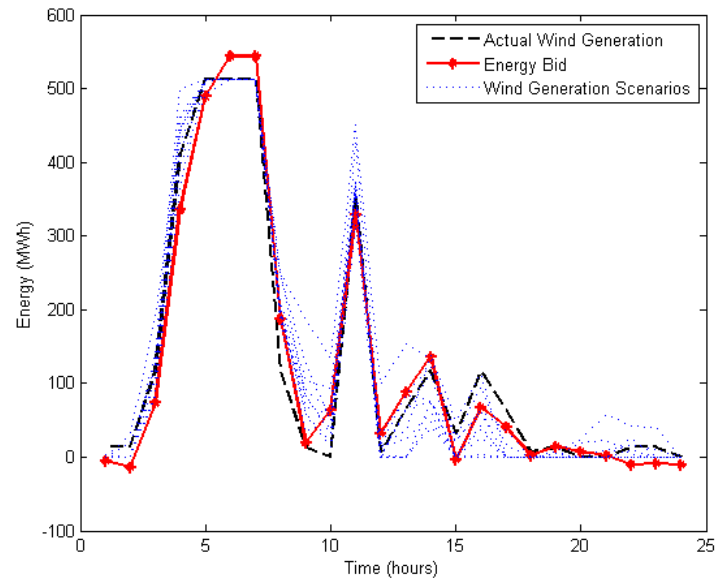
Figure D.4: Scenario Plot - Reliability Case
