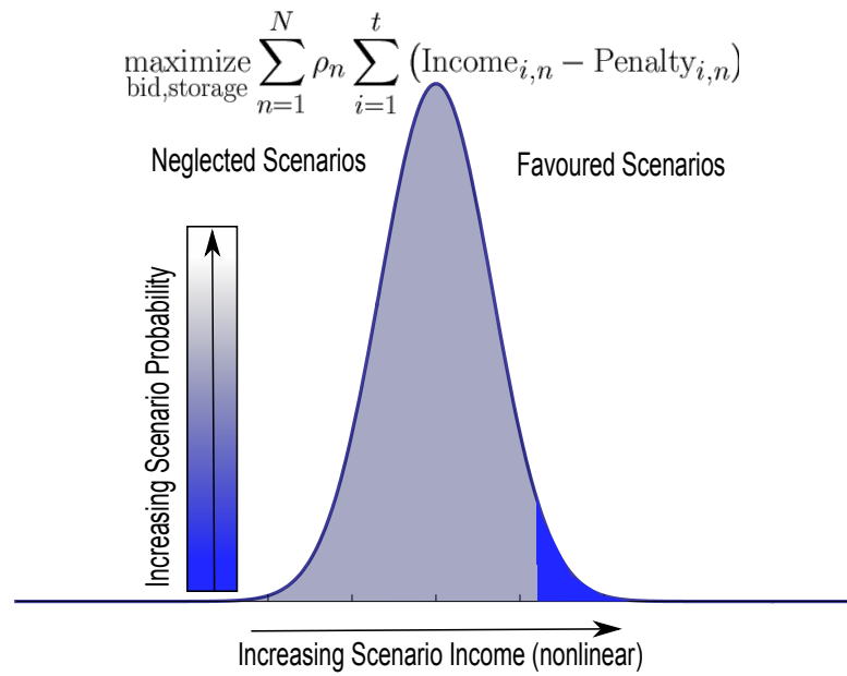
Figure 3.3: Scenario Preference Schematic - Basic Stochastic Case
