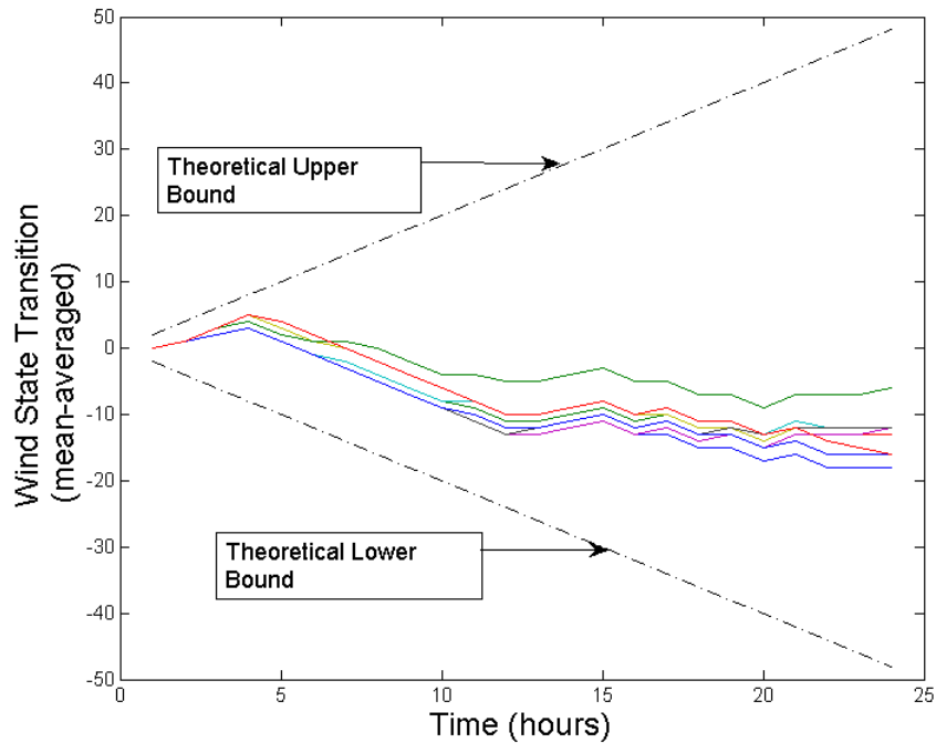
Figure 2.8: Reduced Scenario Tree – Sampling size of 1000 Scenarios Reduced to 10 Scenarios
