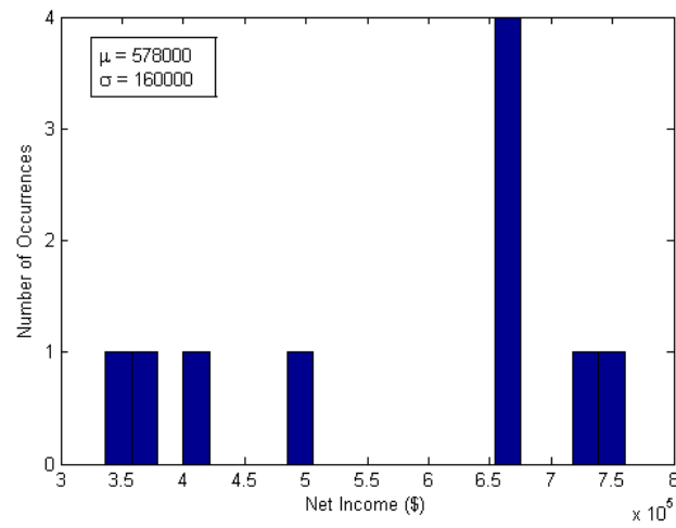
Figure 3.6: Daily Income Histogram – Robust-Reliable Case - Standard Deviation Term in Objective Function
