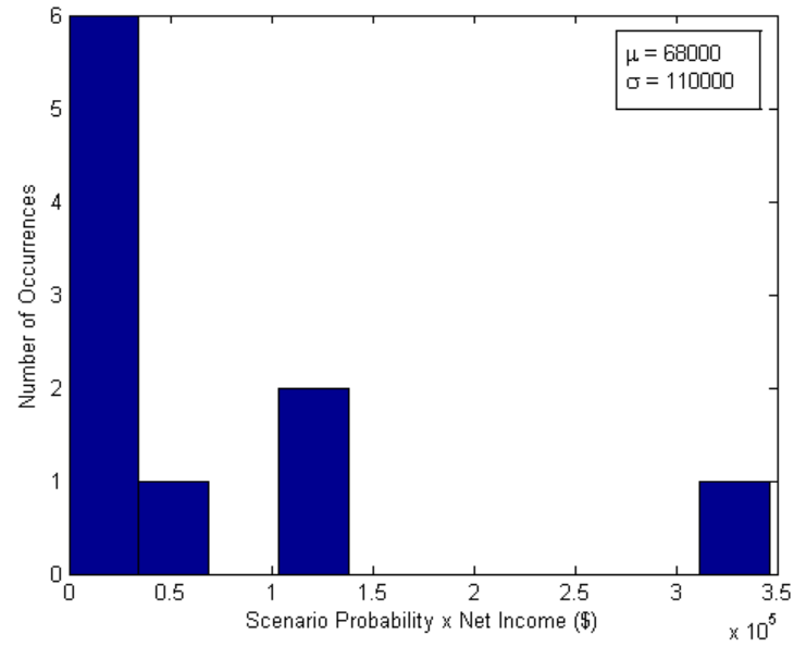
Figure D.9: Probability-Income Product Histogram – Robust Problem
