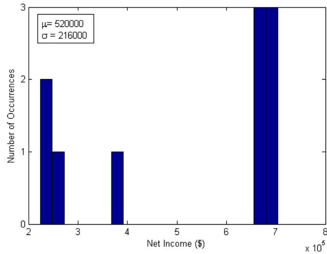
Figure 3.2: Daily Income over a Set of 10 Scenarios - Single Optimal Generating Schedule Applied to all Scenarios
