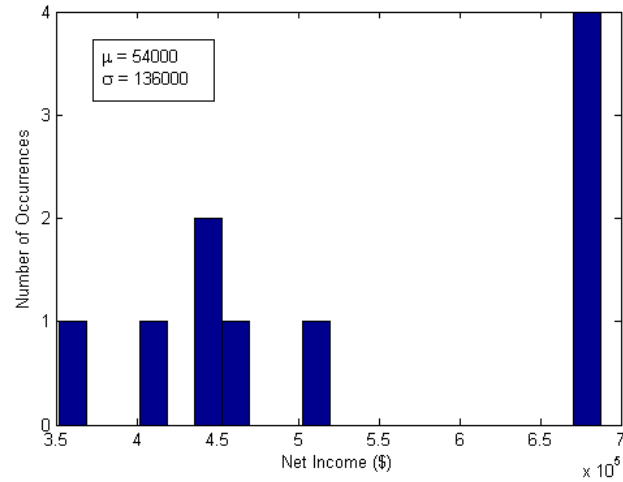
Figure 3.5: Daily Income Histogram – Reliability Case
