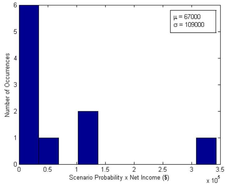
Figure D.10: Probability-Income Product Histogram – Robust-Reliable Problem ( \sigma )
