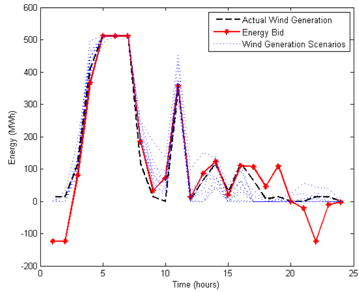
Figure D.3: Scenario Plot - Robust-Reliable Case
