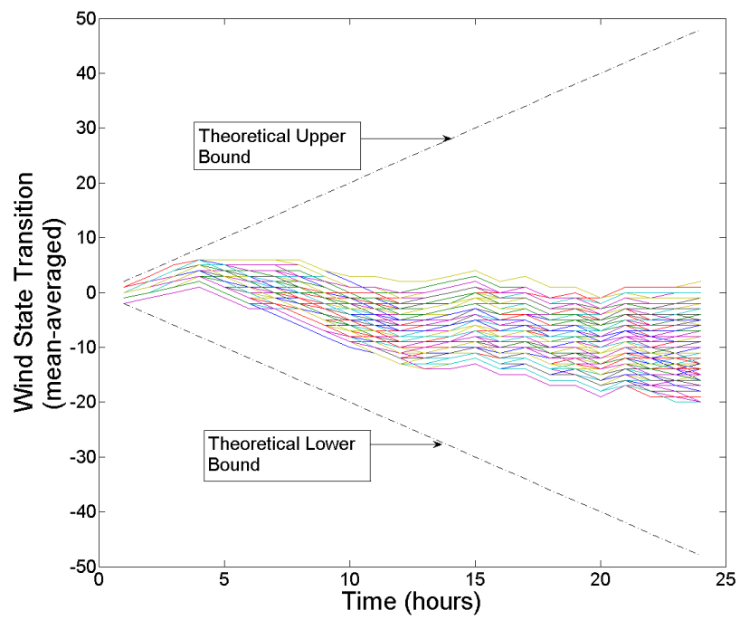
Figure 2.5: Forecast Error Generator Scenario Tree – Sampling size of 1000 Scenarios
