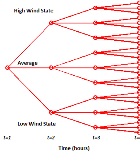
Figure 2.4: Dense Scenario Tree – Simplified Qualitative Example
