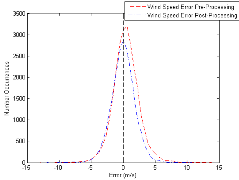
Figure E.1: Day-Out Wind Speed Forecast Error Distribution
