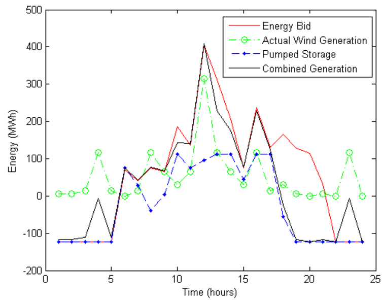
Figure D.6: Sample Day 5 Operation - Robust Case
