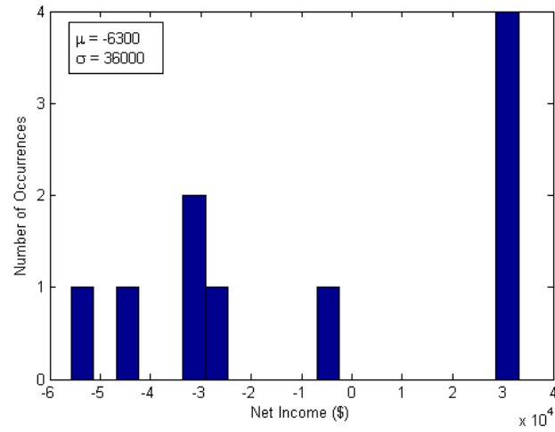
Figure 3.7: Daily Income Histogram - Robust-Reliable Case - Variance Term in Objective Function
