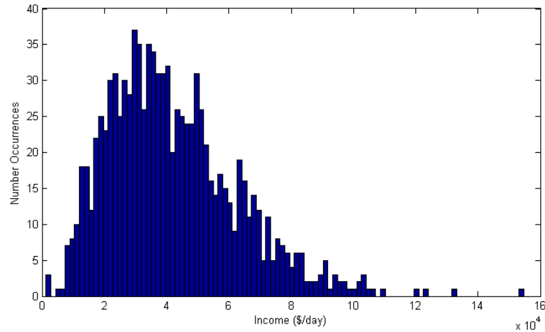
Figure 3.1: Daily Income over a Set of 1000 Scenarios - Optimal Generating Schedule for Each Scenario
