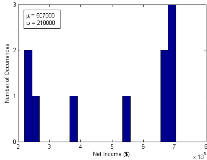
Figure 3.4: Daily Income Histogram - Robust Case
