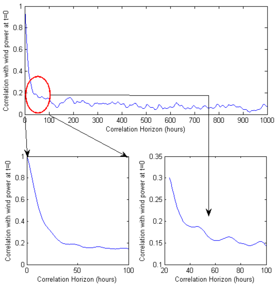
Figure 2.7: Sample Wind Power Correlation with Time Horizon
