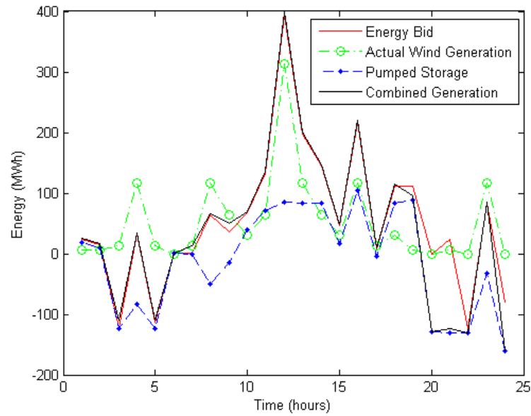
Figure D.7: Sample Day 5 Operation - Robust-Reliable Case
