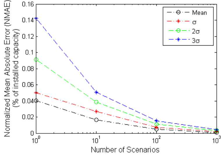
Figure 2.6: Wind Forecast Distribution Moments Convergence
