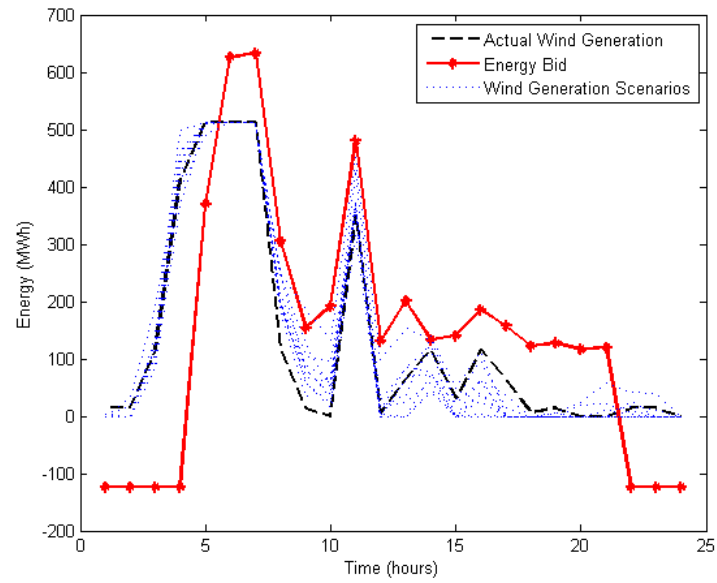
Figure D.2: Scenario Plot - Robust Case
