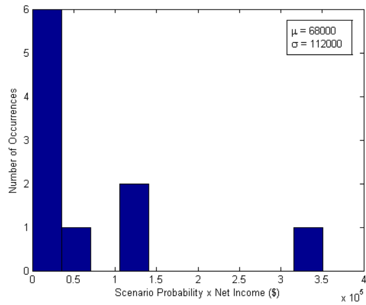
Figure D.12: Probability-Income Product Histogram – Reliable Problem
