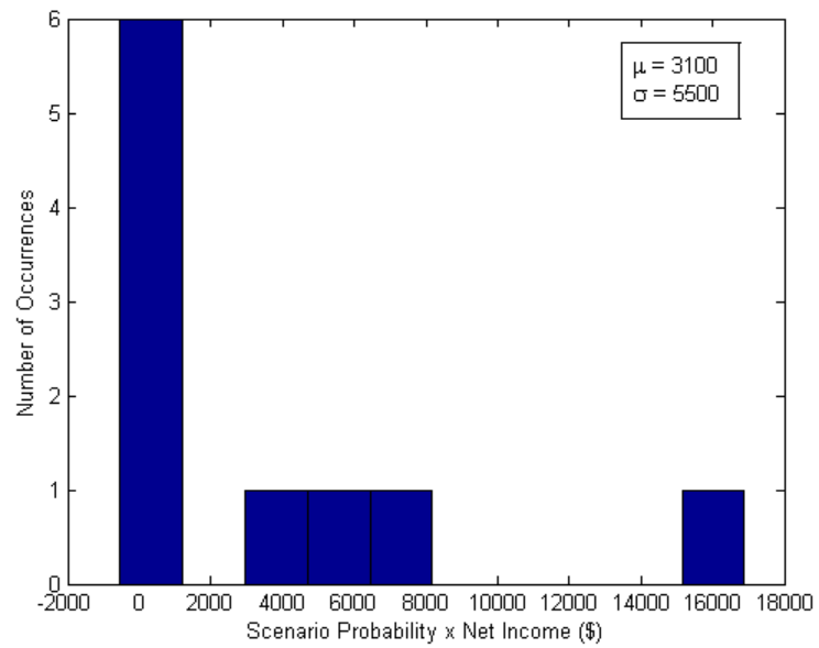
Figure D.11: Probability-Income Product Histogram – Robust-Reliable Problem ( \sigma^2 )
