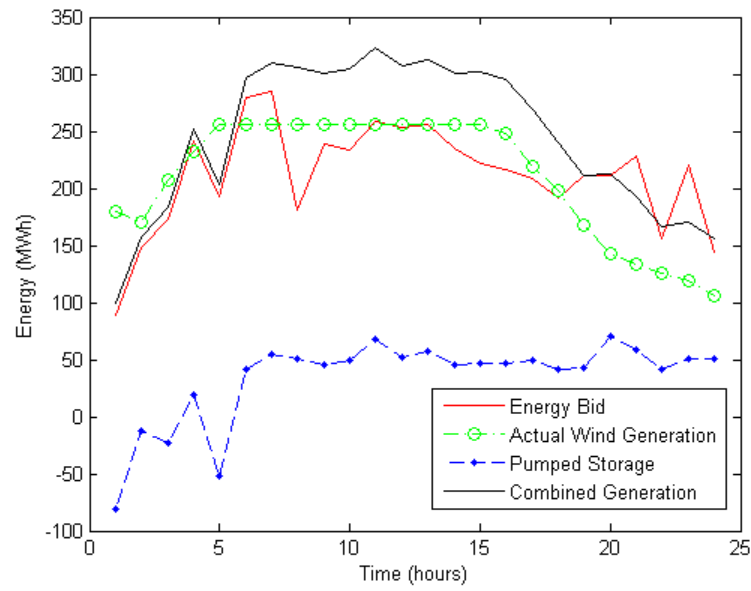
Figure 4.7: Case Study Facility Operation – Day 7
