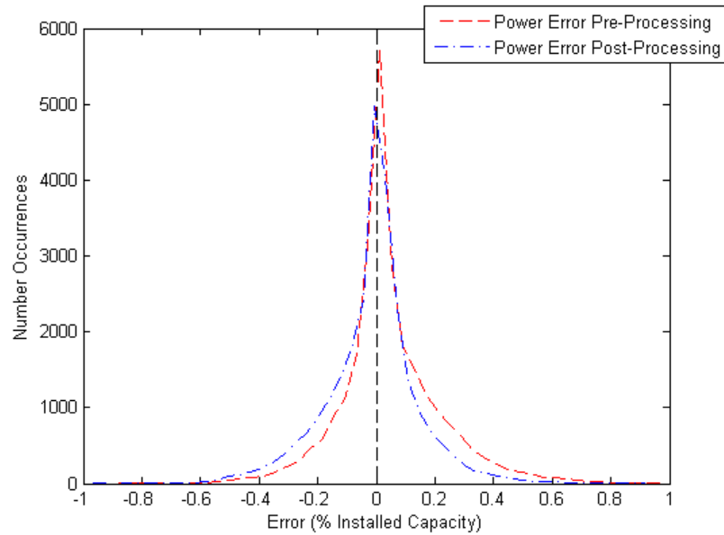
Figure E.6: Day-Ahead Wind Power Forecast Error Distribution
