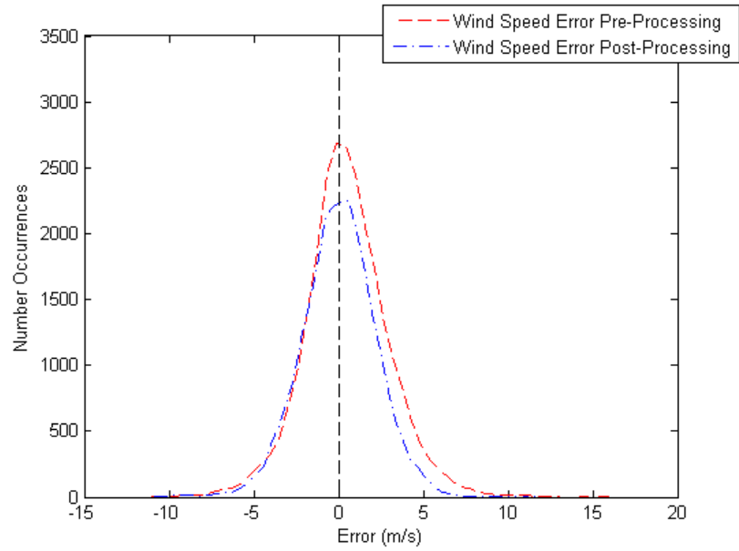
Figure E.3: Two Day-Ahead Wind Speed Forecast Error Distribution
