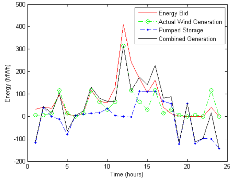
Figure D.5: Sample Day 5 Operation - Deterministic Case
