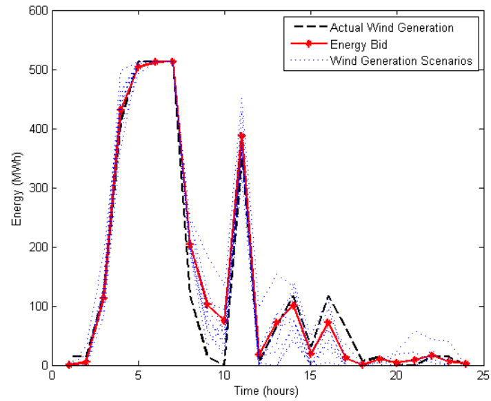
Figure D.1: Scenario Plot - Deterministic Case
