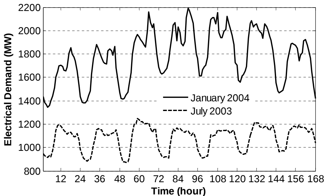
Figure 4.4: Hourly Vancouver Island electrical demand for one week periods in July 2003 and January 2004
