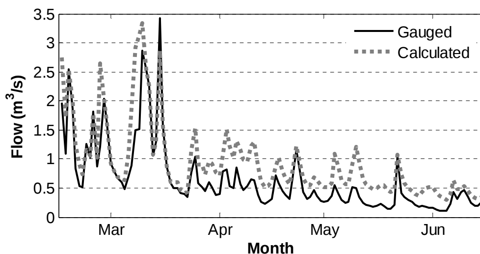
Figure 3.9: Carnation Ck. gauged flow compared to FAC calculated flow
