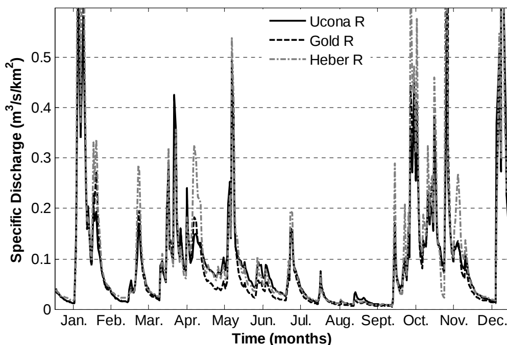
Figure 3.5: 2005 RRA 5 specific discharge hydrograph comparison
