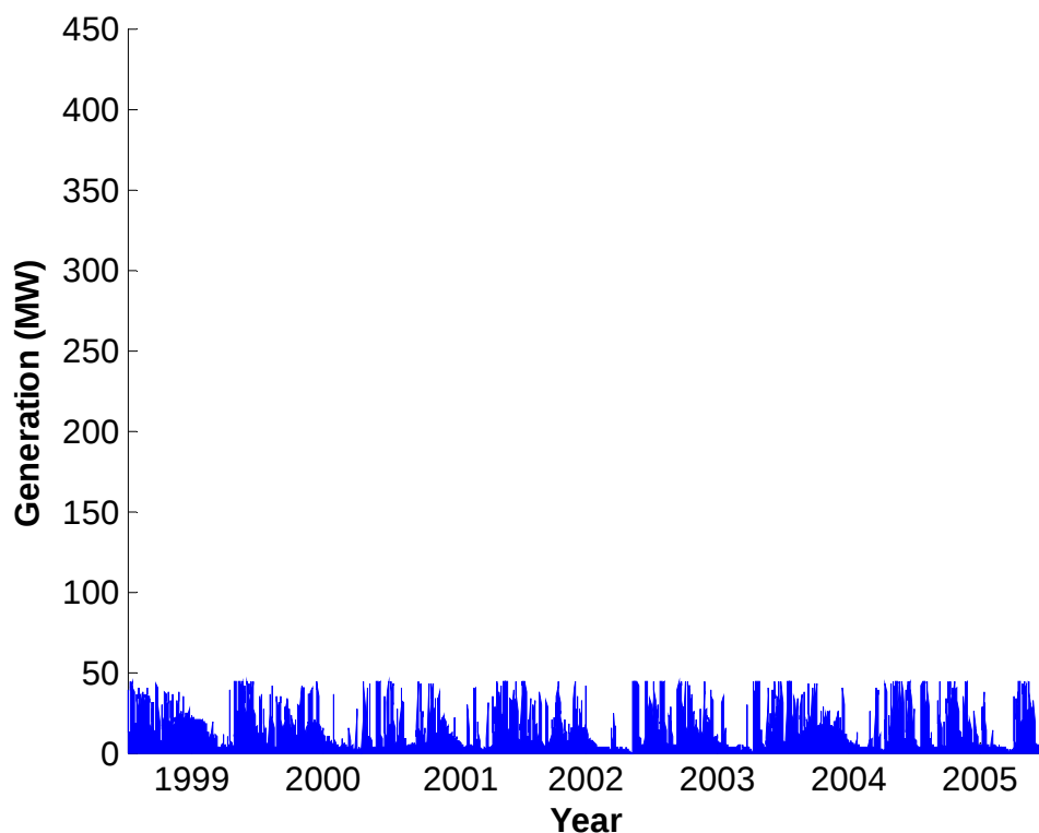
Figure 6.6: Operating daily generation output, 1999-2005
