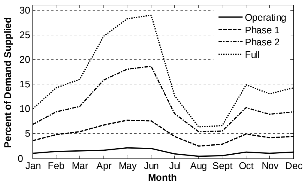
Figure 7.7: Small hydro contribution to Vancouver Island demand in 2000
