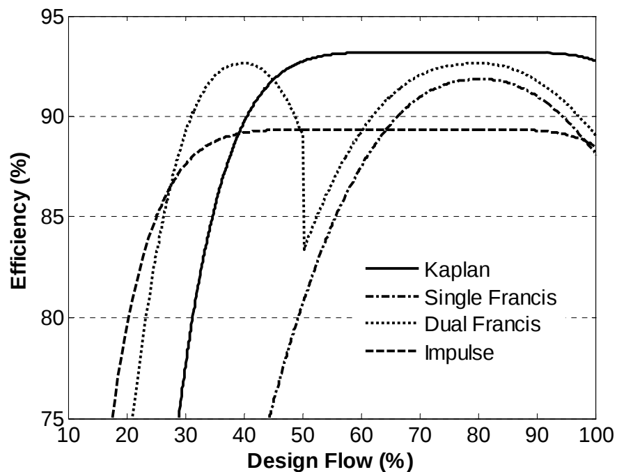
Figure 5.4: Turbine efficiency curves
