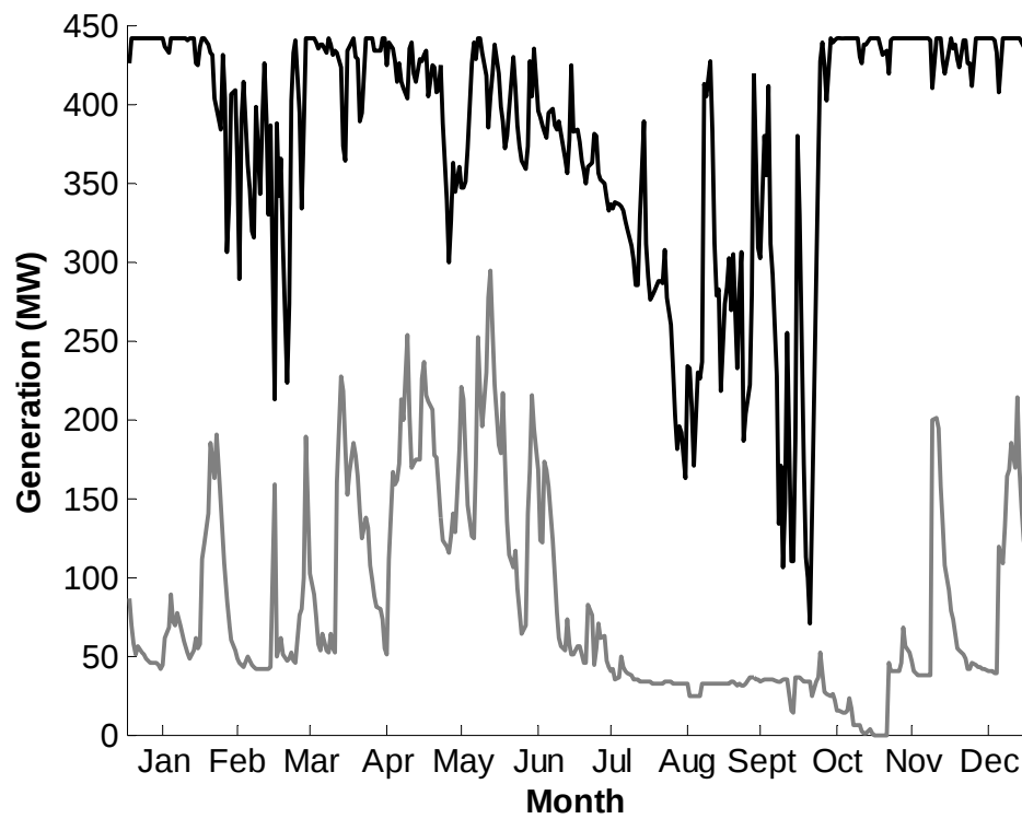
Figure 6.16: Maximum and minimum daily generation for Full development
