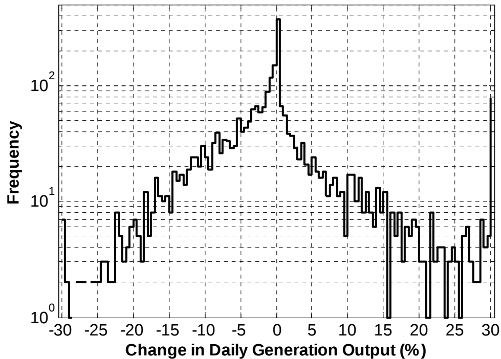
Figure 8.1: Histogram of percent change in daily generation output for full development scenario (441 MW)
