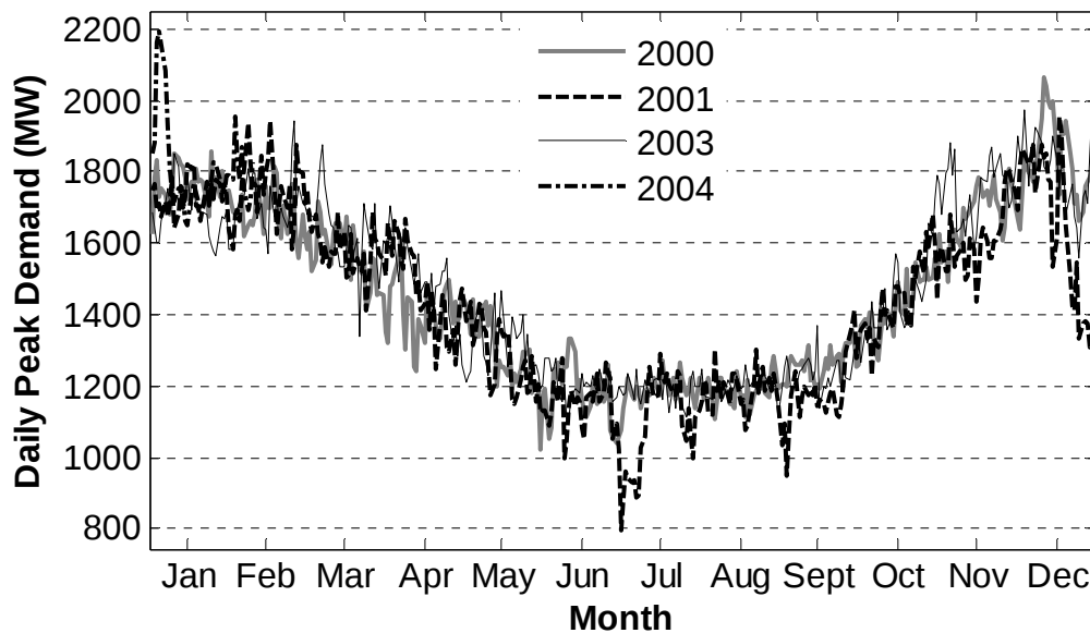
Figure 4.3: Vancouver Island peak daily demand for selected years
