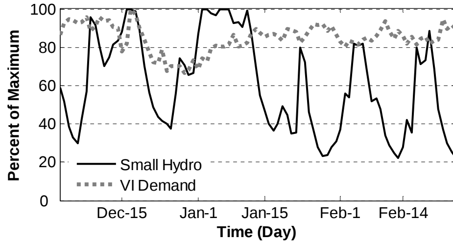
Figure 7.3: Small Hydro capacity and VI demand, Dec. 2001 – Feb. 2002
