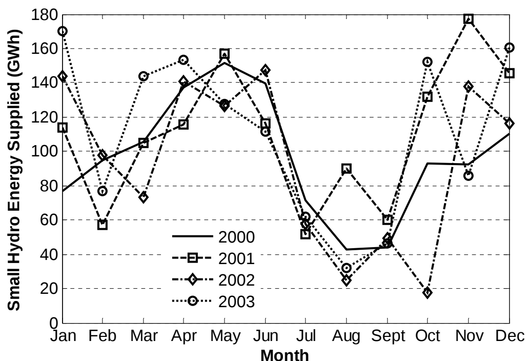
Figure 7.6: Phase 2 development energy contribution, 2000-2003
