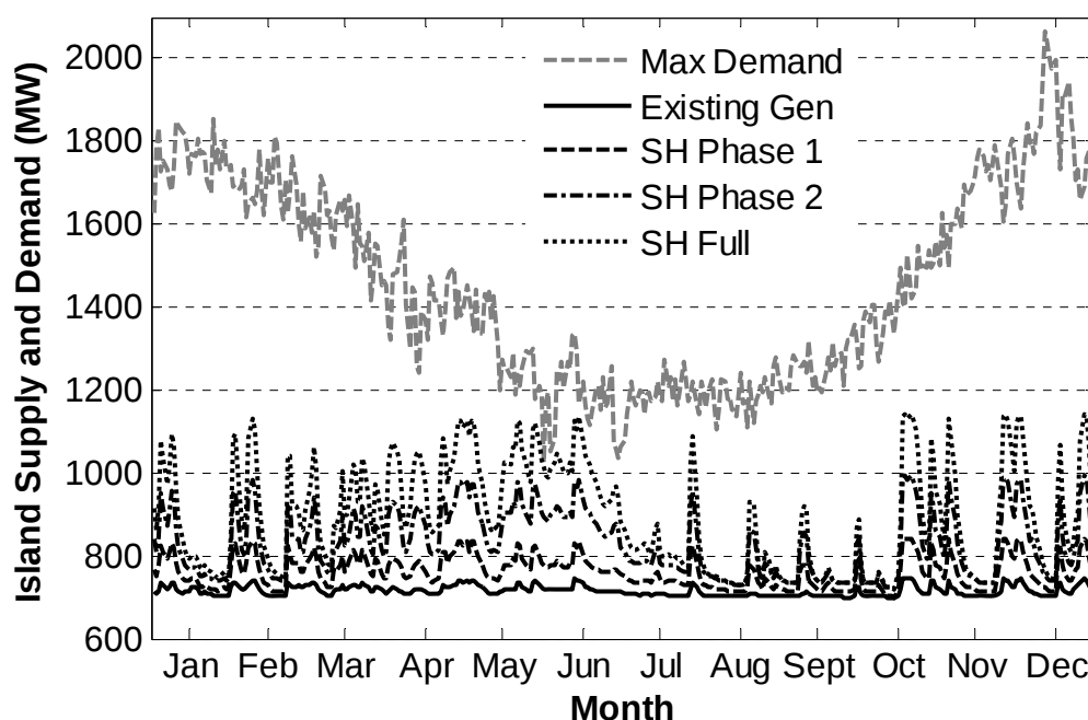
Figure 7.1: Vancouver Island Supply and Demand for 2000 with the addition of stepped small hydro development
