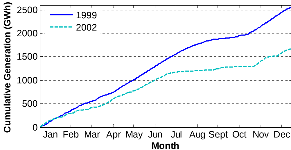
Figure 9.5: Cumulative generation for 1999 and 2002 model years
