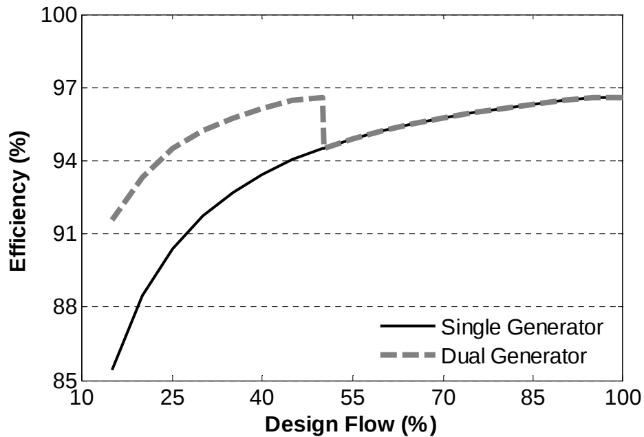
Figure 5.5: Generic generator efficiency curves
