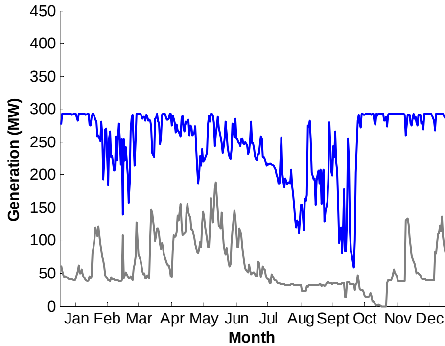
Figure 6.13: Maximum and minimum daily generation for Phase 2 development
