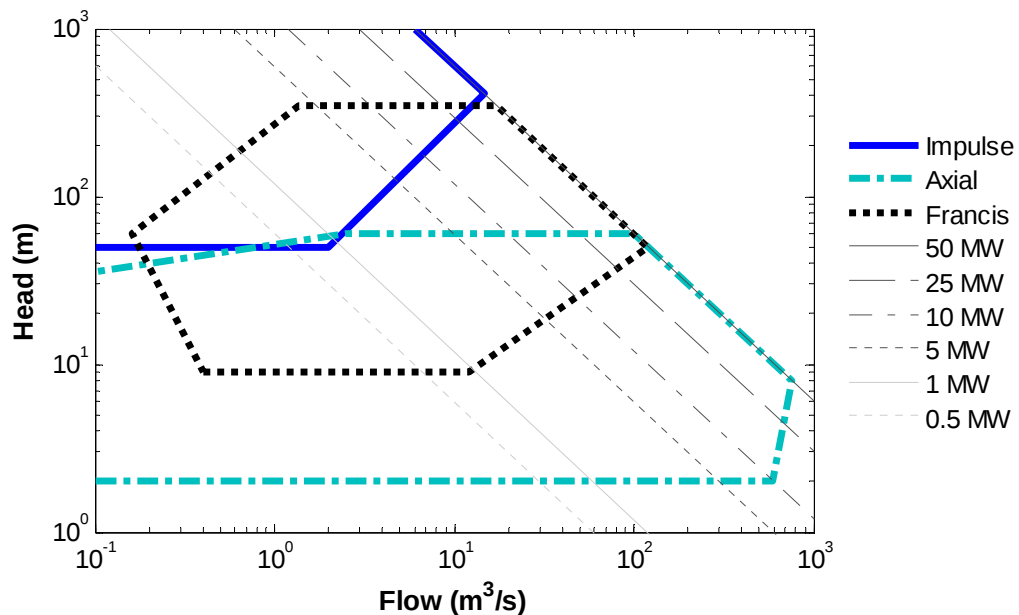
Figure 5.2: Turbine application ranges and generation potential
