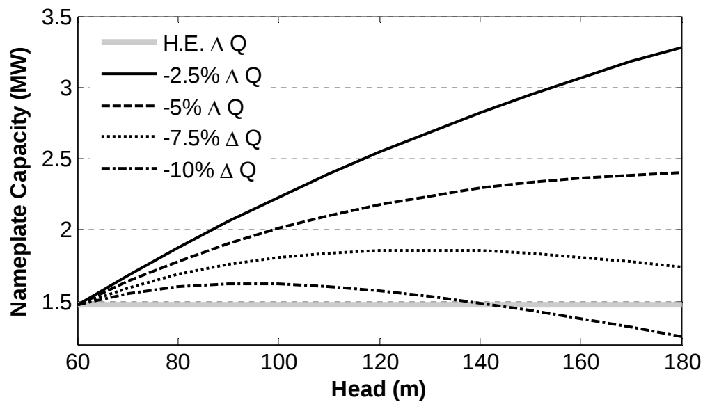
Figure 9.10: Nameplate capacity resulting from increasing head while decreasing flow requirement
