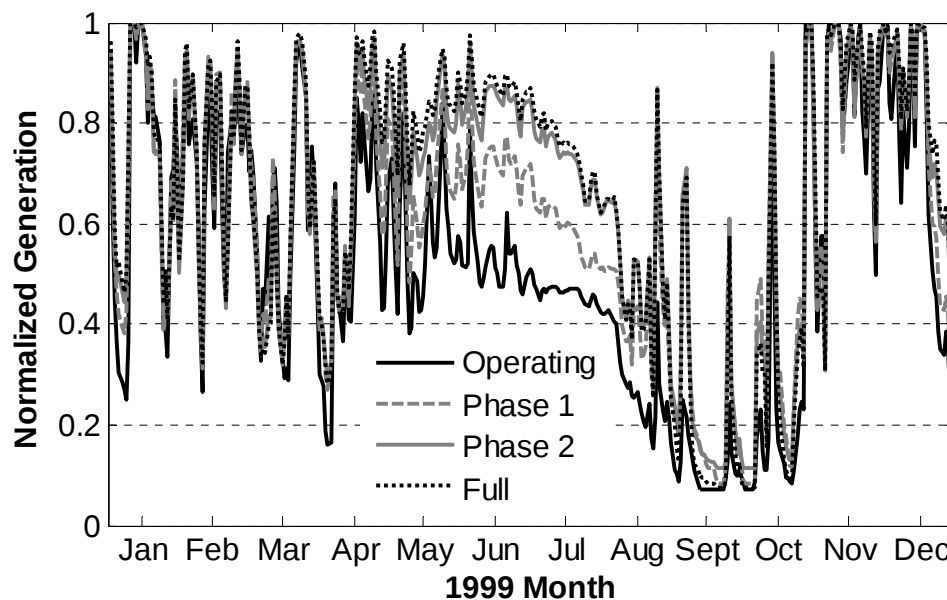
Figure 6.4: 1999 normalized generation comparison
