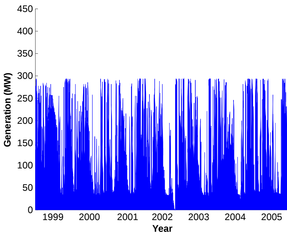
Figure 6.12: Phase 2 daily generation output, 1999-2005
