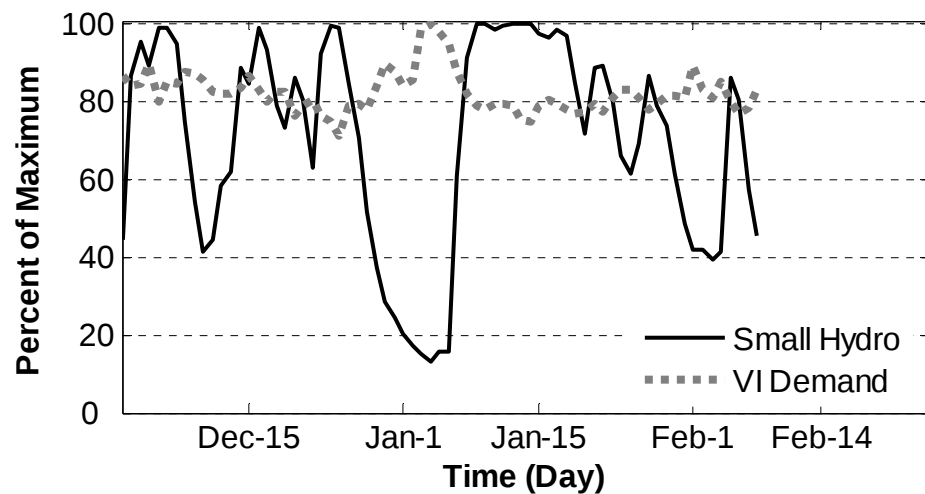
Figure 7.4: Small Hydro capacity and VI demand, Dec. 2003 – Feb. 2004
