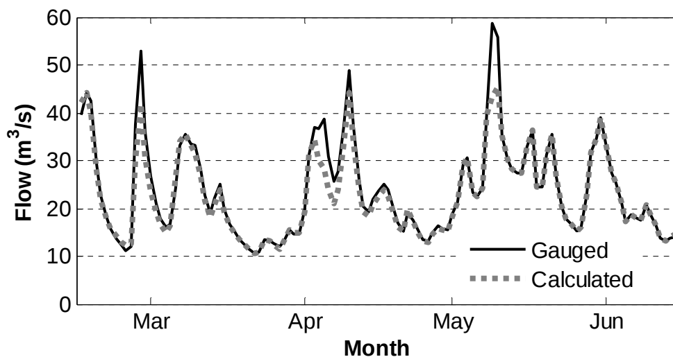
Figure 3.8: Chemanus R. gauged flow compared to FAC calculated flow
