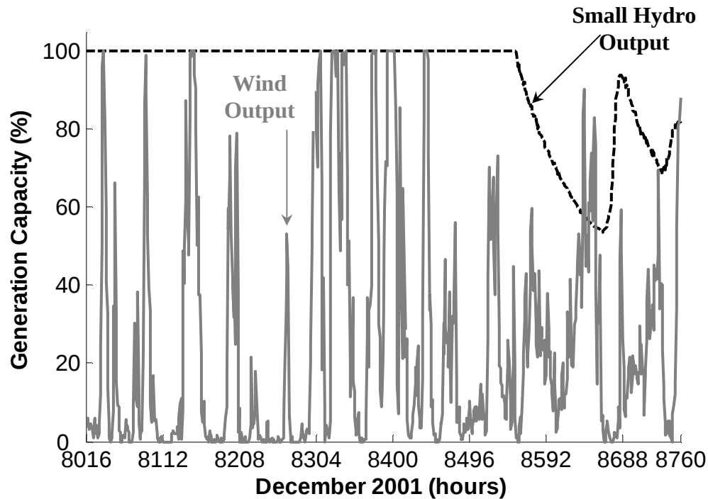
Figure 8.5: Hourly generation capacity of a wind turbine on Jordan Ridge compared to a small hydro installation on the Fleet River
