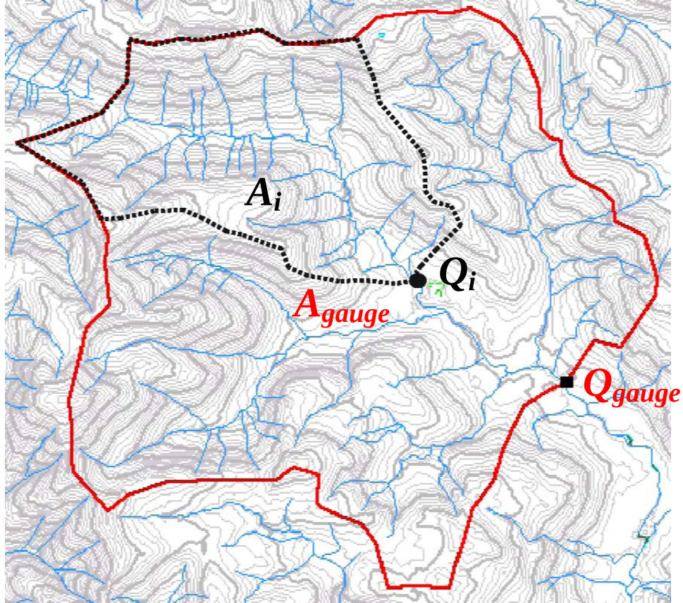
Figure 3.4: Flow adjustment diagram
