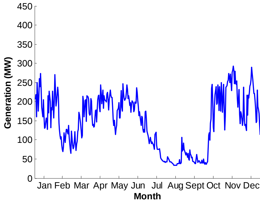
Figure 6.14: Median daily generation for Phase 2 development
