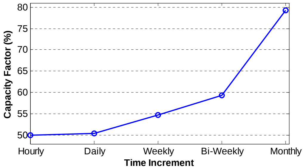
Figure 9.1: Capacity factor for Browns River site as measured using different time increments for assessment (design flow of 3.79 \text{ m}^3/\text{s} )
