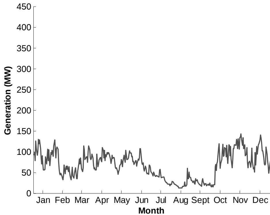
Figure 6.11: Median daily generation for Phase 1 development
