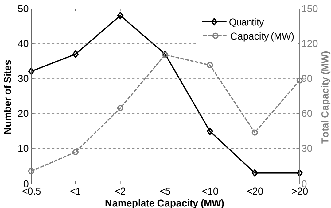
Figure 6.18: Number of sites and total capacity as a function of nameplate capacity
