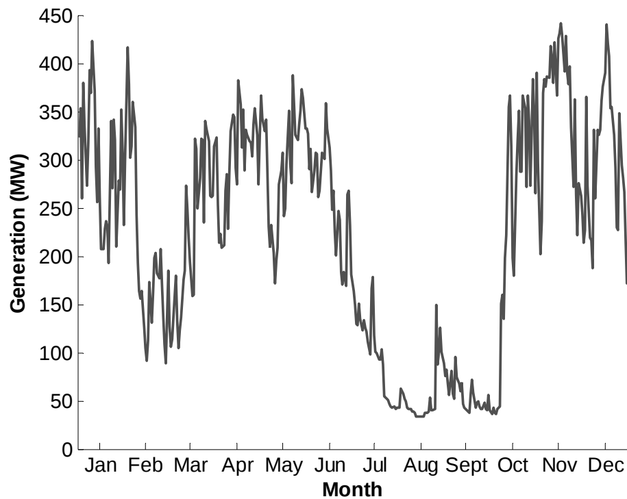
Figure 6.17: Median daily generation for Full development
