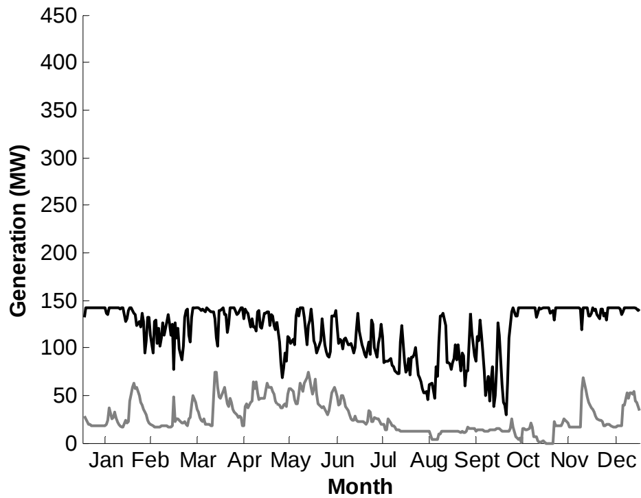
Figure 6.10: Maximum and minimum daily generation for Phase 1 development
