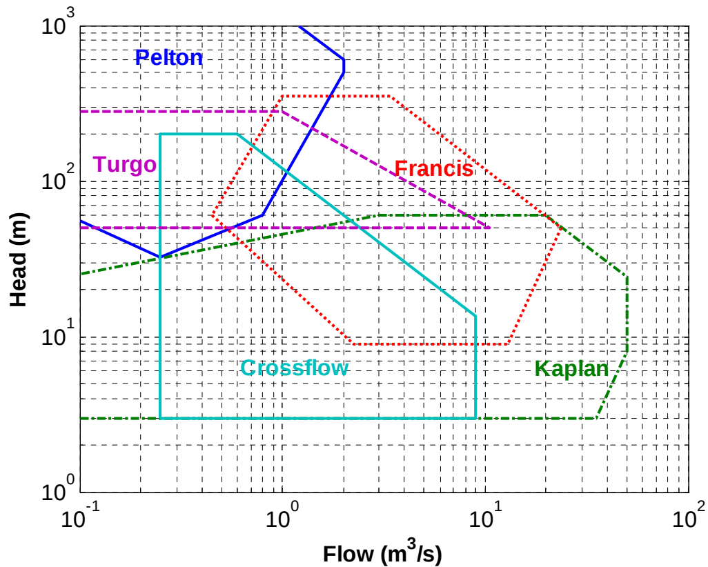
Figure 2.2: Effective head and flow combinations for typical turbine types
