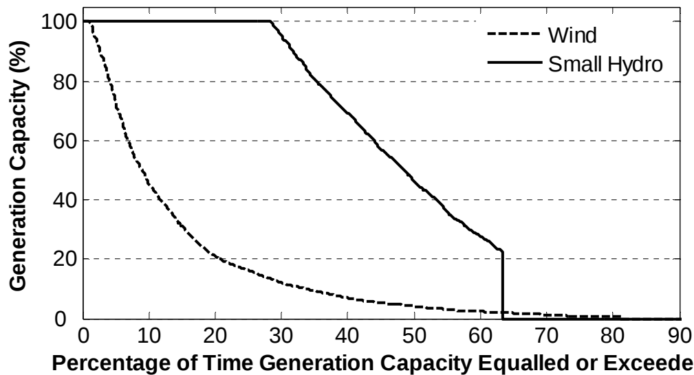
Figure 8.6: Generation Duration Curve for a wind turbine located on Jordon Ridge and a small hydro facility located on the Fleet River
