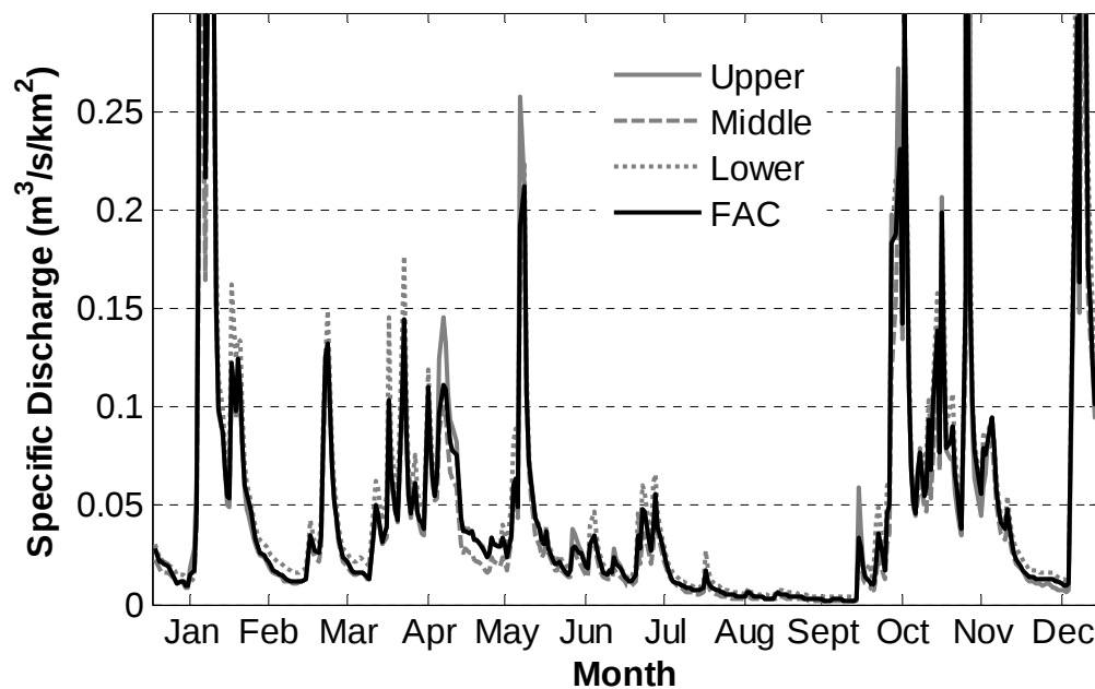
Figure 3.7: Salmon River inter-watershed specific discharge comparison
