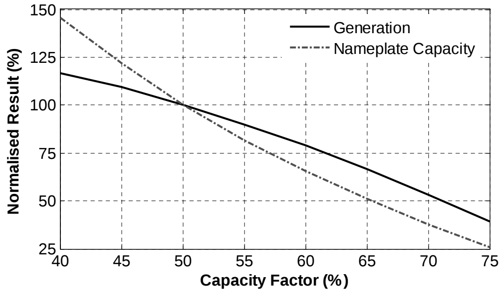
Figure 9.9: Changes to nameplate capacity and generation as a function of capacity factor
