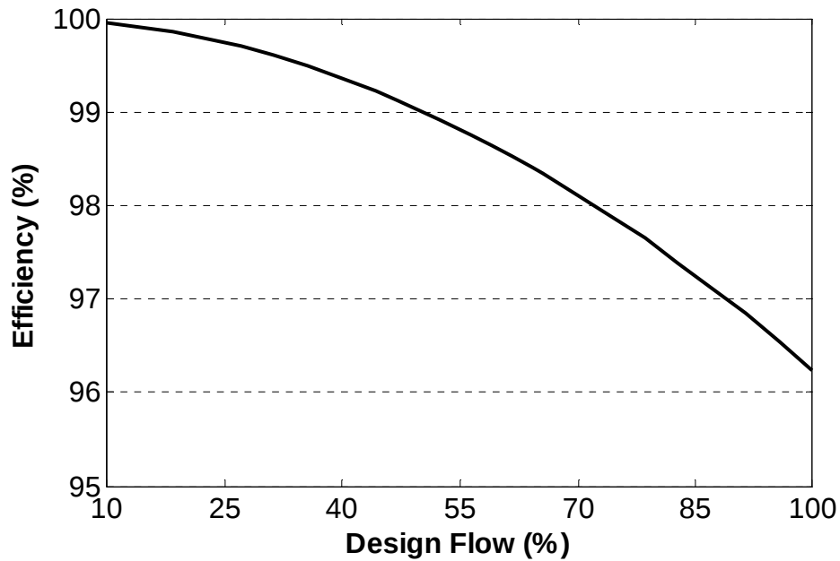
Figure 5.6: Penstock efficiency curve
