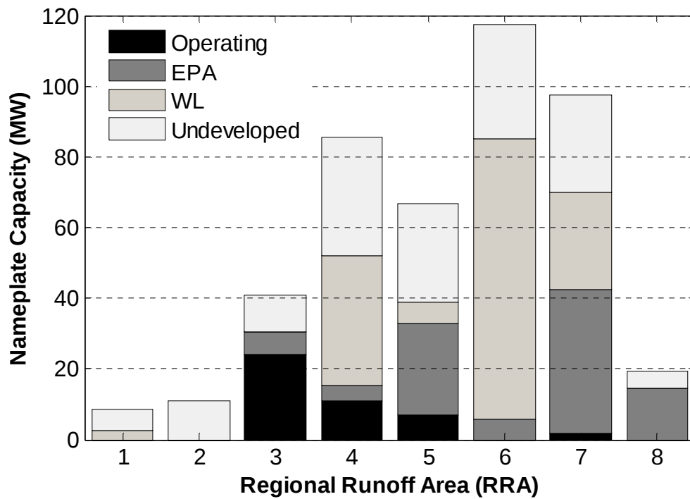
Figure 6.2: Nameplate capacity of small hydro sites by RRA
