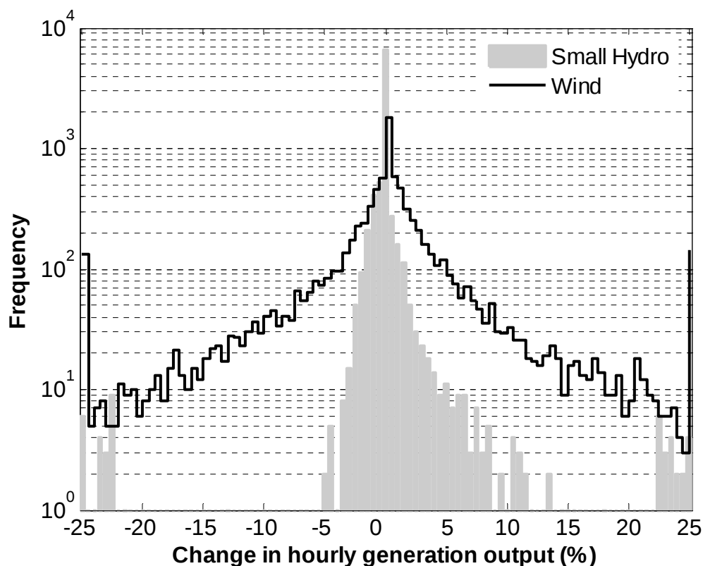
Figure 8.4: Histogram of hourly percent change in generation, small hydro vs. wind
