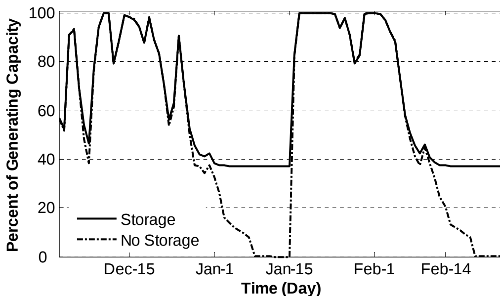
Figure 8.2: Influence of storage on generation output, 2004-2005 maximum demand period
