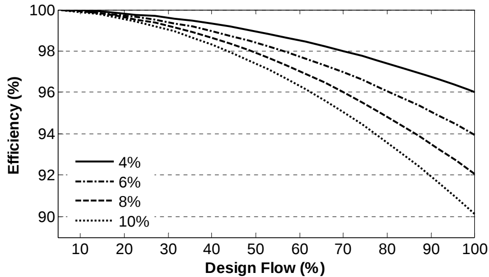
Figure 9.11: Penstock efficiency curves
