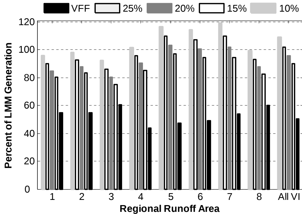
Figure 9.6: Influence of minimum in-stream flow requirements on generation as compared to lowest monthly median (LMM) result
