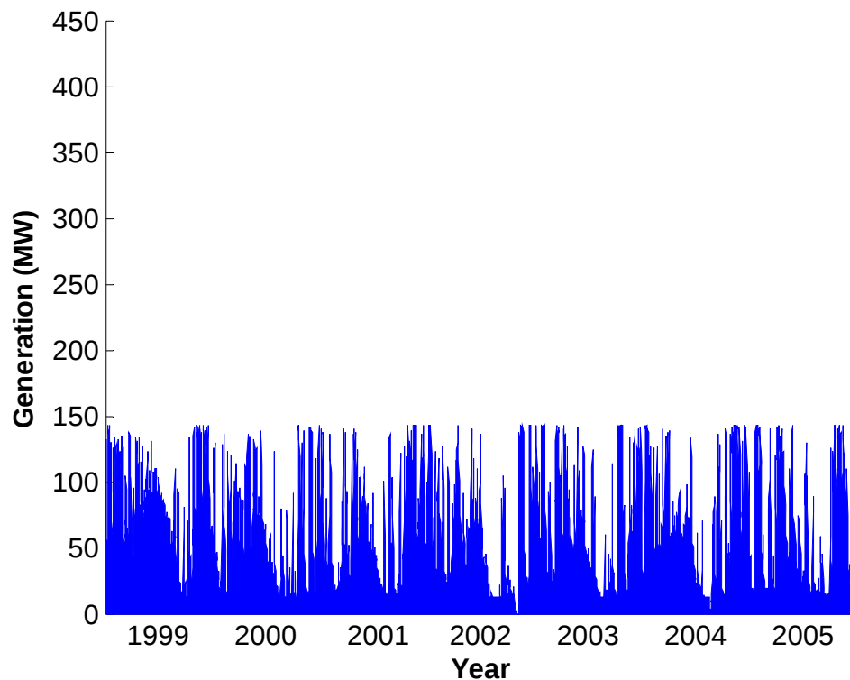
Figure 6.9: Phase 1 daily generation output, 1999-2005
