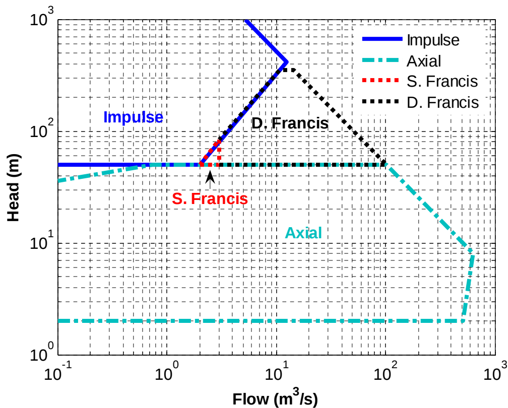
Figure 5.3: Turbine application range used in model turbine selection
