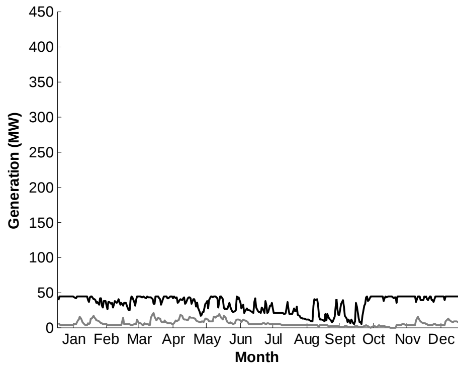
Figure 6.7: Maximum and minimum daily generation from Operating facilities
