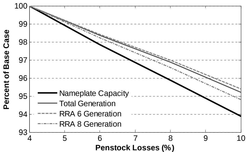
Figure 9.12: Sensitivity of nameplate capacity and total generation to penstock losses
