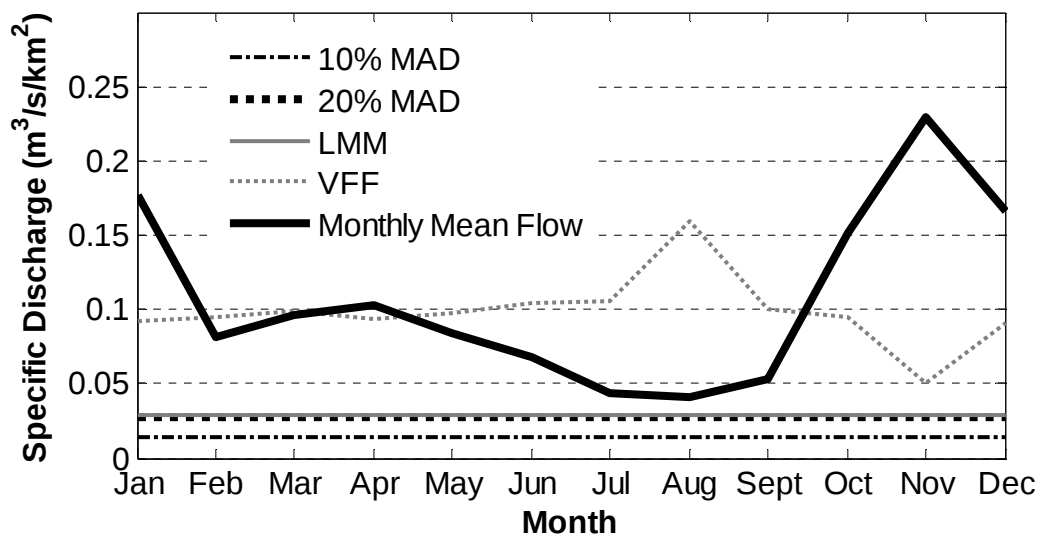
Figure 9.8: In-stream flow analysis results, RRA 7
