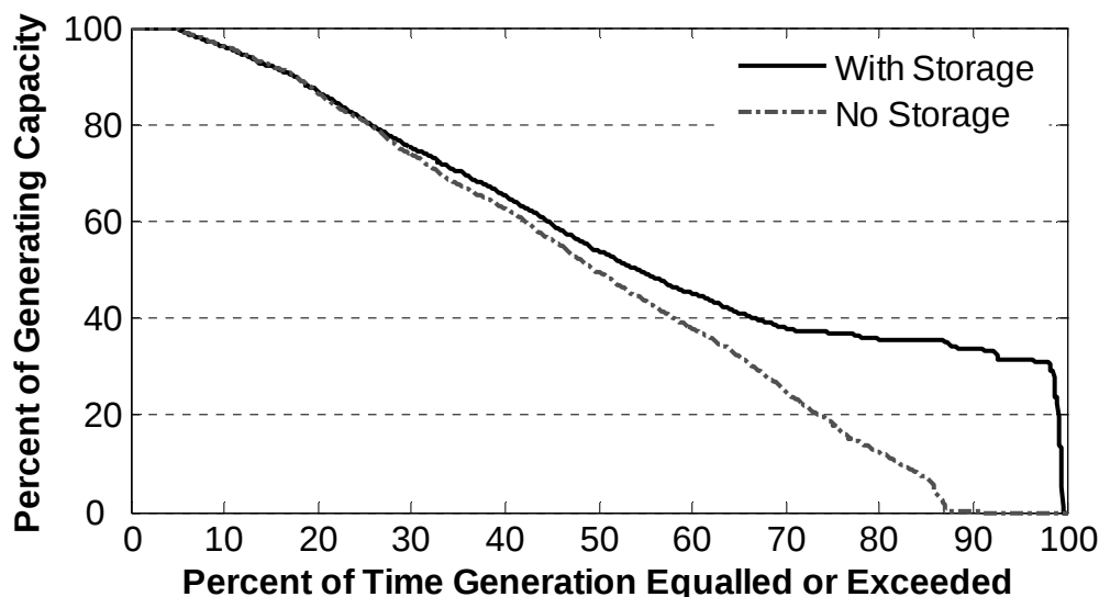
Figure 8.3: Generation duration curve of storage vs. non-storage facilities
