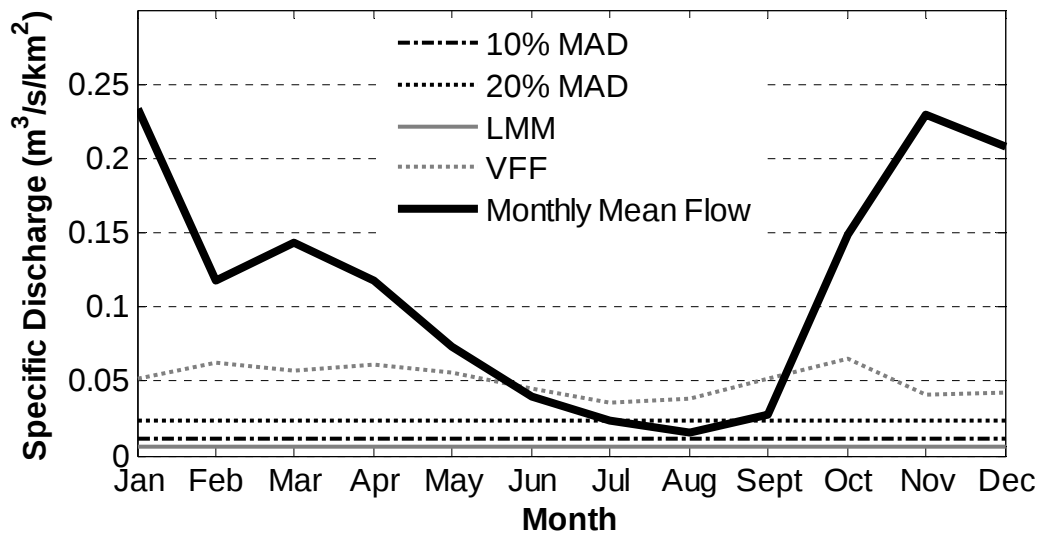
Figure 9.7: In-stream flow analysis results, RRA 3
