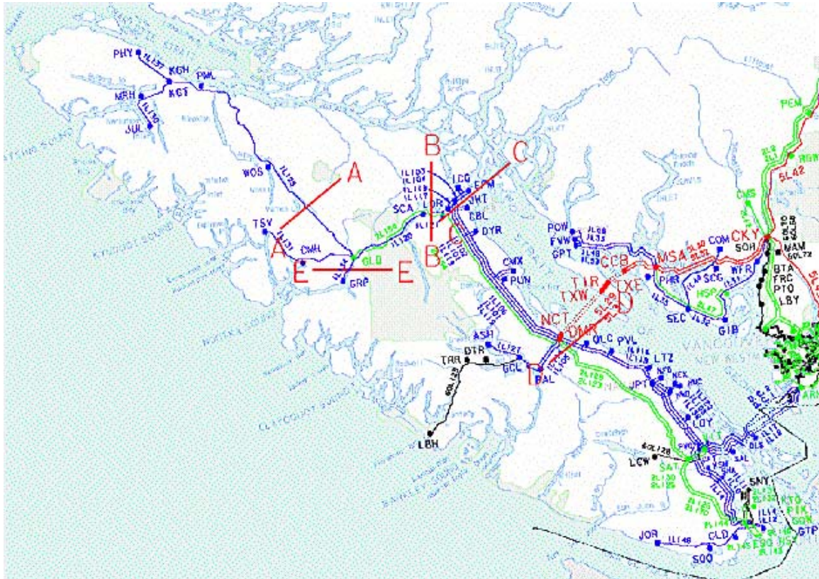
Figure 4.2: Vancouver Island electrical transmission grid [73]
