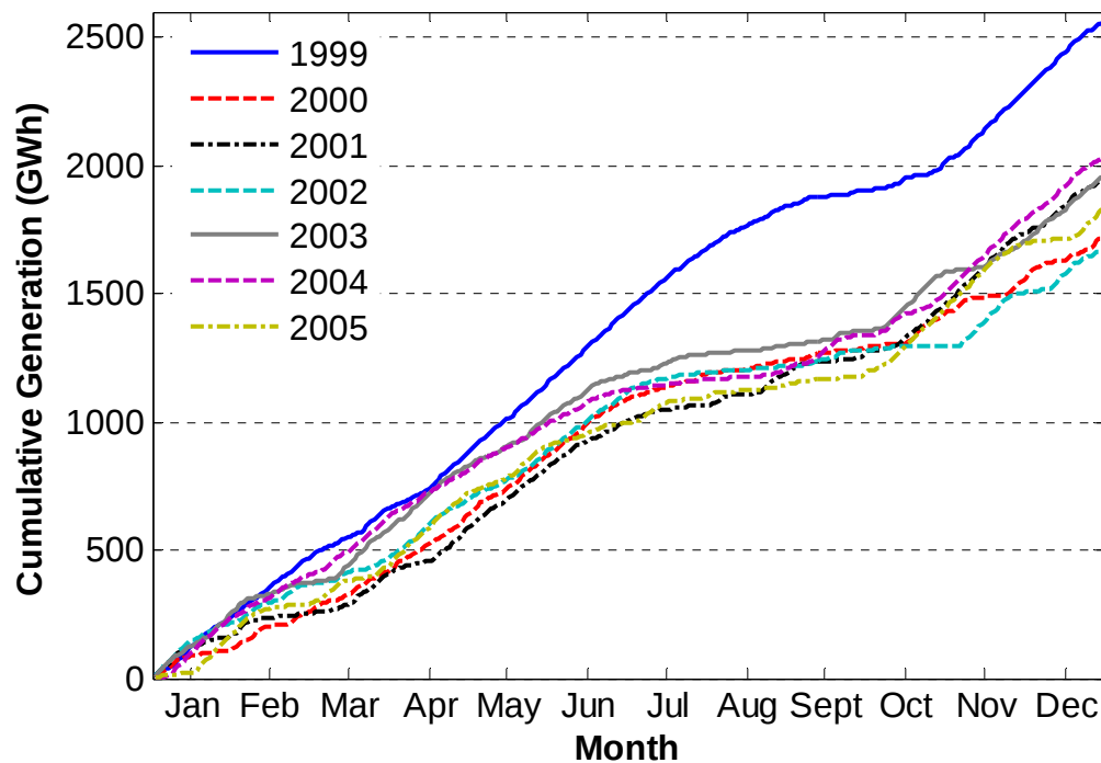
Figure 9.4: Cumulative generation for each model year using the full development scenario, 1999 - 2005
