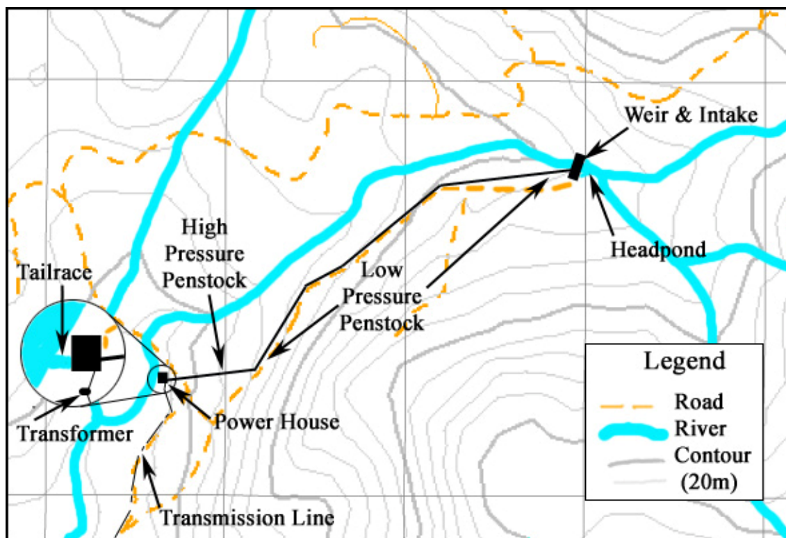
Figure 2.1: Layout of a small hydroelectric facility
