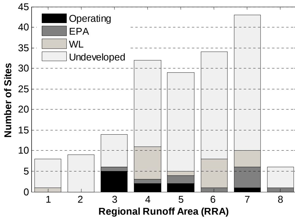
Figure 6.1: Number of small hydro sites by RRA
