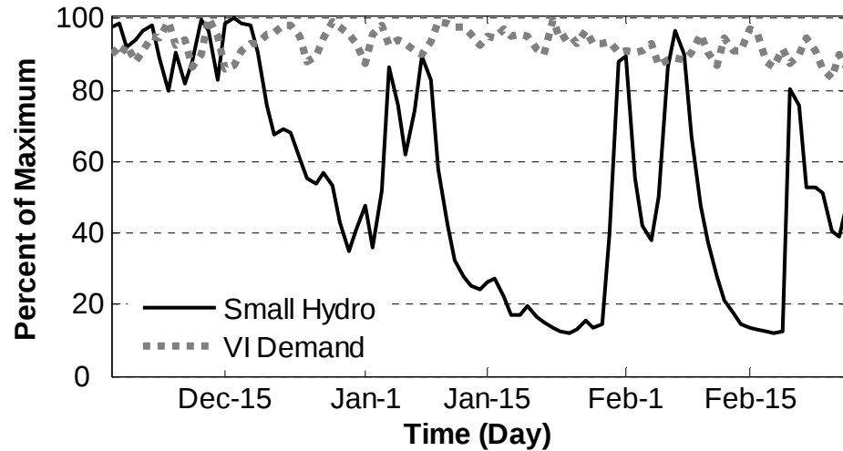
Figure 7.2: Small Hydro capacity and VI demand, Dec. 1999 – Feb. 2000
