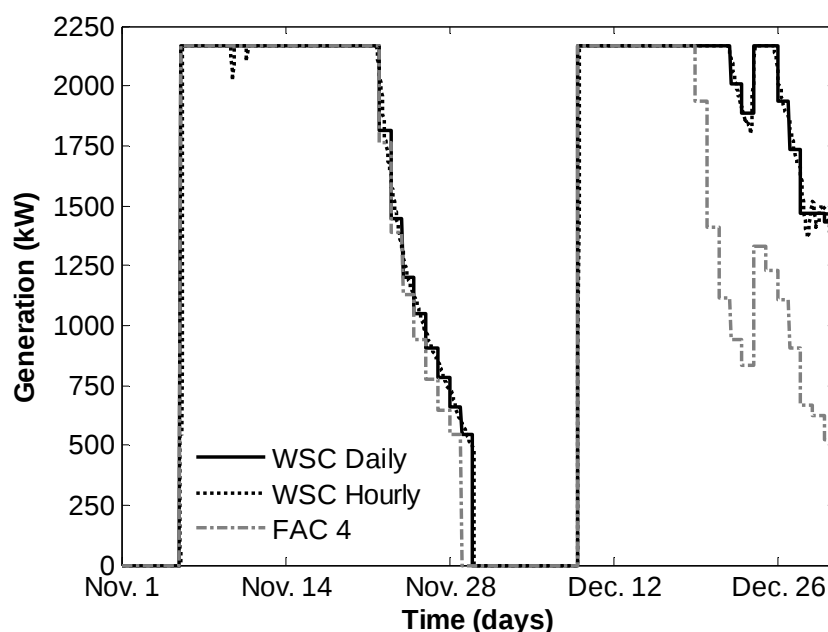
Figure 5.8: Browns River generation comparison, Nov. 1 – Dec. 31, 2004
