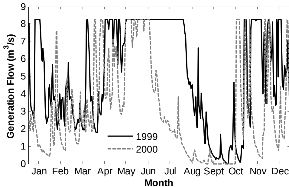
Figure 9.3: Generation hydrograph for a 100 km 2 watershed in RRA 4 1999 and 2000
