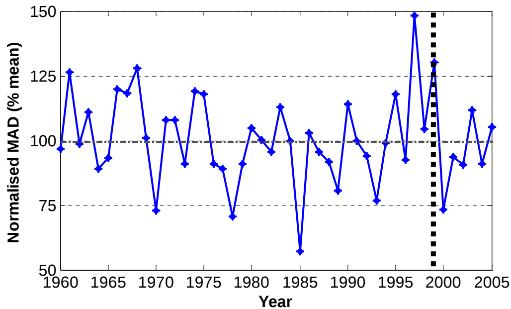
Figure 9.2: Vancouver Island mean annual runoff comparison 1960 – 2005
