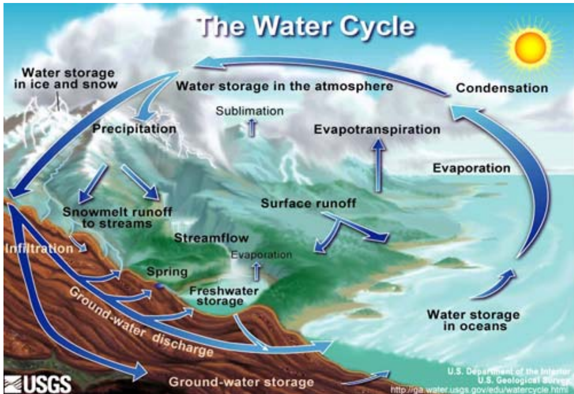
Figure 3.1: The hydrologic cycle [48]
