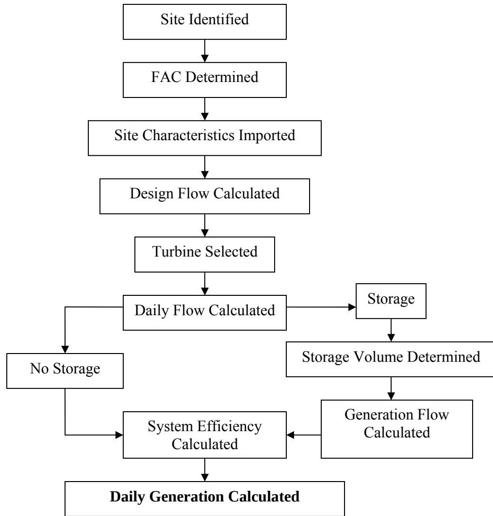
Figure 5.7: Model calculation schematic
