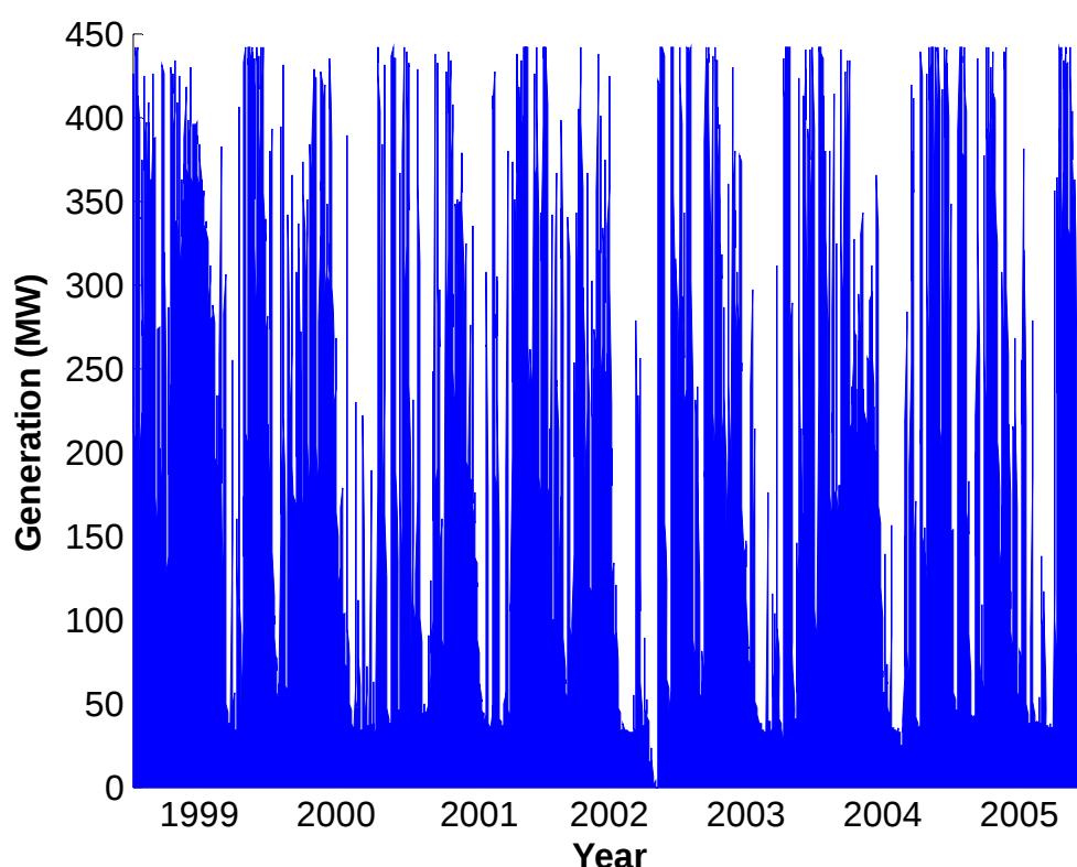
Figure 6.15: Full development daily generation output, 1999-2005
