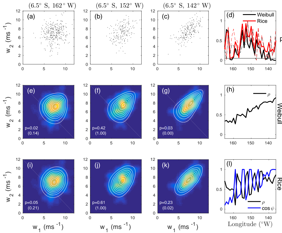
Figure 8. Joint distribution of DJF QuikSCAT wind speeds at (6.5° S, 135° W), denoted w_1 , and westward along a zonal transect to 165° W (denoted w_2 ). (a–c) Scatterplots of wind speed at (6.5° S, 135° W) and at the points (6.5° S, 162° W), (6.5° S, 152° W), and (6.5° S, 142° W). (e–g) Kernel density estimate of the joint pdf (colour) as well as the maximum likelihood bivariate Weibull distribution (white contours). The p -value of a goodness-of-fit test of the bivariate Weibull distribution is quoted in white. The values in brackets are the p -values obtained when the dependence structure is eliminated by shuffling the values of w_2 in time. (i–k) As in panels (e–g) but for the bivariate Rice distribution. (d) p -values of the bivariate goodness-of-fit tests for the wind speeds along the transect, for the bivariate Weibull distribution (solid black) and for the bivariate Rice distribution (solid red). The dashed lines correspond to the p -values for shuffled w_2 . (h) Estimate of the parameter \rho from the best-fit bivariate Weibull distribution along the transect. (l) Estimate of the parameters \rho (black) and \cos \psi (blue) from the best-fit bivariate Rice distribution along the transect. Values of the best-fit model parameters are given in Table 1.
