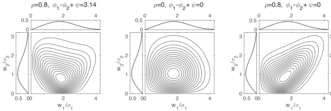
Figure 3. As in Fig. 1 for the bivariate Rice distribution with (\bar{w}_1, \sigma_1, \bar{w}_2, \sigma_2) = (6, 4, 2, 5) and (\rho, \phi_1 - \phi_2 + \psi) = (0.8, \pi), (0, 0), and (0.8, 0) .
