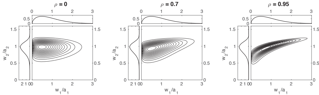
Figure 4. As in Fig. 1 for the bivariate Weibull distribution with (a_1, b_1, a_2, b_2) = (4, 1.5, 5, 7) and \rho = 0, 0.7, and 0.95 and the speeds w_1, w_2 scaled respectively by the Weibull scale parameters a_1, a_2 .
