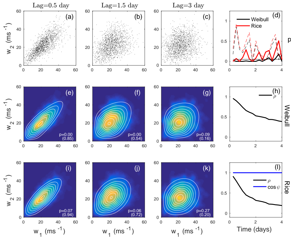
Figure 6. The temporal dependence structure of 500 hPa DJF 00Z wind speeds at ( 39^{\circ} S, 216^{\circ} W) for lags s = 0.25 to 4 days, with w_1 = w(t_n) and w_2 = w(t_{n+s}) . (a–c) Scatterplots of wind speeds separated by 0.5 days (first column), 1.5 days (second column), and 3 days (third column). (e–g) Maximum likelihood bivariate Weibull distribution (white contours) and kernel density estimate of the joint pdf of the lagged data. The p -value of a goodness-of-fit test of the bivariate Weibull fit is quoted in white. The values in brackets are the p -values obtained when the dependence structure is eliminated by shuffling the values of w_2 in time. (i–k) As in panels (e–g) for the bivariate Rice distribution. Panels (d, h, l) show results at a range of different time lags. (d) p -values of bivariate goodness-of-fit tests for bivariate Weibull (solid black) and bivariate Rice (solid red). The dashed lines correspond to the p -values for shuffled w_2 . The thin black curve is the 0.95 significance level. (h) Best-fit estimate of the parameter \rho of the bivariate Weibull distribution. (l) Best-fit estimates of \rho (black) and \cos \psi (blue) for the Rice distribution. Values of the best-fit model parameters are given in Table 1.
