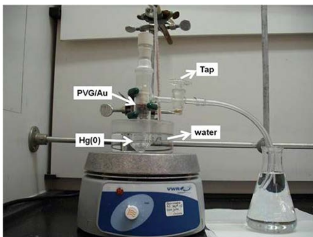
Figure 3. Experimental setup used to expose PVG/Au samplers to mercury vapor in different times at 22 °C.
