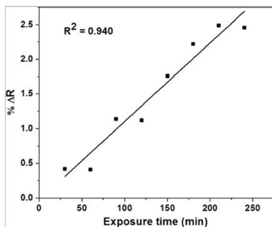
Figure 9. Variation of the PVG/Au reflectance before and after Hg° exposure for 240 min (experiment performed with vapor pressure of Hg° at 60 °C).
