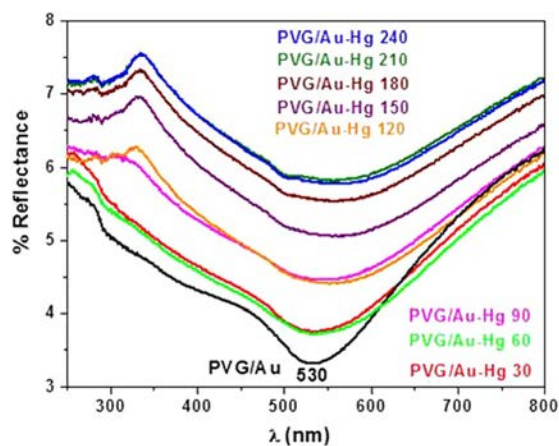
Figure 8. UV-vis spectra of PVG/Au before and after Hg° exposure for 240 min (experiment performed with vapor pressure of Hg° at 60 °C).
