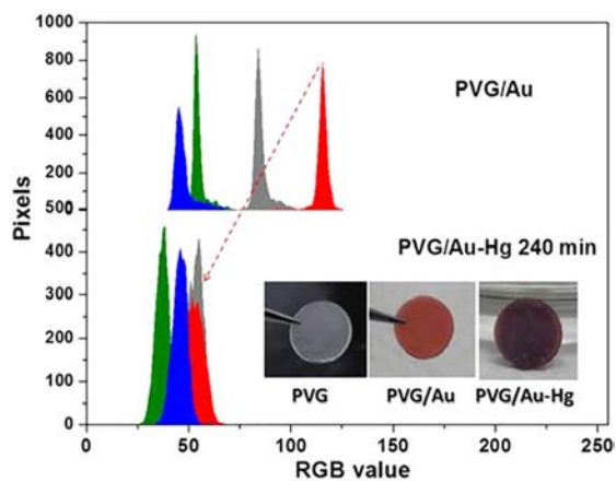
Figure 7. From left to right: PVG disc (colorless), PVG/Au disc (red), and PVG/Au after exposure to Hg° vapor for 240 min (PVG/Au-Hg). RGB and gray histograms of PVG/Au and PVG/Au after 240 min of exposure to Hg° (experiment performed with vapor pressure of Hg° at 60 °C).
