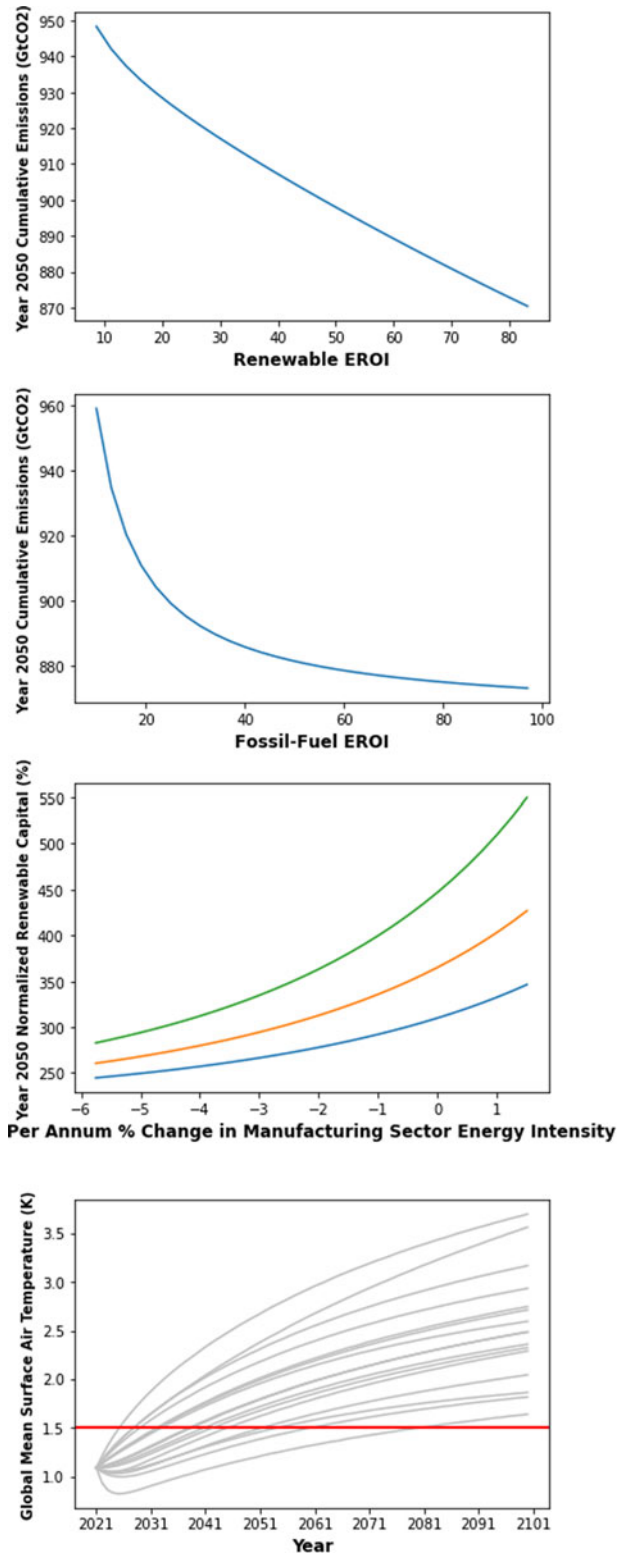
Fig. 4. Panels (1) and (2) display a sensitivity of year 2050 cumulative emissions over a range of assumed values for the renewable and fossil-fuel EROIs. Panel (3) displays the year 2050 renewable capital stock for each of the growth assumptions across a range of energy intensity assumptions. Panel (4) (grey plots) displays the global average surface temperature trajectories for each of model representative parametrizations of the underlying CMIP5 climate models. Growth scenario trajectories (green plots), steady-state trajectories (orange plots), degrowth scenario trajectories (blue plots).
