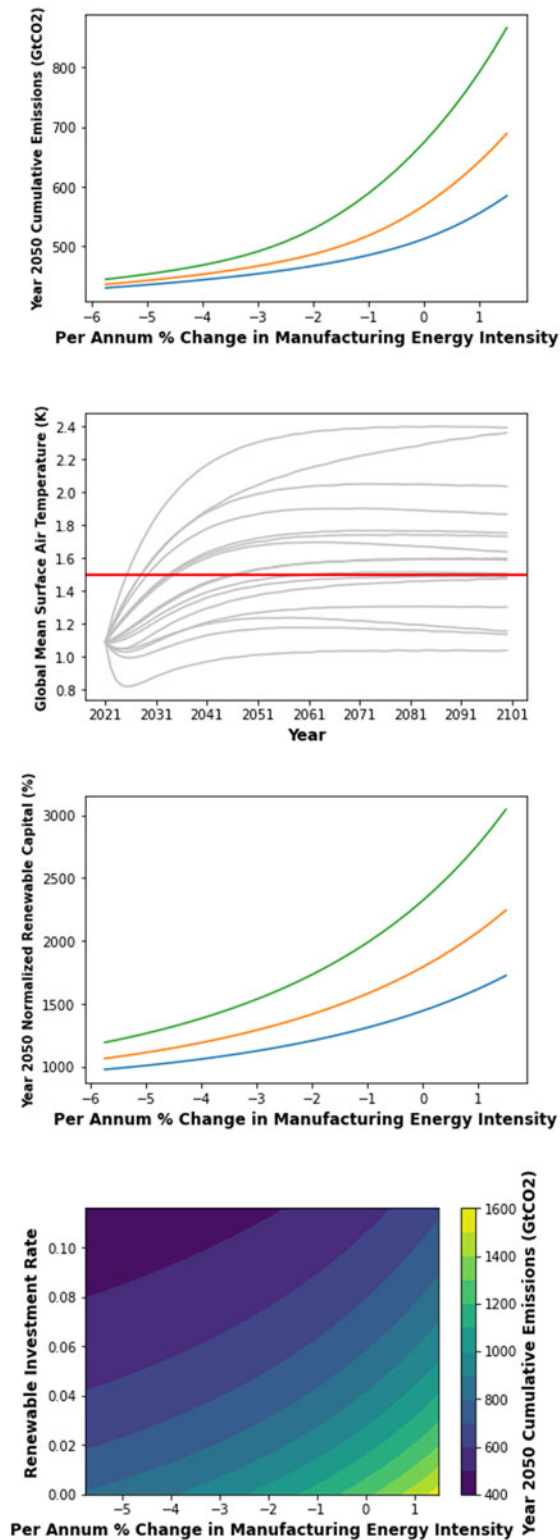
Fig. 6. Panels (1) and (3) display a sensitivity analysis of year 2050 cumulative emissions and year 2050 renewable capital stock sizes over a range of per annum energy intensity declines. Panel (2) (grey plots) displays the global average surface temperature trajectories for each of model representative parametrizations of the underlying CMIP5 climate models. Panel (4) displays the contour plot for year 2050 cumulative emissions over a range of energy intensity declines and renewable investment rates. Growth scenario trajectories (green plots), steady-state trajectories (orange plots), degrowth scenario trajectories (blue plots). The solid red lines in panels (2) and (3) correspond to the 500 GtCO 2 carbon budget and 1.5°C warming threshold, respectively.
