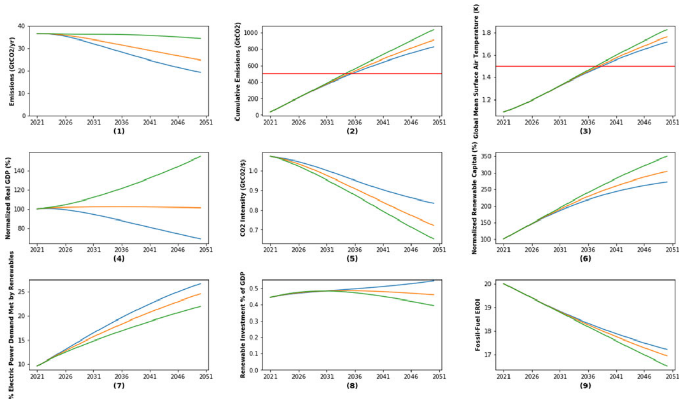
Fig. 2. Trajectories for select SFCIO-IAM model variables assuming \Delta_1 = 0.01 and \sigma_{ne}^M = 0.03 . Growth scenario trajectories (green plots), steady-state trajectories (orange plots), degrowth scenario trajectories (blue plots). The solid red lines in panels (2) and (3) correspond to the 500 GtCO 2 carbon budget and 1.5°C warming threshold, respectively.
