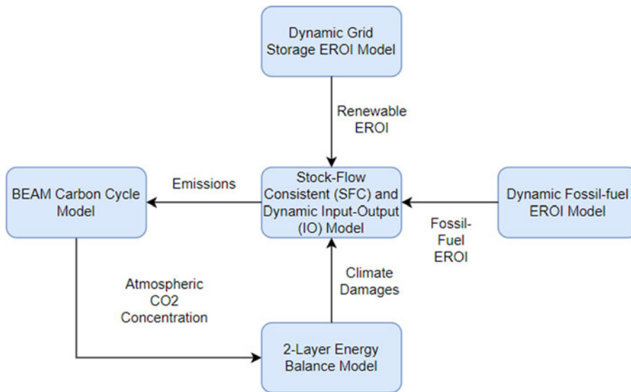
Fig. 1. Overview of key SFCIO-IAM model components.
