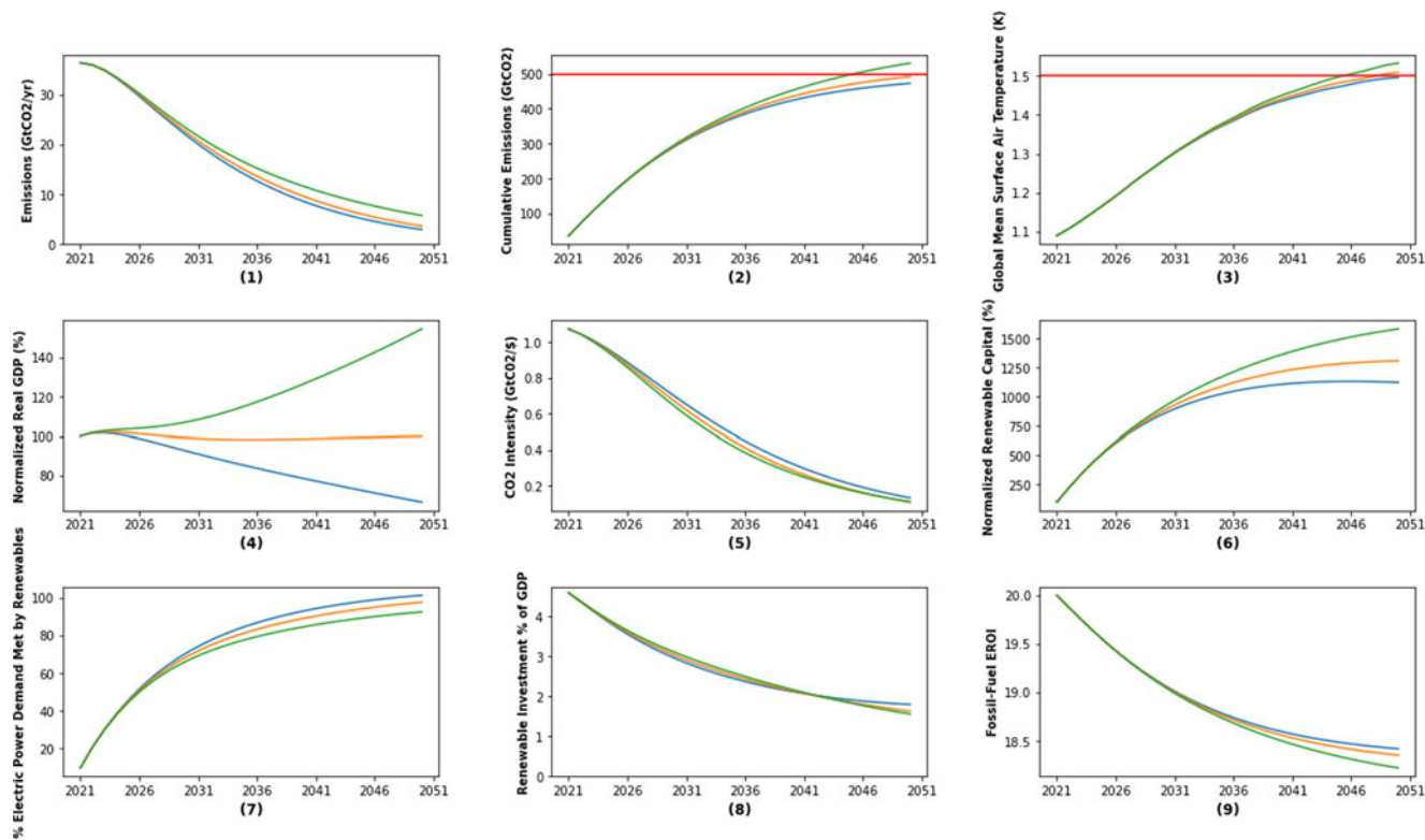
Fig. 5. Trajectories for select SFCIO-IAM model variables assuming \Delta_1 = 0.105 and \sigma_{ne}^M = 0.05 . Growth scenario trajectories (green plots), steady-state trajectories (orange plots), degrowth scenario trajectories (blue plots). The solid red lines in panels (2) and (3) correspond to the 500 GtCO 2 carbon budget and 1.5°C warming threshold, respectively.
