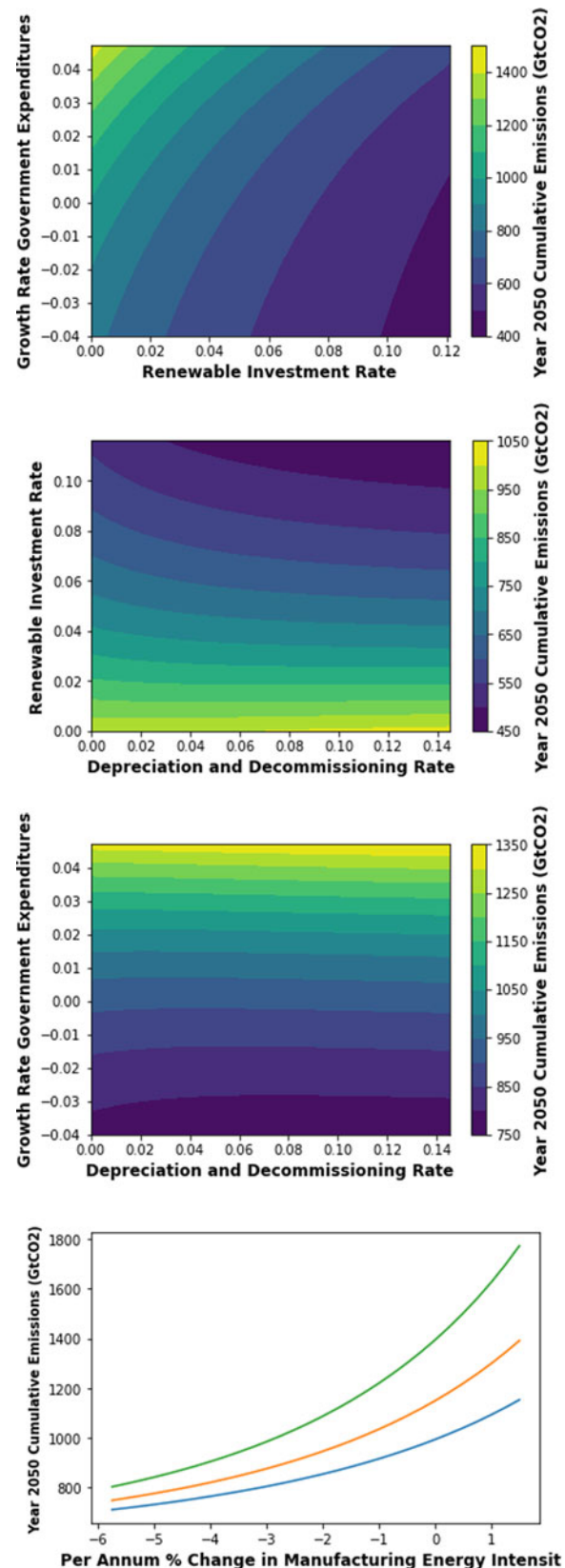
Fig. 3. Panels (1), (2) and (3) display contour plots of year 2050 cumulative emissions for various combinations of underlying model variables. Panel (4) displays a sensitivity analysis of year 2050 cumulative emissions over a range of per annum energy intensity declines. Growth scenario trajectories (green plots), steady-state trajectories (orange plots), degrowth scenario trajectories (blue plots).
