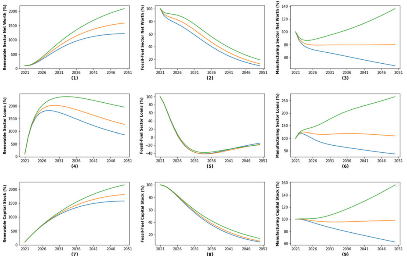
Fig. 7. Trajectories for SFCIO-IAM sectoral model variables assuming \Delta_1 = 0.105 and \sigma_{ne}^M = 0.05 . Growth scenario trajectories (green plots), steady-state trajectories (orange plots), degrowth scenario trajectories (blue plots).
