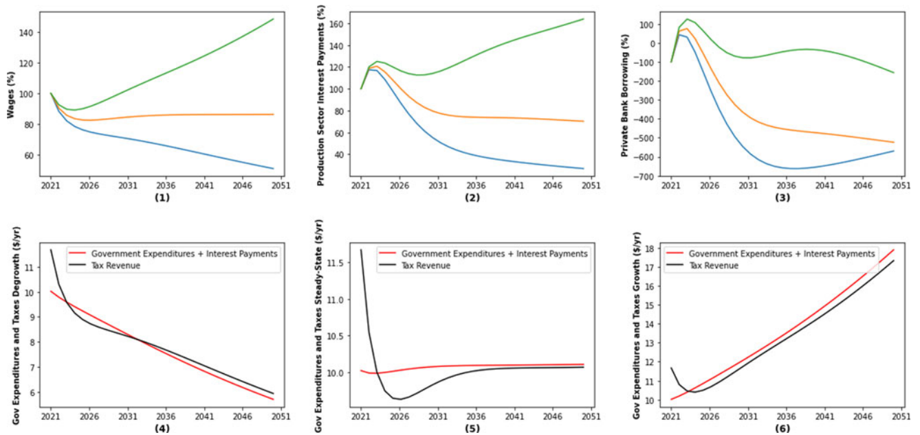
Fig. 8. Trajectories for SFCIO-IAM sectoral macroeconomic variables assuming \Delta_1 = 0.105 and \sigma_{ne}^M = 0.05 . Growth scenario trajectories (green plots), steady-state trajectories (orange plots), degrowth scenario trajectories (blue plots).
