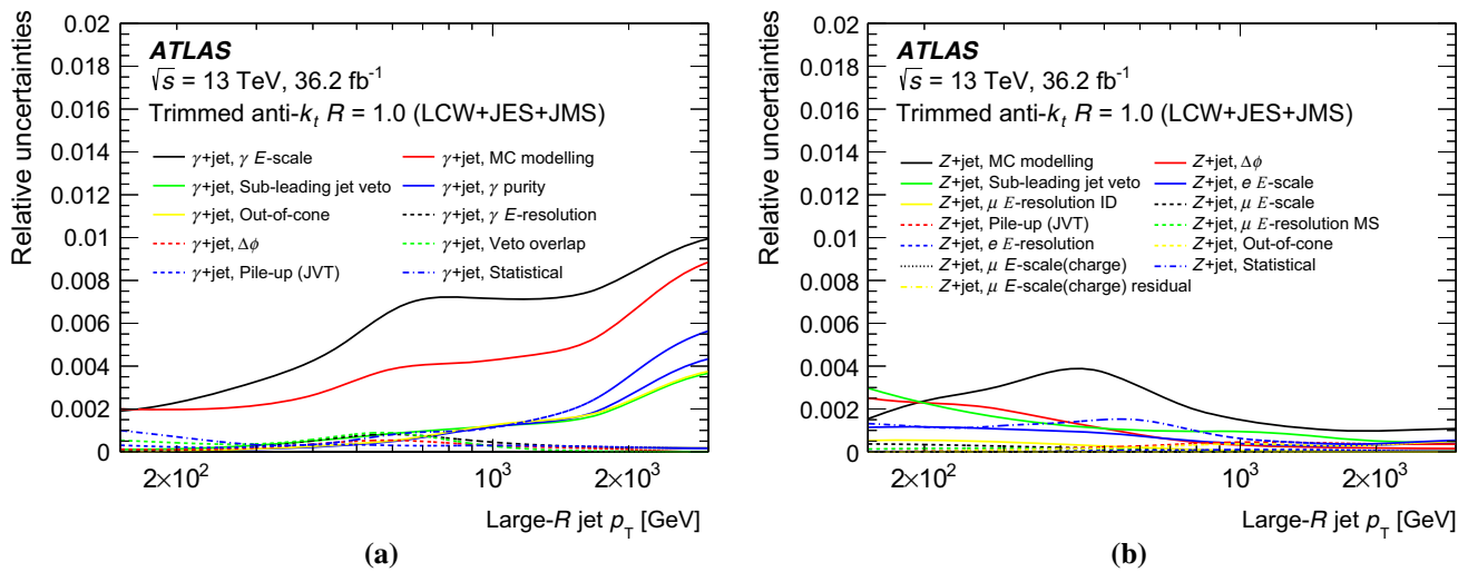
Fig. 28 Breakdown of the combined uncertainty in the large- R jet p_T response as a function of the jet transverse momentum p_T , for the a \gamma +jet and b Z+jet analyses. Contributions are shown for each of the nuisance parameters of the \gamma +jet and Z+jet balance methods. The vertical axis reflects the uncertainty introduced by a given nuisance parameter
