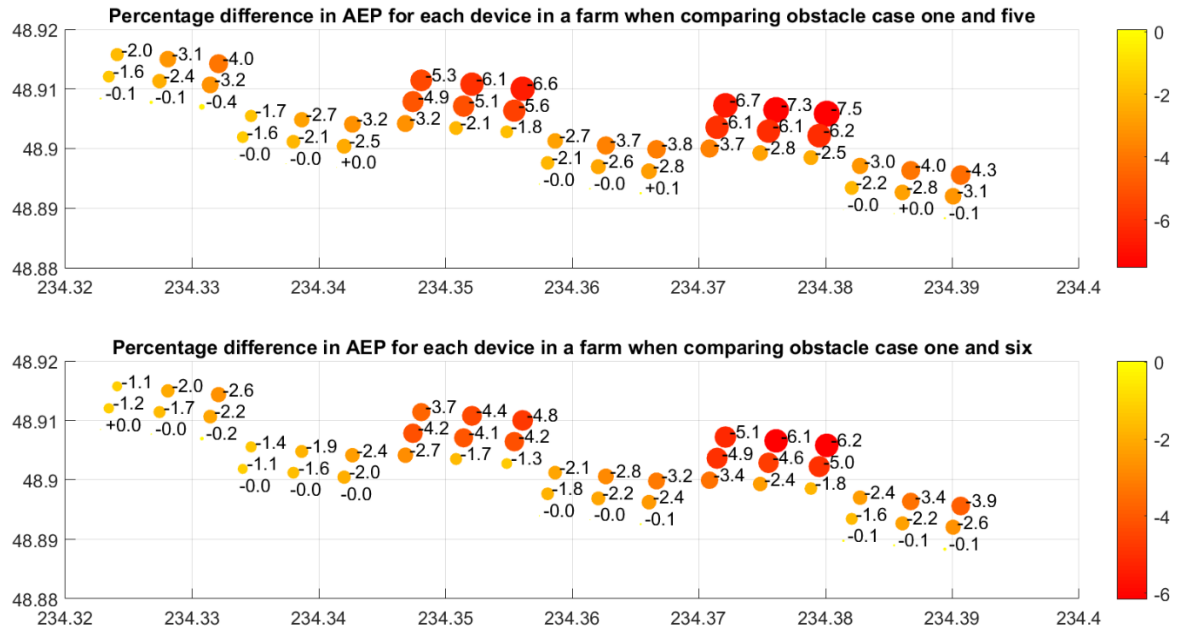
Figure 66: Percentage difference in annual energy production between obstacle cases one and five (top) and one and six (bottom)
