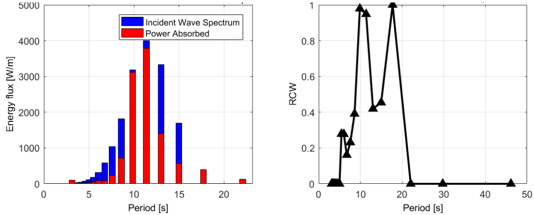
Figure 31: Power in a H_s = 1.75\text{m} and T_p = 11.1\text{s} sea state and power absorbed by the device overlayed on the left. RCW curve associated with this sea state on the right.
