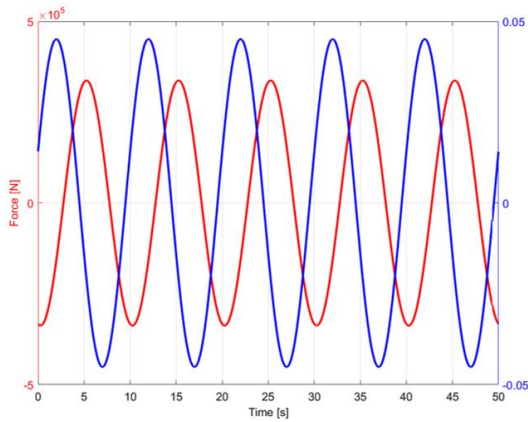
Figure 28: Force and velocity time series signal associated with a frequency of 0.1 Hz for a body in heave
