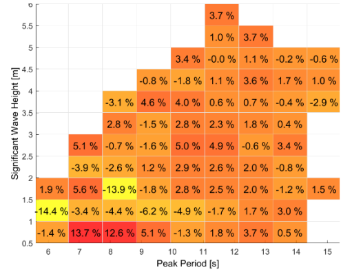
Figure 38: Difference in Spectral and Bulk Summation of the (P_{INC} - P_{RAD}) term of the Power Balance for each sea state modelled in the time domain
