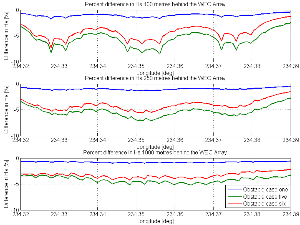
Figure 64: H_s interpolated at 100, 250 and 1000 metres in a high energy sea
