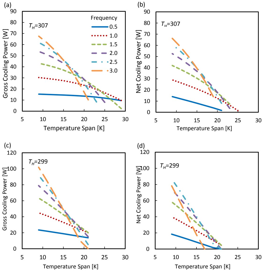
Fig. 22 Gross cooling power (a) and (c) and net cooling power (b) and (d) as a function of temperature span and frequency - (a) and (b) Hot side temperature is 307 K; (c) and (d) hot side temperature is 299 K. Displaced volume is 10.4 \text{ cm}^3 for all cases.
