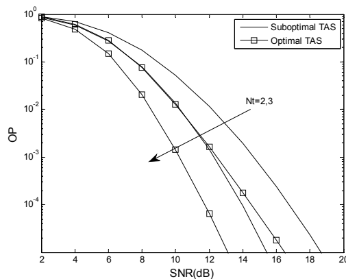
Figure 8. The OP performance of the optimal and suboptimal TAS schemes for different numbers of antennas N_t .
