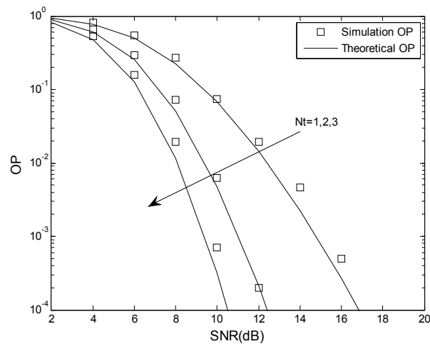
Figure 4. The OP performance of the optimal TAS scheme when \gamma_{th} < \gamma_P .
