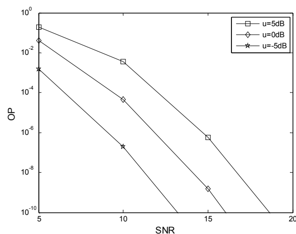
Figure 3. The effect of the relative geometrical gain \mu on the OP performance.
