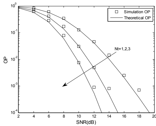
Figure 6. The OP performance of the suboptimal TAS scheme when \gamma_{th} < \gamma_P .
