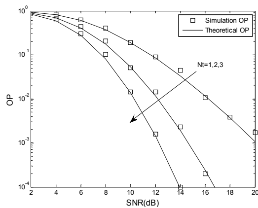
Figure 7. The OP performance of the suboptimal TAS scheme when \gamma_{th} > \gamma_P .
