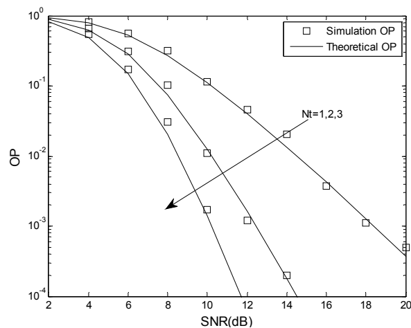
Figure 5. The OP performance of the optimal TAS scheme when \gamma_{th} > \gamma_P .
