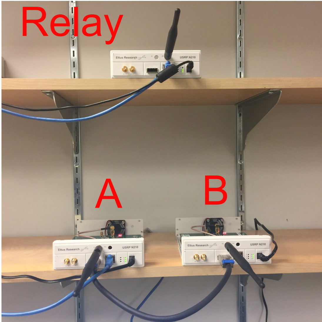
Figure 4.2: Testbed, two-hop scenario.
