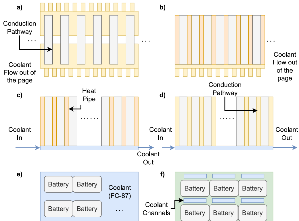
Fig. 3. Thermal management configurations analyzed in [47] (adapted).
