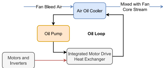
Fig. 15. Six passenger quadrotor TMS loop architectures. Source: Adapted from [61].
