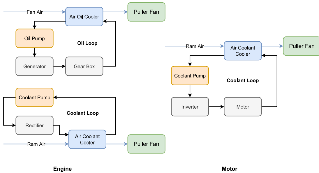
Fig. 10. RVLT tiltwing baseline TMS architecture. Source: Adapted from [55].
