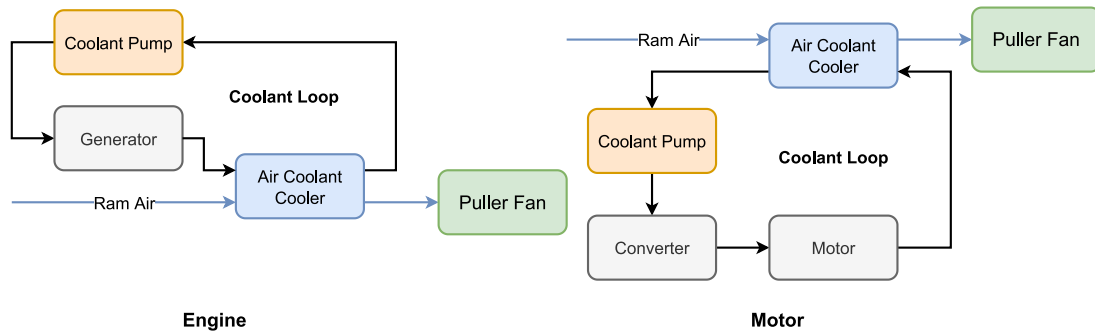
Fig. 11. RVLT tiltwing advanced technology TMS architecture. Source: Adapted from [55].
