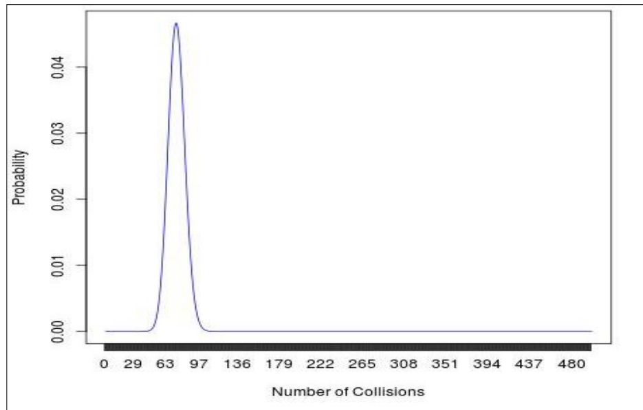
Figure 14. Poisson distribution with mobile photo radar present.
