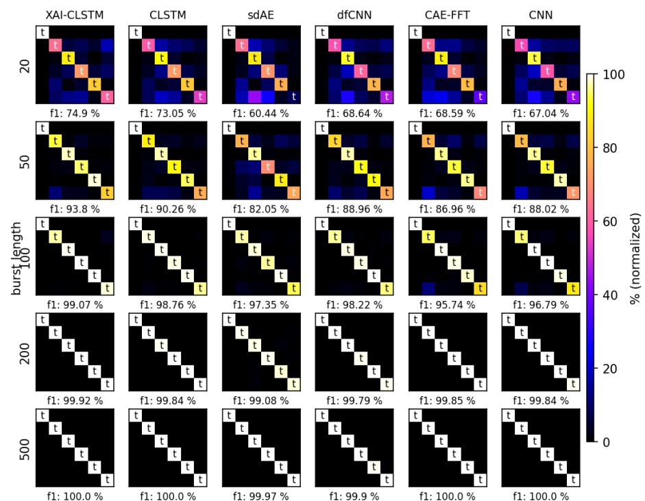
Figure 5. Classification performance comparison on CWRU dataset—t represents the correctly classified samples.
