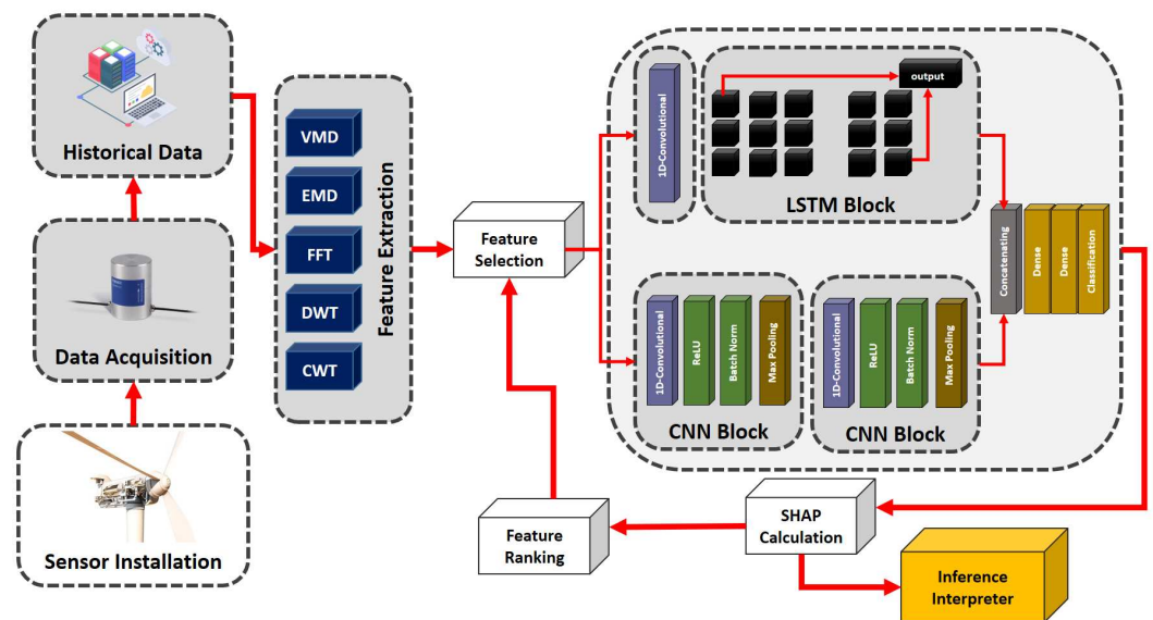
Figure 2. The suggested framework for XAI-based fault diagnosis.
