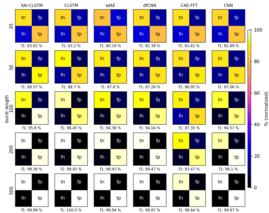
Figure 6. Classification performance comparison on wind turbine dataset—tn, fp, tp, and fn represent true negatives, false positives, true positives, and false negatives, respectively.
