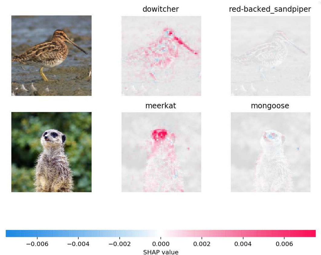
Figure 1. A demonstration of applying SHAP values in a computer vision task.
