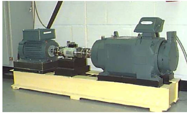
Figure 4. Two horsepower (left), a torque transducer and encoder (center), and a dynamometer (right) used to collect the dataset
