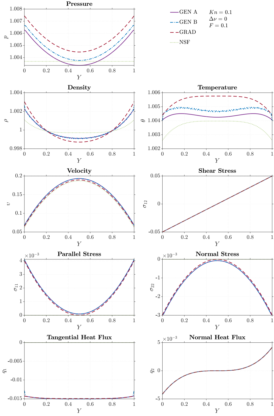
Figure 11. Poiseuille Flow for NSF, Grad-13, and GENERIC-13 at Kn = 0.1 , F = 0.1
