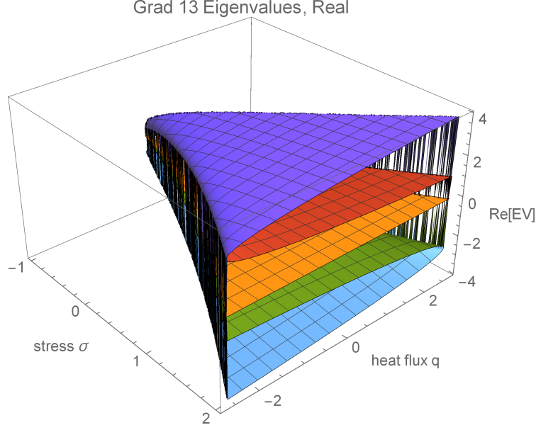
Figure 1. The eigenvalues \Lambda^\alpha for the Grad-13 matrix \mathcal{A}_{AB}^{\text{Grad}} for dimensionless variables. The eigenvalues are only shown where all are real, outside the plotted regions at least some of the \Lambda^\alpha are complex, and the Grad-13 equations lose hyperbolicity.
