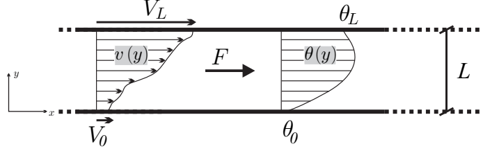
Figure 4. Geometry for steady-state plane flows between two parallel planes in distance L with prescribed boundary temperatures \theta_0 , \theta_L , velocities V_0 , V_L , and driving force F .
