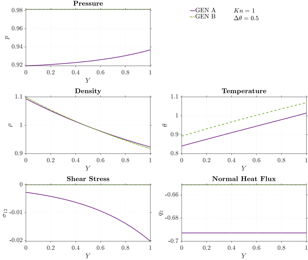
Figure 6. Heat Transfer for NSF and GENERIC-13 at Kn = 1 , \Delta\theta = 0.5 .
