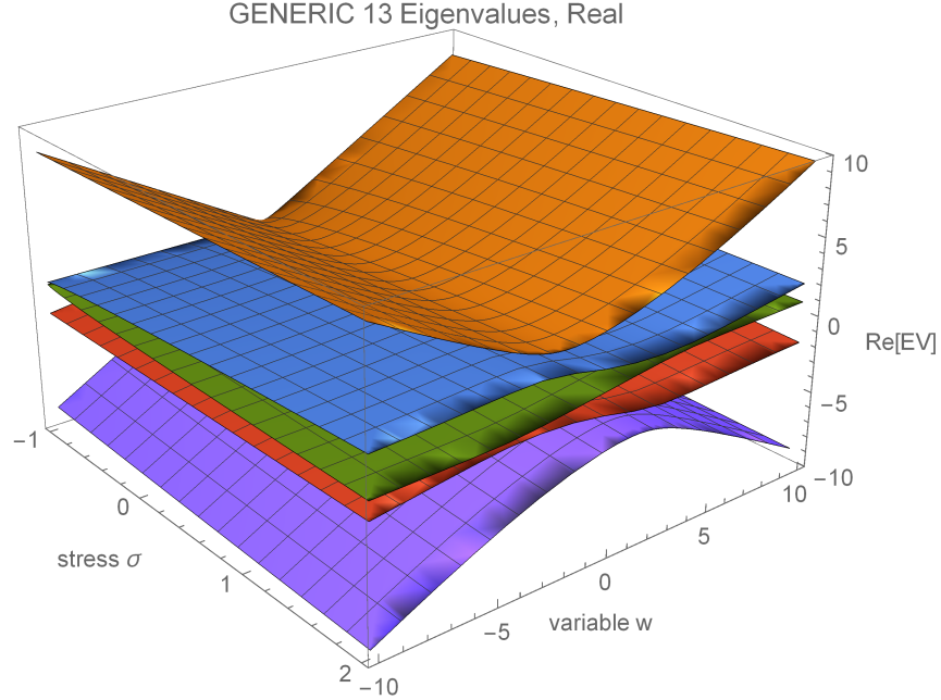
Figure 2. The eigenvalues \Lambda^\alpha for the GENERIC-13 matrix \mathcal{A}_{AB}^{\text{GEN13}} for dimensionless variables. All eigenvalues are real for all data.
