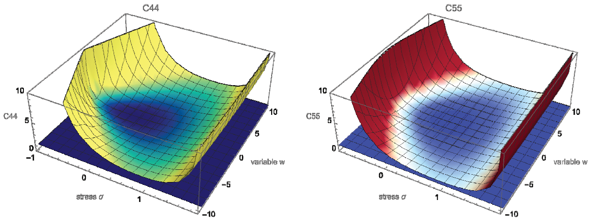
Figure 3. Damping factors C_{44} and C_{55} for GENERIC-13 and Grad-13 equations. While Grad-13 factors are constant, GENERIC-13 factors are non-linear with strong damping for processes far from equilibrium.
