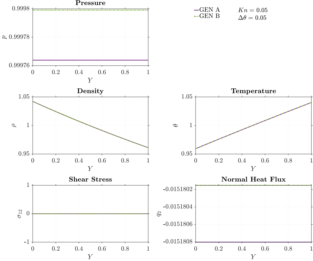
Figure 5. Heat Transfer for NSF and GENERIC-13 at Kn = 0.05 , \Delta\theta = 0.05 .
