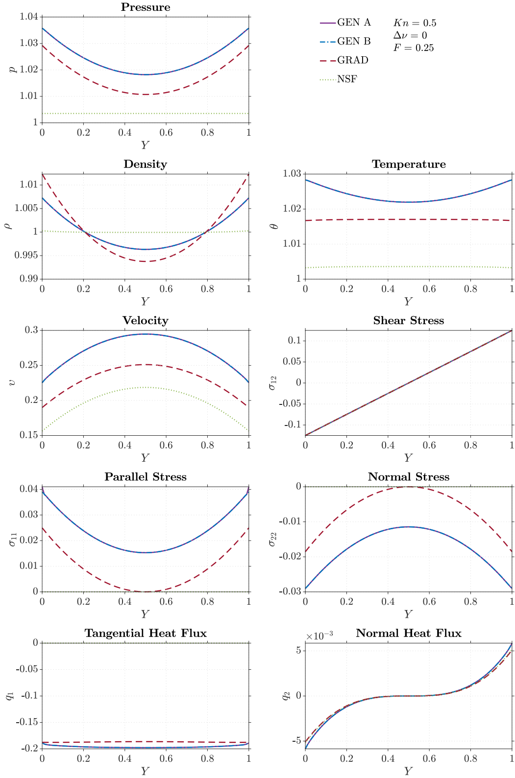
Figure 12. Poiseuille Flow for NSF, Grad-13, and GENERIC-13 at Kn = 0.5 , F = 0.25
