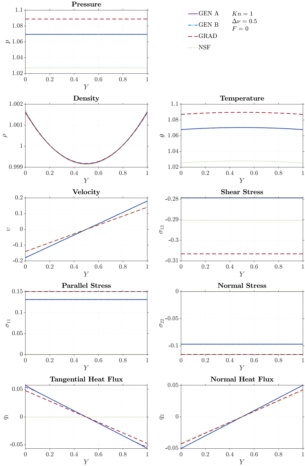
Figure 10. Couette Flow for NSF, Grad-13, and GENERIC-13 at Kn = 1 , \Delta v = 0.5
