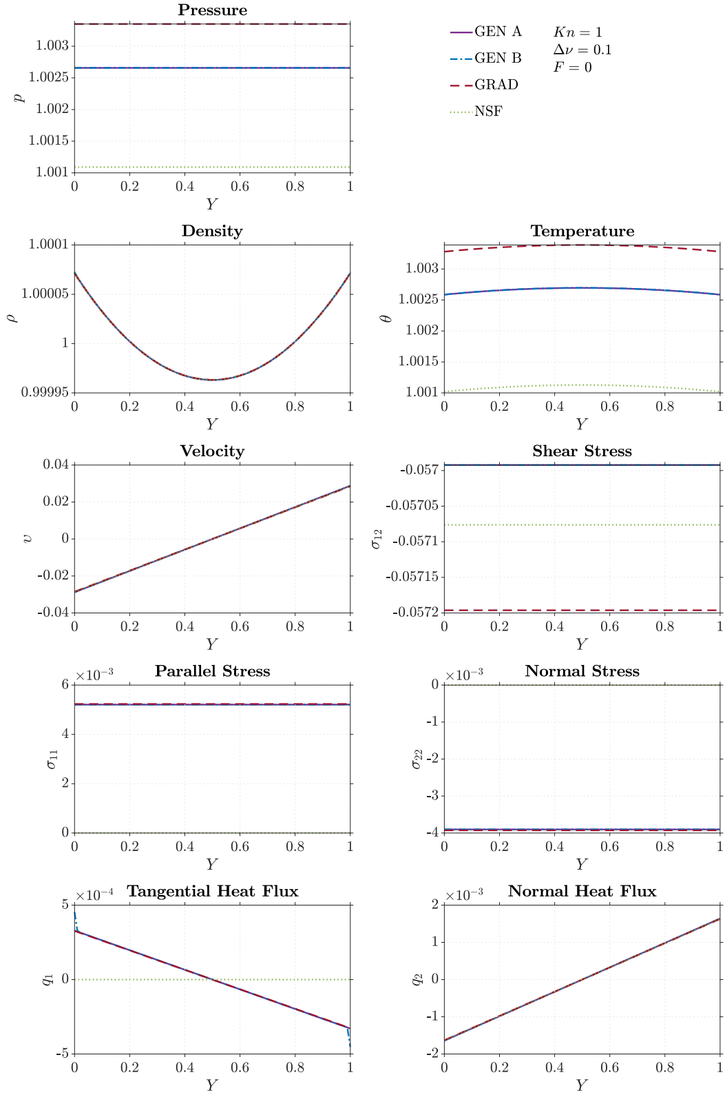
Figure 9. Couette Flow for NSF, Grad-13, and GENERIC-13 at Kn = 1 , \Delta v = 0.1
