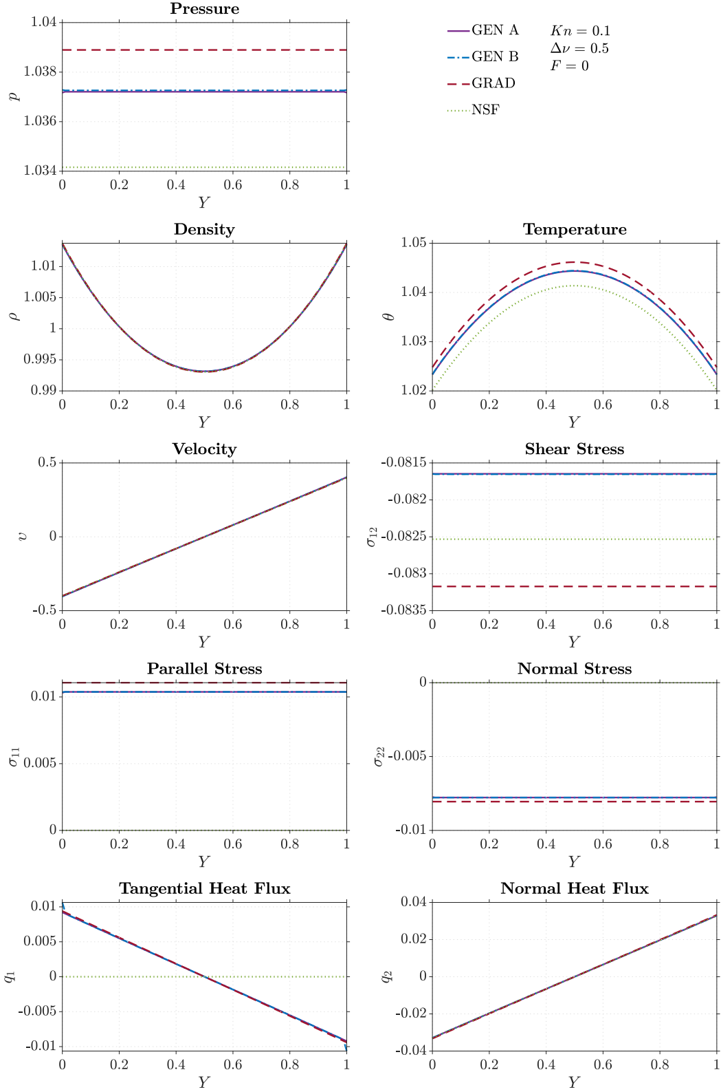
Figure 8. Couette Flow for NSF, Grad-13, and GENERIC-13 at Kn = 0.1 , \Delta v = 0.5
