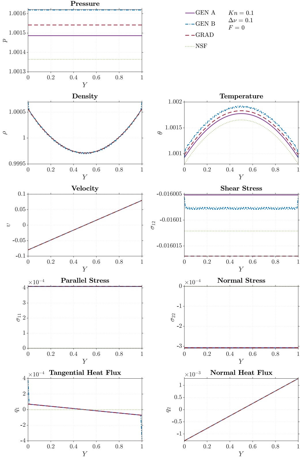
Figure 7. Couette Flow for NSF, Grad-13, and GENERIC-13 at Kn = 0.1 , \Delta v = 0.1
