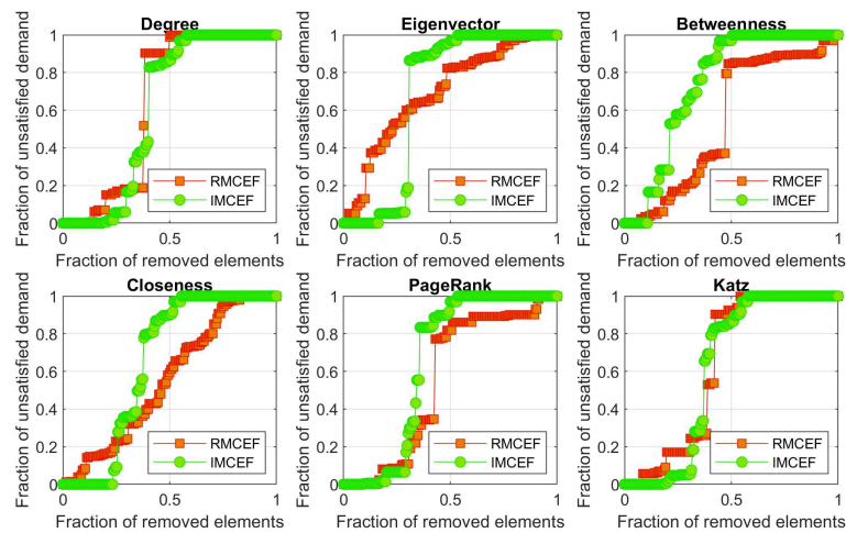
Figure 14. Vulnerability curves obtained from attacks on pipes with different centrality measures and attack sequences for the representative urban Saudi Arabian WDS.
