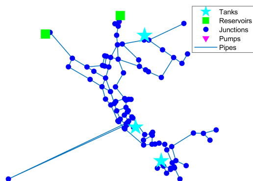
Figure 7. Network topology of the selected benchmarks (Net3).
