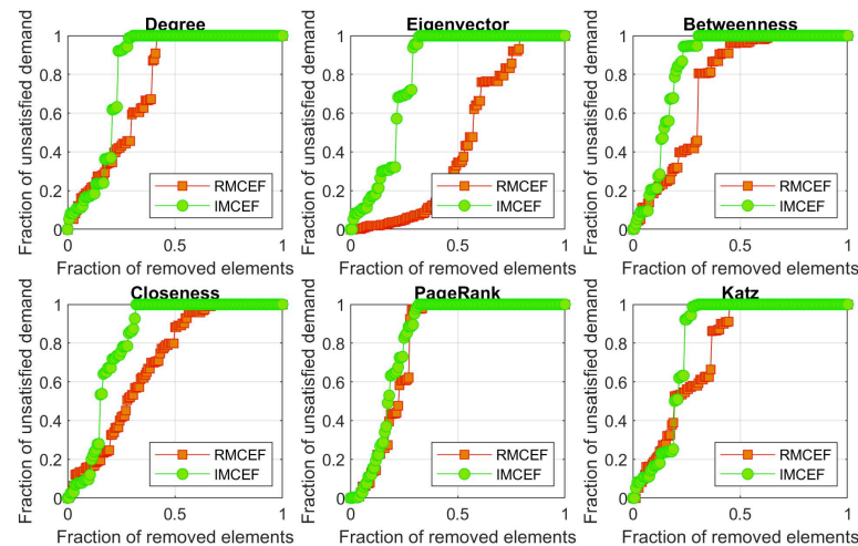
Figure 11. Vulnerability curves obtained from attacks on junctions with different centrality measures and attack sequences for the representative urban Saudi Arabian WDS.
