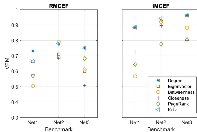
Figure 9. VPM through assaults using various fault methods and pipe removal.
