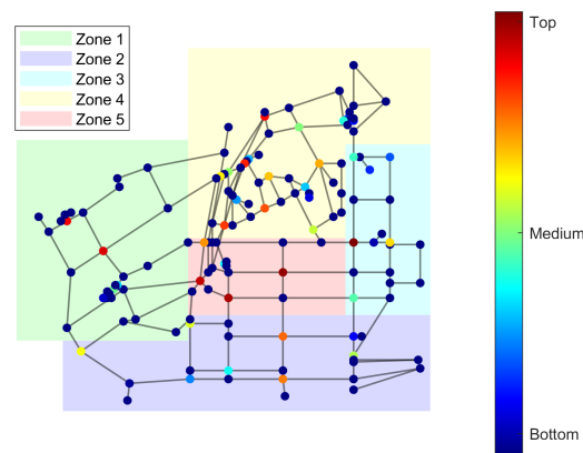
Figure 12. Zone definition and vulnerability ranking of junctions for the representative urban Saudi Arabian WDS.
