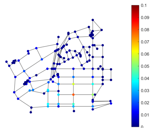
Figure 13. Ranking of junctions according to the normalised individual damage.
