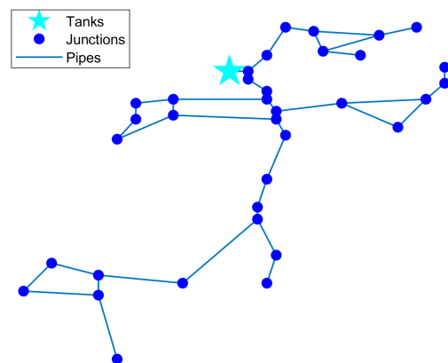
Figure 6. Network topology of the selected benchmarks (Net2).
