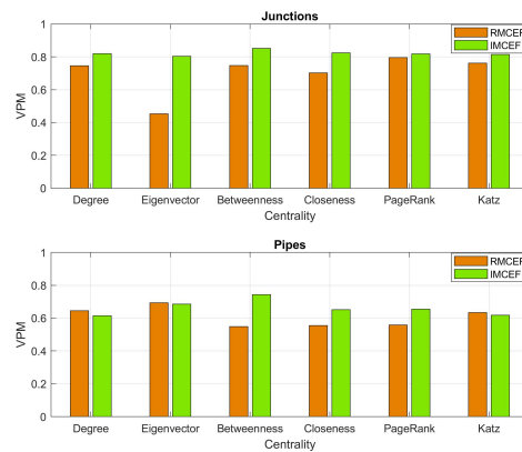
Figure 15. Summary of the VPM for the representative urban Saudi Arabian WDS.
