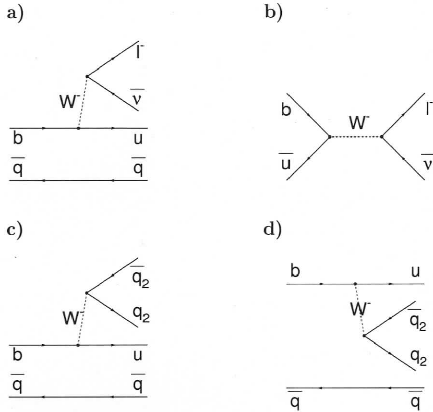
Figure 2.3: First order Feynman diagrams for the weak decay of a B meson ( b\bar{q} ) via different channels: a) semileptonic, b) leptonic, and c) and d) hadronic. The label q denotes a quark, l a lepton and \nu a neutrino.
