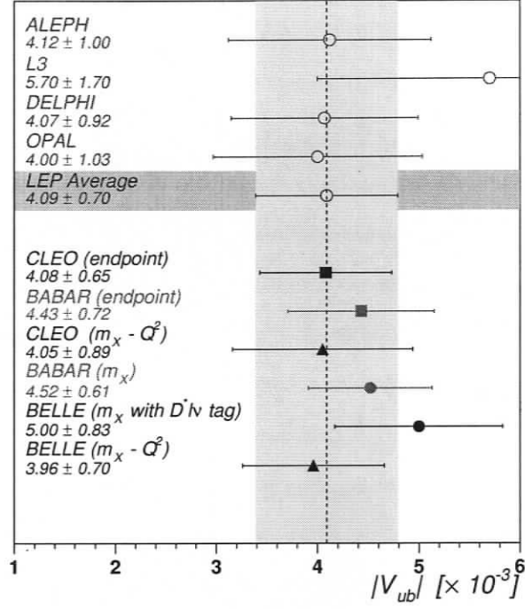
Figure 2.8: Status of |V_{ub}| measurements prior to this work (winter 2002 [19]). An additional 5% error must be added to the above results to account for the determination of |V_{ub}| from \mathcal{B}_u^{\text{SL}} (equation 2.35).
