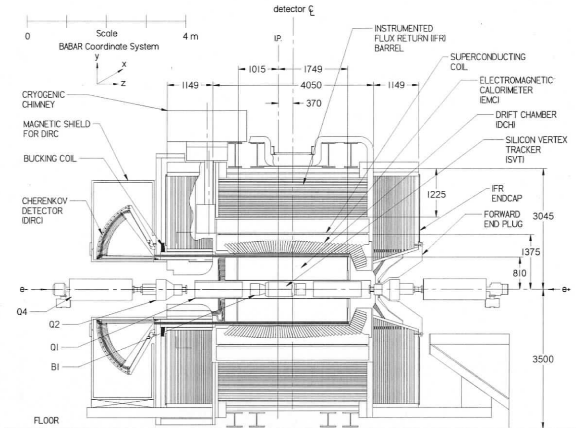
Figure 3.1: Longitudinal view of the BABAR detector. Unless referenced otherwise, all of the figures appearing in this chapter have been obtained from [44].
