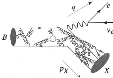
Figure 2.4: Higher order QCD interactions in a semileptonic B decay. Also represented are the kinematic variables used to describe B \rightarrow X e \bar{\nu}_e decays.
