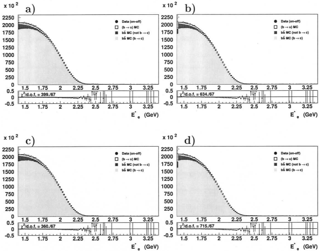
Figure 7.6: Effects of the uncertainty in simulating bremsstrahlung emission (top) and final state radiation (bottom) in terms of E_e^* . Shown are the 1- (left) and 1+ (right) cases. The above spectra should be compared with the nominal E_e^* spectrum displayed in figure 5.8.
