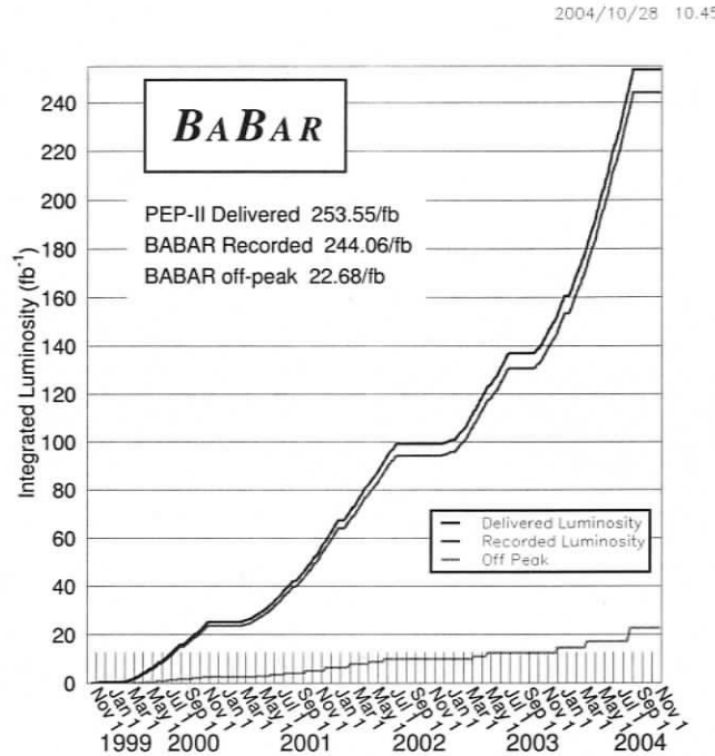
Figure 3.3: Integrated luminosity delivered by the PEP-II collider and recorded by the BABAR detector. Note that this analysis is based on Run-1 and Run-2 data taking periods (before November 2002), which contains about 88 million B\bar{B} pairs.
