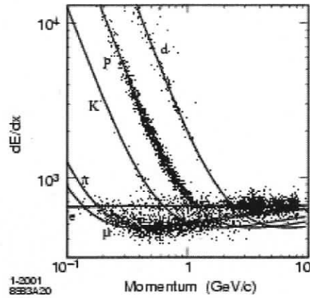
Figure 3.9: Particle identification via dE/dx measurements in the drift chamber [44].
