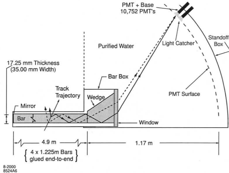
Figure 3.10: Schematic of the DIRC displaying a fused silica bar (grey), standoff box (white) and imaging region (dashed line) [44].
