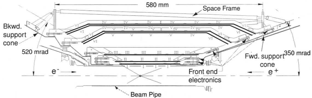
Figure 3.5: Longitudinal view of the upper half of the SVT. The outer layers have an arched structure to minimize the amount of silicon needed for the solid angle coverage and to reduce large incidence angles [44].
