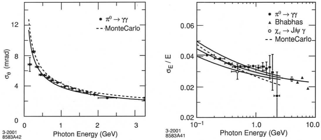
Figure 3.13: Electromagnetic calorimeter performance. The spatial (left) and energy (right) resolutions are plotted as a function of the incident photon energy [44].
