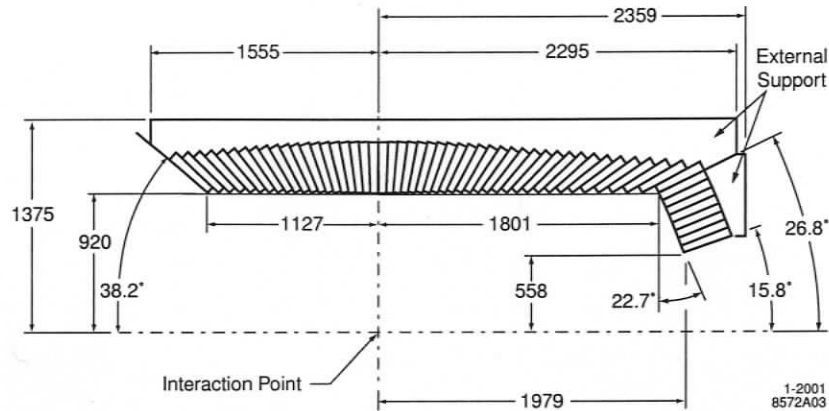
Figure 3.11: Longitudinal cross-section of the EMC showing the dimensions of the calorimeter barrel and forward endcap [44].
