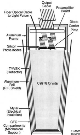
Figure 3.12: Schematic view of an EMC crystal assembly [44].
