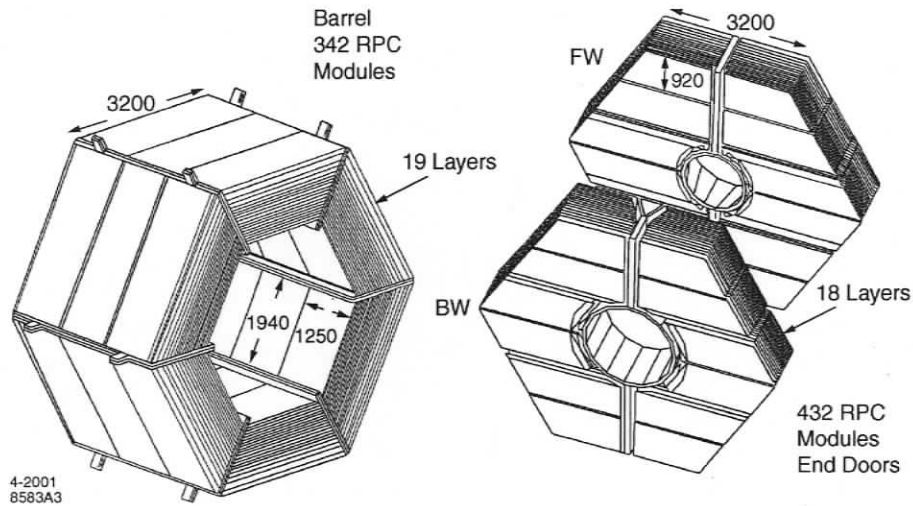
Figure 3.14: View of the IFR barrel and endcap wheels [44].
