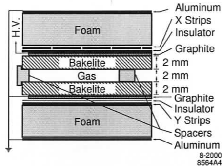
Figure 3.15: Cross-section of a RPC from the IFR [44].
