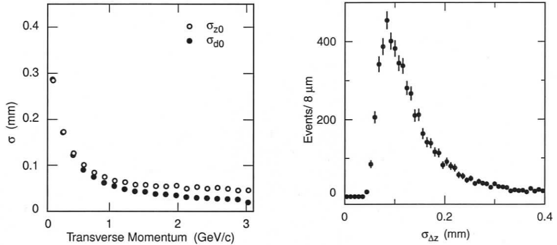
Figure 3.6: Resolution in the parameters d_0 and z_0 for tracks as a function of the transverse momentum (left), and error distribution for the measurement of the separation between two B meson decay vertices [45].
