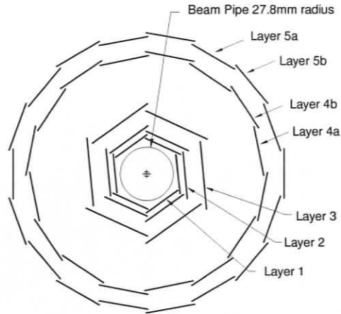
Figure 3.4: Cross-section of the SVT in a plane perpendicular to the beam axis ( x - y plane). The first layer radius is 3.3 cm, and the maximum fifth layer radius is 14.4 cm [44].
