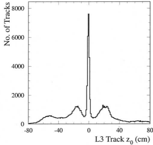
Figure 3.16: Distribution of z_0 for tracks satisfying the L1 trigger as reconstructed by L3 [44].
