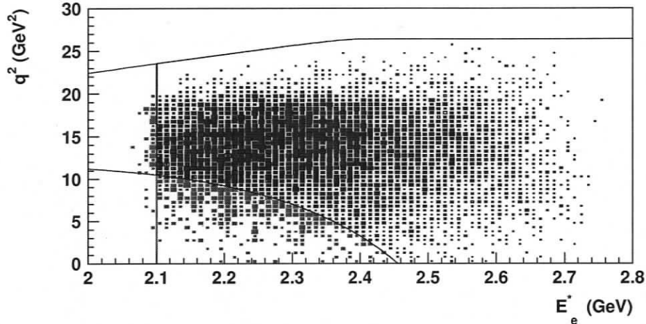
Figure 7.1: Generated B \rightarrow X_u \ell \bar{\nu}_\ell events which have been reconstructed in the q^2 - E_e^* signal region. As can be seen, events generated outside the signal (target) region may feed into the signal region due to poor E_e^* or, more likely, q^2 reconstruction.
