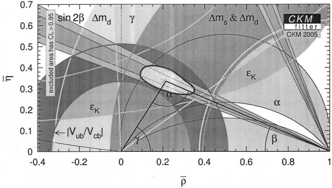
Figure 2.2: Status of CP violation with respect to the Standard Model [20]. The unknown apex (\bar{\rho}, \bar{\eta}) of the unitarity triangle is located in the ellipse-like shaded area. It is primarily constrained by the measurements of \sin 2\beta and |V_{ub}/V_{cb}| .
