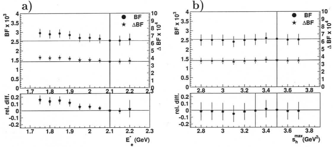
Figure 8.1: Changes in the B \rightarrow X_u e \bar{\nu}_e branching fraction measurement (solid points) as a function of a) the lower bound on E_e^* and b) the upper bound on s_h^{\max} . The behavior of the partial branching ratio is also displayed (stars) and the appropriate scale is provided on the right hand side of the plots. The lower plots display the relative difference with respect to the nominal requirements: \mathcal{B}_u^{\text{SL}}(E_e^* > x)/\mathcal{B}_u^{\text{SL}}(E_e^* > 2.1 \text{ GeV}) - 1 , and \Delta\mathcal{B}_u^{\text{SL}}(E_e^* > x)/\Delta\mathcal{B}_u^{\text{SL}}(E_e^* > 2.1 \text{ GeV}) - 1 . The errors shown are purely statistical.
