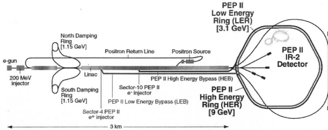
Figure 3.2: Schematic view of the linear accelerator and PEP-II collider at SLAC [44].
