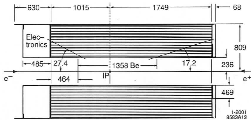
Figure 3.7: Longitudinal cross-section of the DCH [44].
