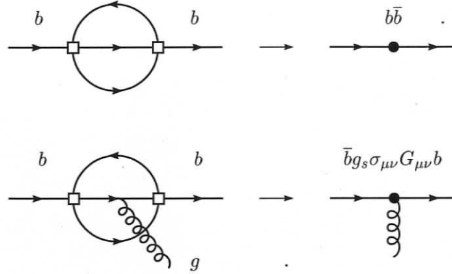
Figure 2.5: Perturbative contributions to the transition operator (left) and the corresponding operators in HQE [31].
