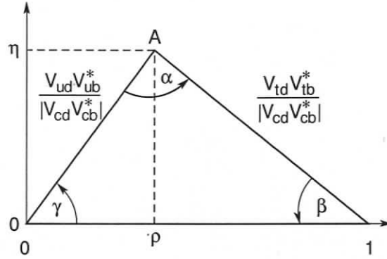
Figure 2.1: The rescaled unitarity triangle. The phase convention is such that V_{cd}V_{cb}^* is real.
