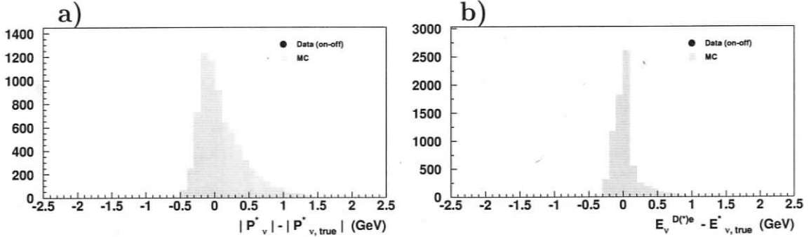
Figure 6.7: Resolution plots using the simulation for the two neutrino estimators, a) |\vec{P}_\nu^*| - |\vec{P}_{\nu,true}| and b) E_\nu^{D^{(*)}e} - E_{\nu,true} for the D^0 e \bar{\nu}_e X control sample for events satisfying the refined selection defined in section 5.5 (but not s_h^{\max} ).
