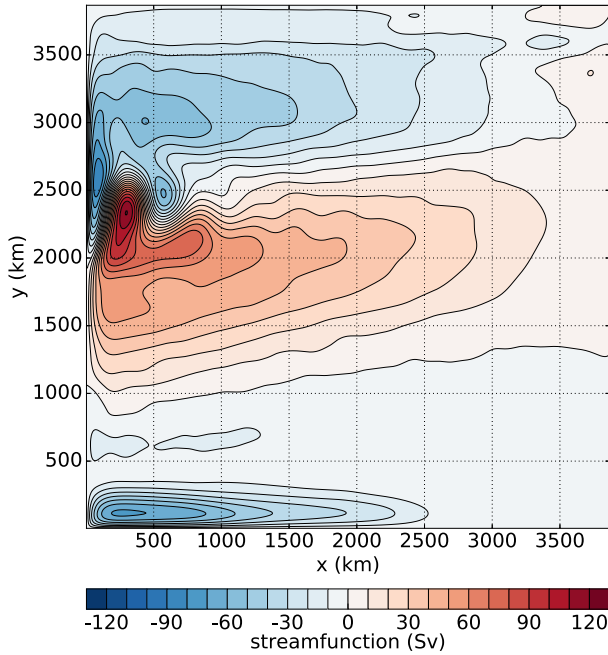
Fig. 3. Time-mean barotropic streamfunction in the idealized primitive equations model using days 3500–7210 ( \approx 10 years of data) sampled at 10-day intervals. Red is clockwise circulation, blue counterclockwise. (For interpretation of the references to colour in this figure legend, the reader is referred to the web version of this article.)
