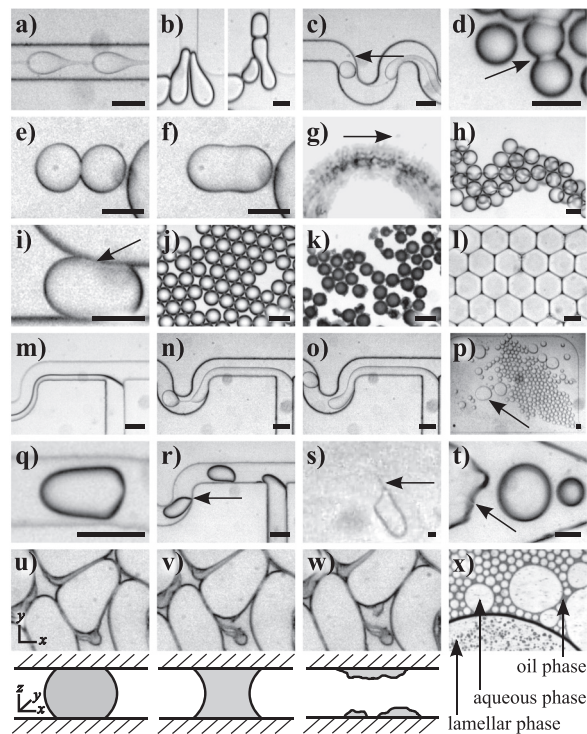
FIG. 5. Images of droplet failure modes. Failure modes caused by shear forces and interfacial tension: (a) beading, (b) droplet splitting, and (c) satellite droplet formation. Failure modes that occur due to surfactant effects in flow: (d) DIB formation, (e) and (f) droplet merging, (g) micelle formation, (h) non-permanent droplet adhesion, and (i) surfactant-monomer interactions. Failure modes that occur due to surfactant effects during storage: (j) and (k) budding and (l) raft-driven droplet deformation. Droplet failure modes caused by wetting and surface affinity in flow: (m) co-flow, (n) and (o) dripping mode, (p) localised adhesion, (q) generalised substrate-driven droplet deformation, (r) localised substrate-driven droplet deformation, (s) tip-streaming, and (t) wetting. Droplet failure modes caused by wetting and surface affinity during storage: (u)–(w) substrate-driven droplet spreading (sequential images were taken over the course of approximately 30 min), with a schematic representation of the cross-sectional view through the channel below. (x) Tertiary phase formation occurs due to the phase properties of the droplet system during droplet storage. Arrows highlight the failure modes and scale bars are approximately 50 \mu\text{m} . For experimental details and videos, see the supplementary material. 28
