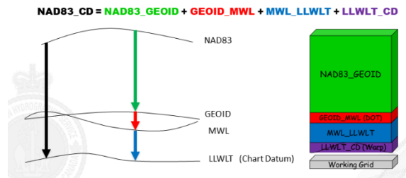
Figure 66-1. (left) Summary of vertical layers making up the NAD83-CD HyVSEP. (Right) Operational NAD83-CD HyVSEP surface for 2022.
