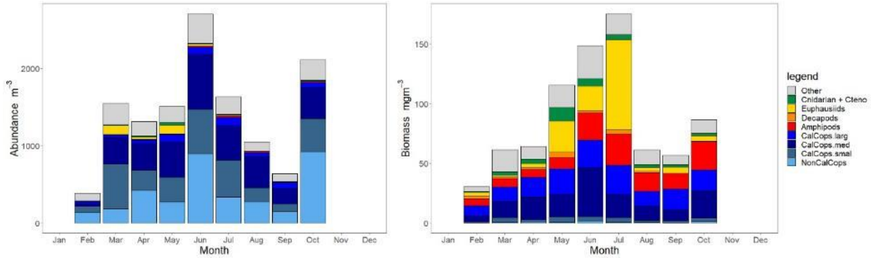
Figure 43-4. Taxonomic composition of zooplankton from northern and central Strait of Georgia in 2022, averaged by month. Left: abundance ( m^{-3} ); Right: biomass ( mg\ m^{-3} ). Legend: CalCops.larg – calanoid copepods, prosome length (PL)>3mm; CalCops.med – calanoid copepods PL 1-3mm; CalCops.small – calanoid copepods PL <1mm; NonCalCops – all other copepods; Amphipods – all amphipods (hyperiid and gammarid); Decapod – all decapods (shrimp, crab larvae); Euphausiid – all euphausiids (eggs, larvae and adults); Cnidarian + Cteno – all Cnidarian (medusa and siphonophores) and Ctenophores; Other – everything else: Molluscs, Polychaetes, Chaetognaths, Ichthyoplankton, Larvaceans, etc.
