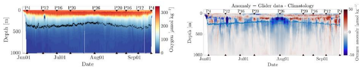
Figure 13-4. Transect of ocean glider oxygen concentration along Line P from P4 to OSP between May and September 2022 as a function of depth and time (left). The black dots show the 60 μmol/kg surface, indicating the hypoxic boundary and the approximate top of the OMZ. Oxygen anomaly along the same transect (right). The blue dots show the location of the 1026.7 kg/m 3 isopycnal.
