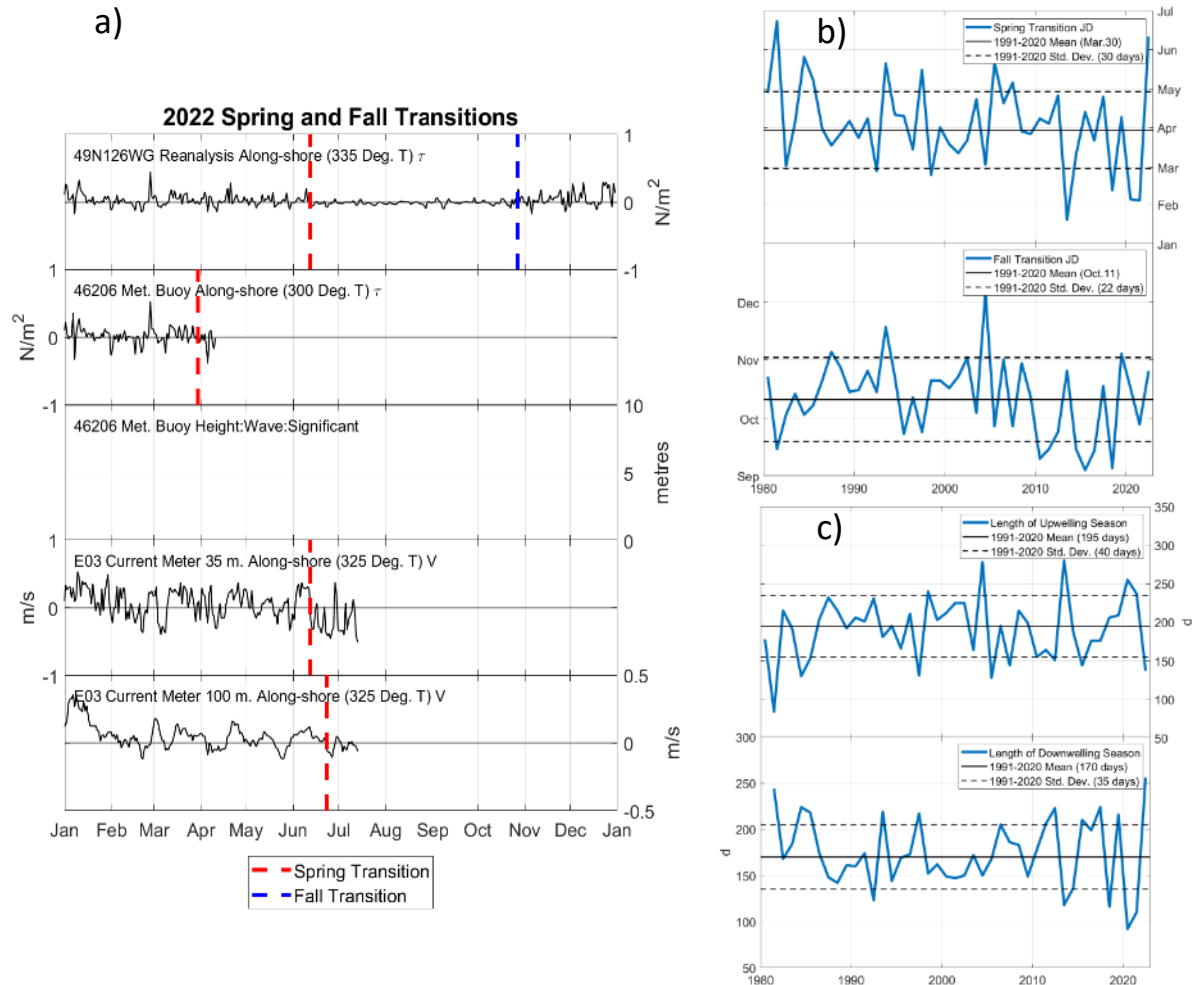
Figure 8-2. (a) Time series depicting the Spring and Fall Transitions off the West coast of Vancouver Island in 2022. Wind stress at Reanalysis-1 grid point 49°N 126°W and meteorological buoy 46206; significant wave height at 46206; along-shore current velocity at 35 and 100 m depth at mooring E03 (Folkes et al. 2017; Thomson et al. 2013). Positive flow is poleward (downwelling-favourable) and negative flow is equatorward (upwelling-favourable). Vertical dashed lines show derived transition times using a cumulative sum approach (e.g., Foreman et al. 2011). (b) The annual Spring and Fall Transitions derived from time series in panel a. (c) The length of the upwelling and downwelling seasons derived from the time series in panel b.
