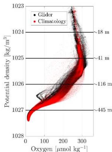
Figure 13-2. Ocean glider oxygen concentrations along Line P from P4 to OSP between May and September 2022 (black dots) as a function of potential density, compared to a climatology linearly interpolated to the same sampling locations and days of year (red dots). Average isopycnal depths are indicated.
