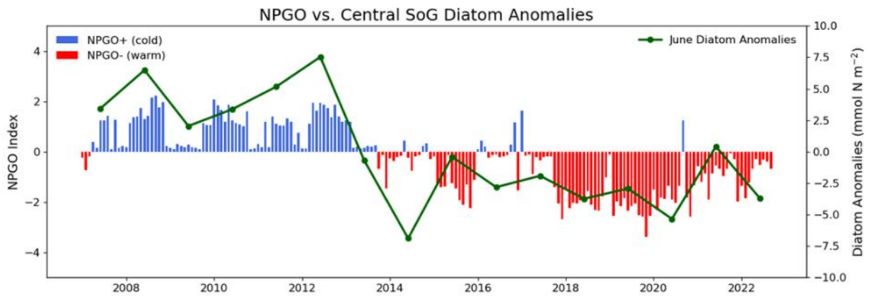
Figure 41-2. NPGO time series (bars) versus diatom biomass anomalies (line) in the Central SoG in June. Note the strong correlation.
