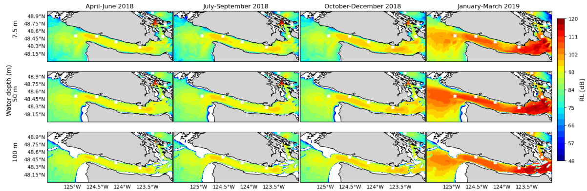
Figure 49-2. Vessel noise additions at 125 Hz for commercial Class A vessels transiting the study area as obtained from the shipping noise model. Comparisons were made for median noise levels ( L_{50} ) for 3-month periods, and for water depths 7.5 m, 50 m, 100 m.
