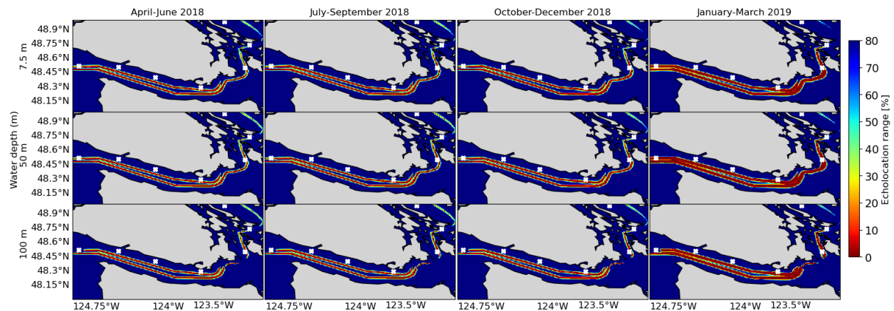
Figure 49-5. Proportional reduction, due to vessel noise, of 50 kHz signal range from 'minimum ambient' conditions representing echolocation use by SRKW. Comparisons were made for 3-month periods, with whale at 10 m echolocating on Chinook salmon prey at depths of 7.5 m, 50 m, 100 m.
