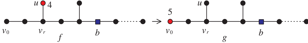
Figure 6: A step in the proof of Lemma 5.1.
