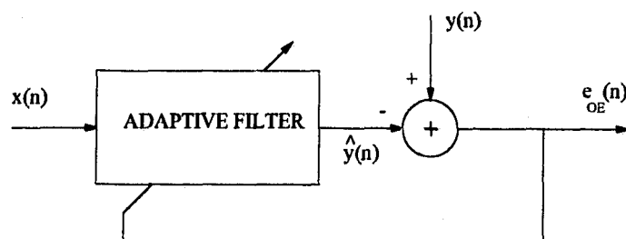
Figure 1.2: Block diagram of a general adaptive system.
