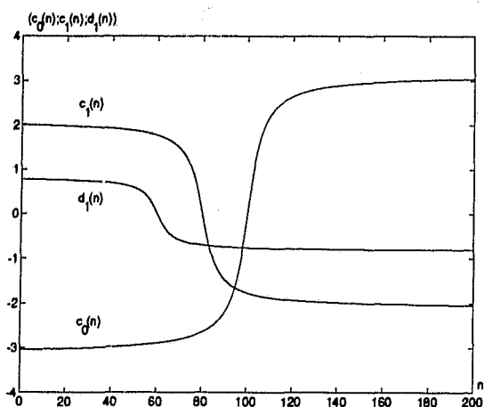
Figure A.1: Example A.18 - Time-varying coefficients c_0(n) , c_1(n) , and d_1(n) , with s = 0.2 .
