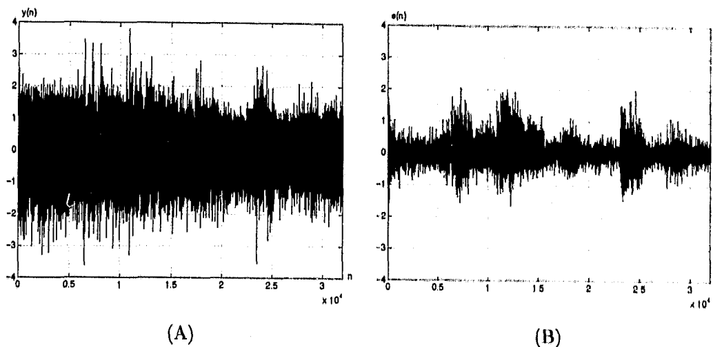
Figure 5.3: Noise cancellation example using the LMS algorithm with \mu = 0.003 and N = 300 : (A) Original reference signal (B) Resulting error signal.
