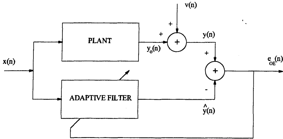
Figure 1.3: Block diagram of an adaptive system identifier.
