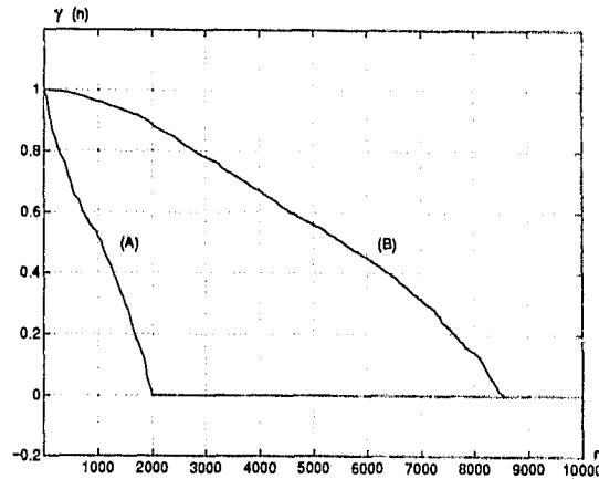
Figure 3.4: Example 3.9 - Convergence in time of the time-varying composite parameter: (A) \hat{\theta}(0) = [0.8 \ 0.3]^T ; (B) \hat{\theta}(0) = [0.0 \ -0.3]^T .
