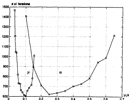
Figure 3.1: Example 3.5 - Number of iterations required for the CSE signal averaged over 50 experiments to reach -200\text{dB} as a function of \mu in the fixed convergence factor case ('o') and \alpha in the variable convergence factor case ('x'), for the SD-CSE algorithm.
