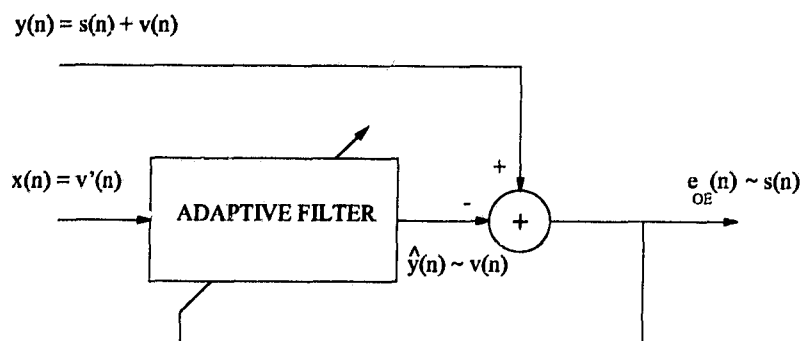
Figure 5.1: Block diagram of an adaptive noise canceller.
