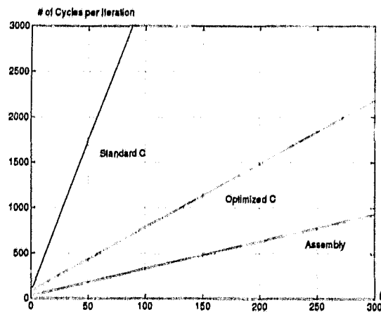
Figure 5.2: Number of cycles per iteration \times filter order for the off-line LMS algorithm using standard C, optimized C, and assembly languages.
