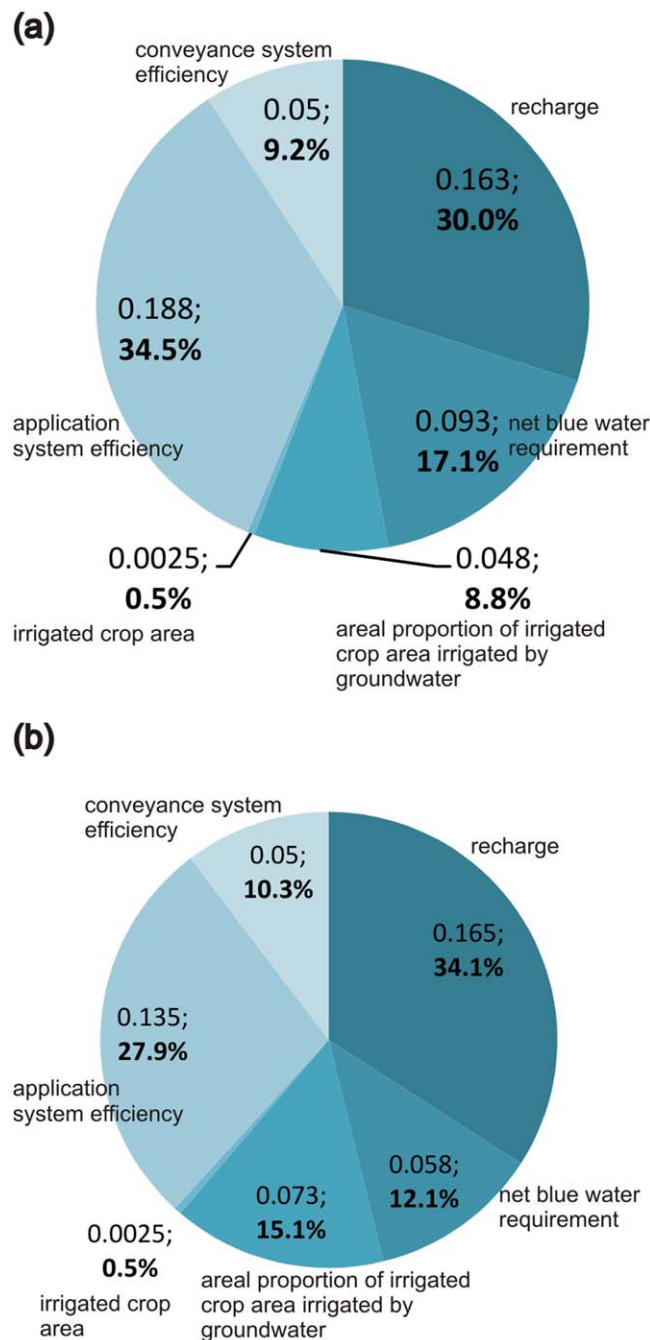
Figure 2. Contribution of parameter uncertainty to total relative uncertainty for (a) the Central Valley and (b) High Plains aquifer systems. The first value indicates the actual value of the relative uncertainty of the parameter in the aquifer system and the second value (% in bold) indicates the relative contribution of this uncertainty to the total relative uncertainty in the aquifer system.
