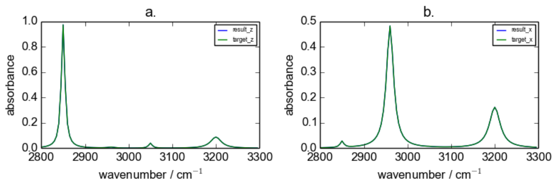
Figure 3.5: IR spectra plotted by the return compositions from the constraint study based on Case 4 of simplified molecular model. a. z -polarized IR spectra; b. x -polarized IR spectra.
