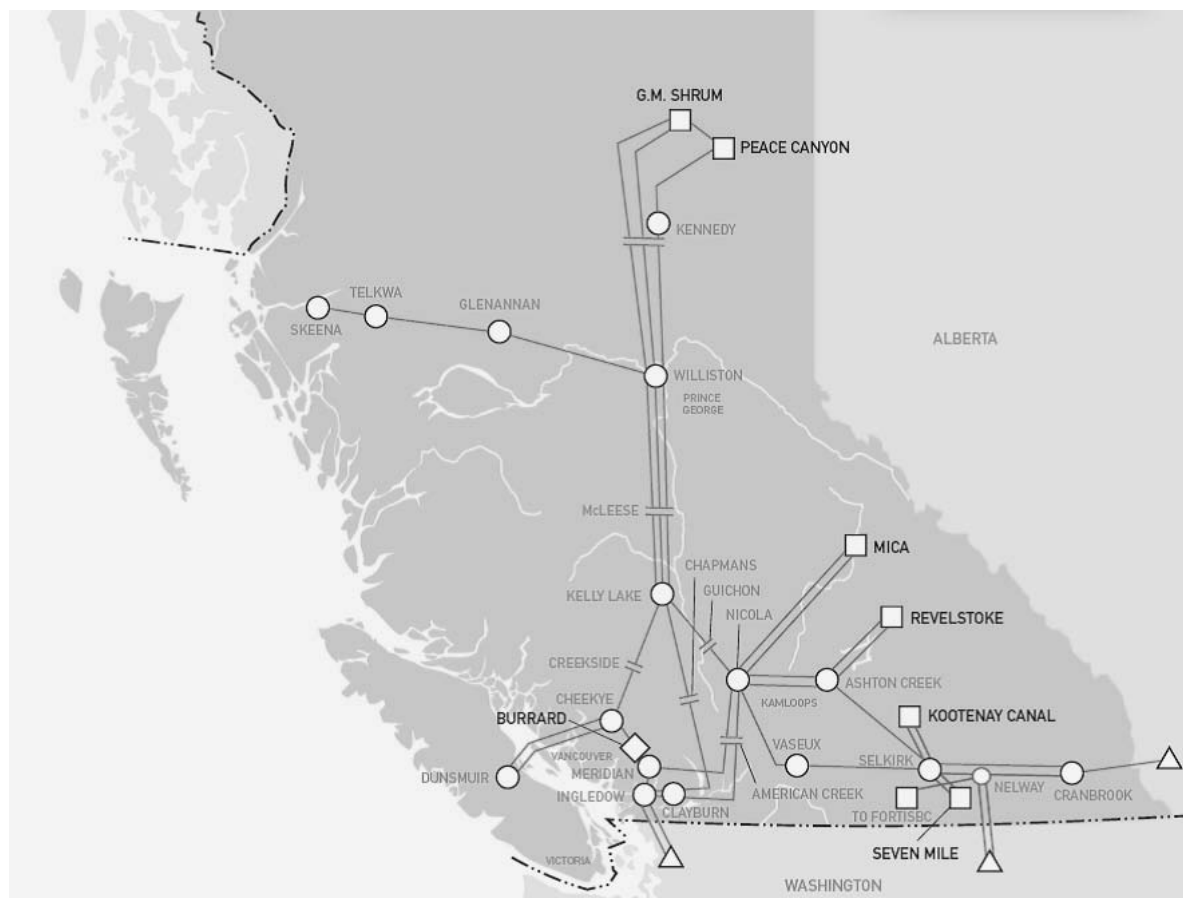
Figure 2.8: Map of BC's transmission grid and connected generators.
