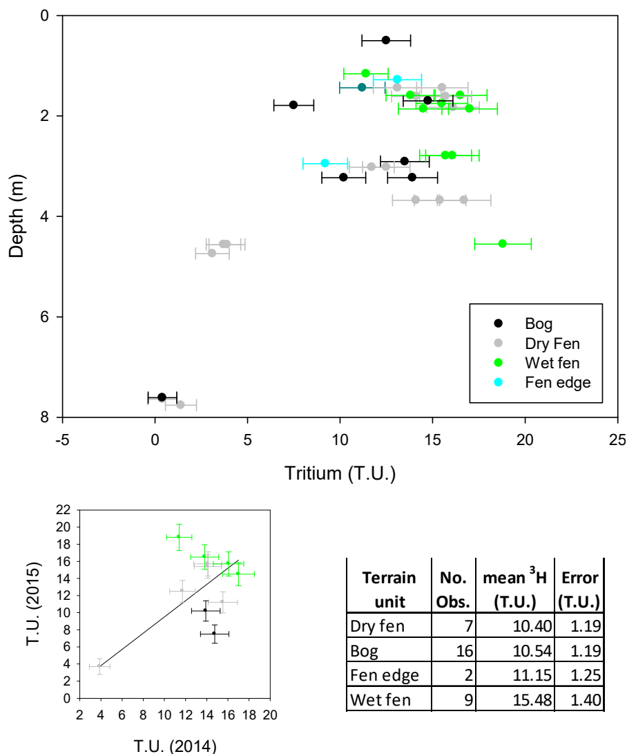
Figure 7. Tritium variations with depth at ML for various terrain units. Inset shows comparison of tritium measured in 2015 versus 2014. Averages for each terrain unit are tabulated and presented in order of increasing rates of turnover or hydrologic intensity.
