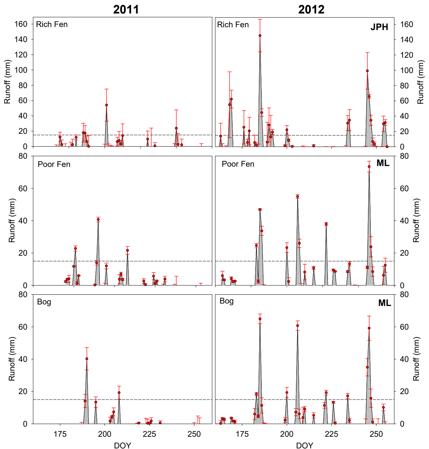
Figure 4. Time series of 2011 and 2012 runoff potential as estimated by vertical water balance for selected terrain units at ML and JPH sites. Red points denote individual daily values, error bars show 1 standard deviation of uncertainty. Dashed lines indicate detention storage capacity thresholds estimated from LiDAR surveys.
