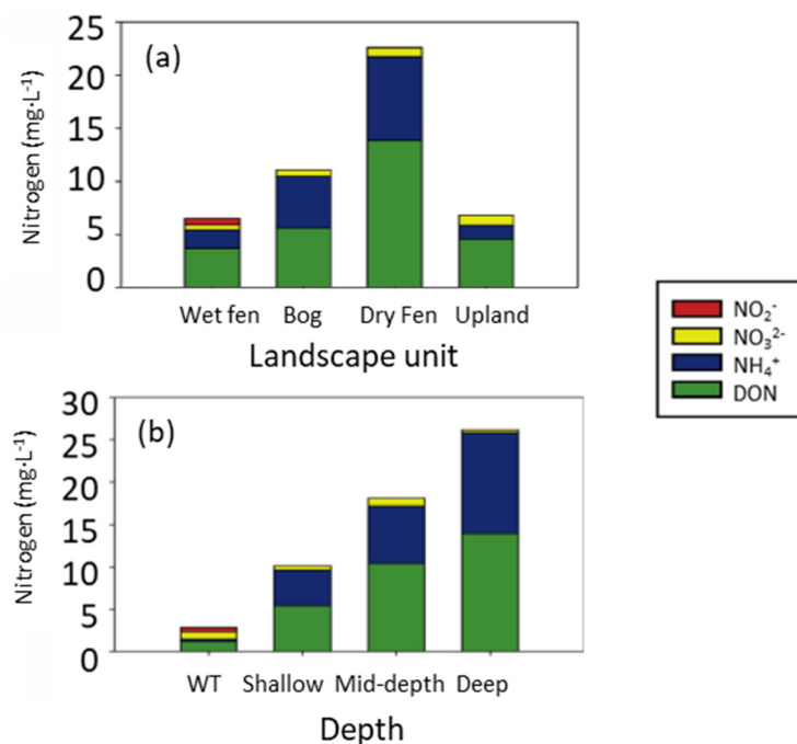
Figure 9. Summary of average nitrogen concentrations observed at ML by (a) landscape unit and (b) depth (modified after [25]).
