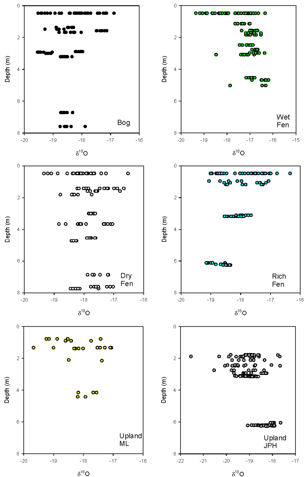
Figure 6. Depth-wise variations in \delta^{18}\text{O} in various terrain units: bog, wet fen, and dry fen (ML), rich fen (JPH), upland (ML), and upland (JPH). Seasonal variability is shown to be greater for near-surface soil water. Note that 10 highly-enriched water table well samples that were evidently sourced by brief summer precipitation events were not included.
