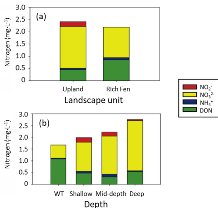
Figure 8. Summary of average nitrogen concentrations observed at JPH by (a) landscape unit and (b) depth (modified after [25]).
