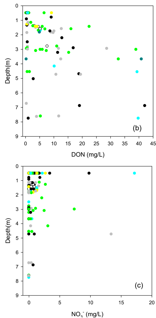
Figure 10. Distribution of major nitrogen species concentrations with depth at ML for individual samples, (a) \text{NH}_4^+ , (b) DON and (c) \text{NO}_3^- . Wetland terrain units are colour-coded. Upland is shown in yellow.
