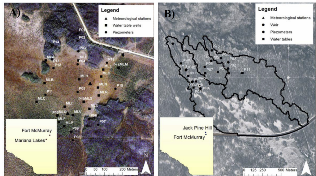
Figure 2. Location of instrumentation installed at (A) ML and (B) JPH. Note the scale differences in (A,B). Colours at ML depict uplands (purple), bogs (green), and fens (brown). Outlines at JPH depict delineated drainage areas including the rich fen (unit located to the southwest) and upland terrain units.
