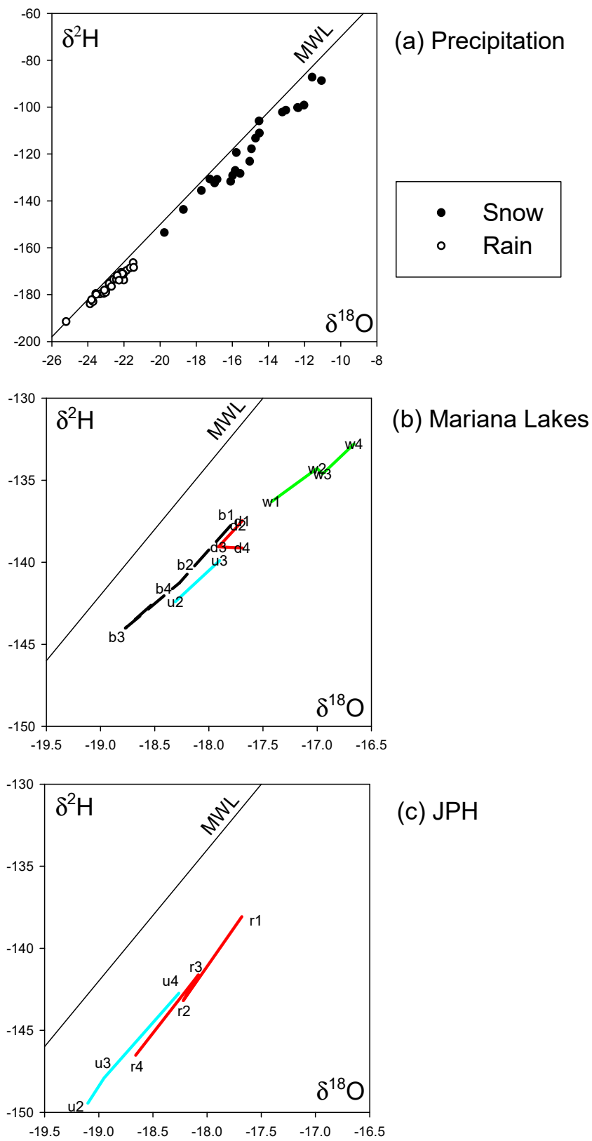
Figure 5. Isotopic composition of (a) precipitation (snow and rain), and average isotopic composition of water table wells, and shallow to deep piezometers (b) Mariana Lakes, and (c) Jack Pine High. Note that b—bog, d—dry fen, w—wet fen, r—rich fen, u—upland; 1—water table, 2—shallow piezometers, 3—intermediate piezometers, 4—deep piezometers.
