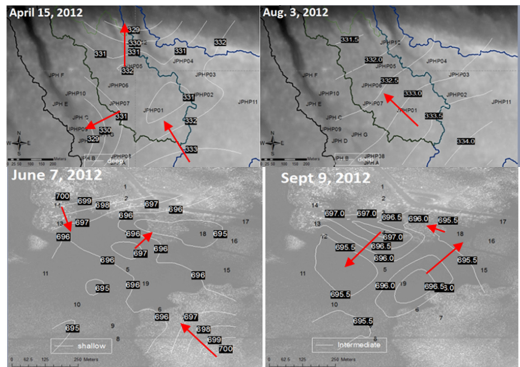
Figure 3. Maps showing hydraulic head elevations and inferred flow directions: for JPH ( top left ) April 2012, ( top right ) August 2012; and, for ML ( bottom left ) June 2012, and ( bottom right ) September 2012.
