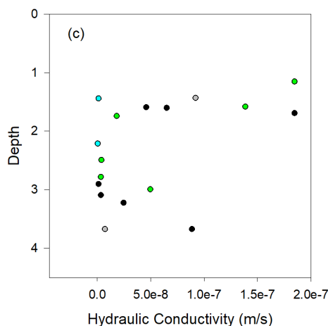
Figure 11. Plots of (a) nitrate and (b) ammonium species versus hydraulic conductivity ( \text{m}\cdot\text{s}^{-1} ) and (c) depth versus hydraulic conductivity for ML wetlands. Terrain units are colour-coded. Error bars represent 1 standard deviation of measurements. Note that hydraulic conductivity and depth were one-time determinations.
