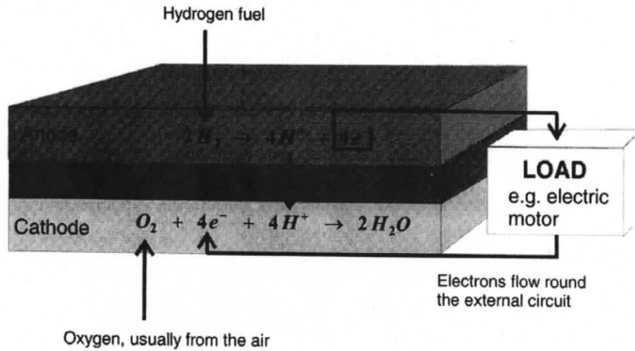
Figure 1.1: Hydrogen-Oxygen Fuel Cell Diagram [1].
