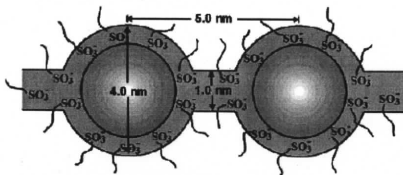
Figure 1.6: Cluster-network model [6].
