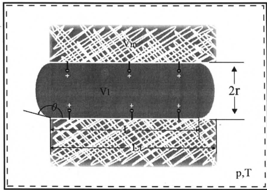
Figure 2.1: Cylindrical Pore System.
