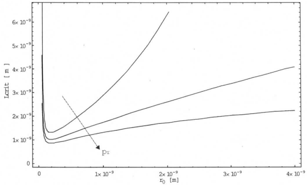
Figure 3.5: Critical Length vs r_0 ( p_r = 0.8 : 1.2 ) - Cylindrical Pore.
