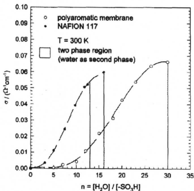
Figure 1.5: Conductivity vs Water Content [18].
