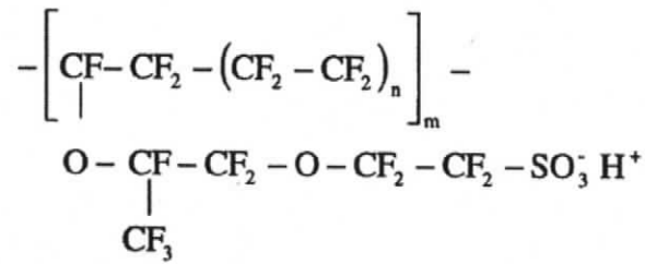
Figure 1.2: Nafion chemical structure [4].
