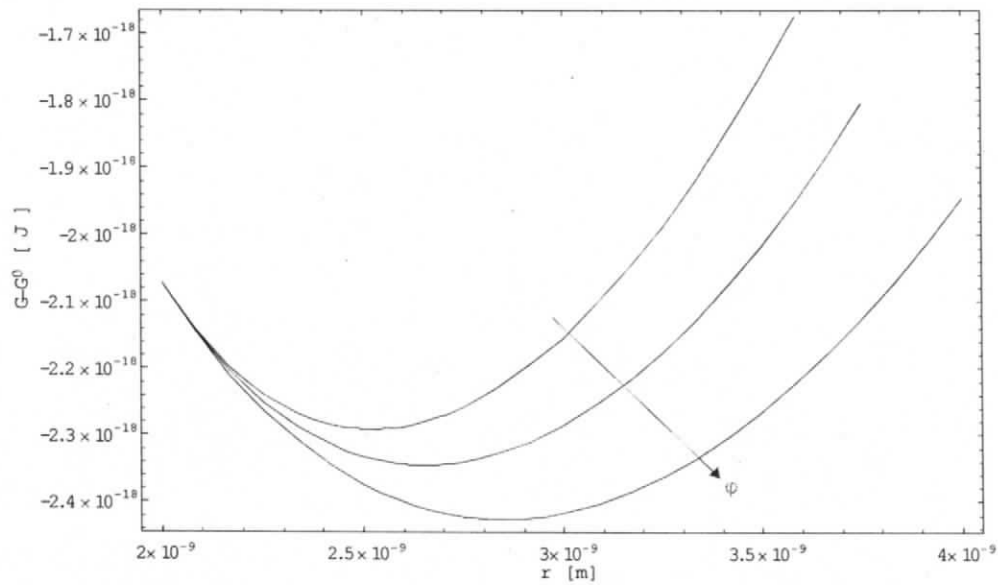
Figure 3.14: Total Free Energy vs r ( \phi = 1/2, 1/3, 1/4 ) - Spherical Pore ( r_0 = 0.5 \text{ nm} ) with a constant liquid-vapor interface.
