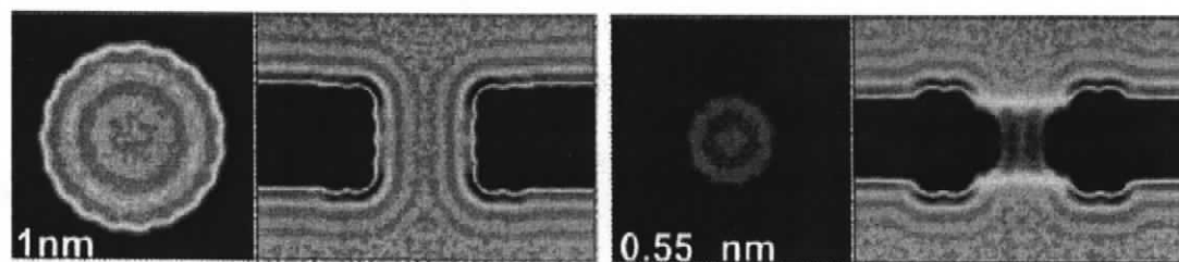
Figure 1.3: Evaporation in Nanopores [12].
