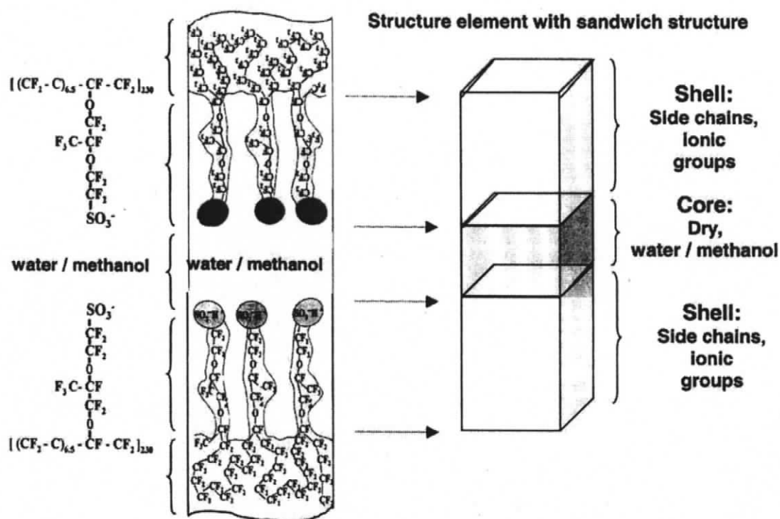
Figure 1.7: Sandwich Structure [28].
