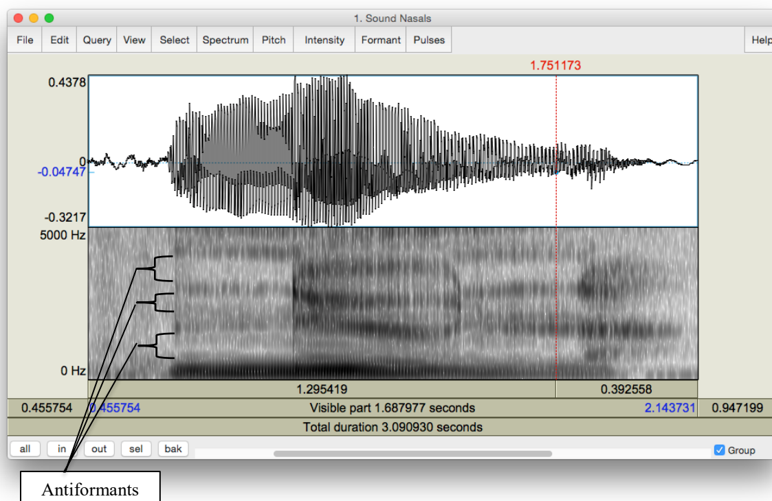
Figure 7.2 Antiformants
