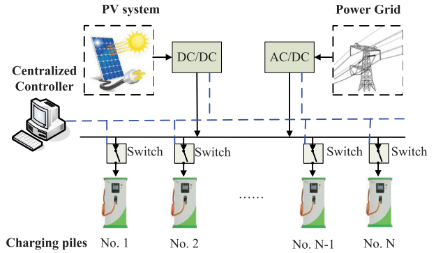
FIGURE 1. The operation model of the designed system.
